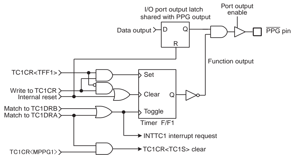
Figure 8-7 PPG Output
