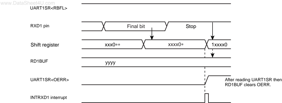
Figure 12-7 Generation of Overrun Error
