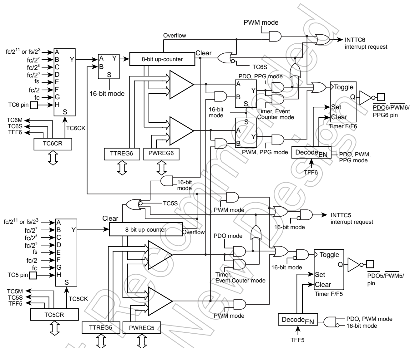
Figure 9-1 8-Bit TimerCounter 5, 6
