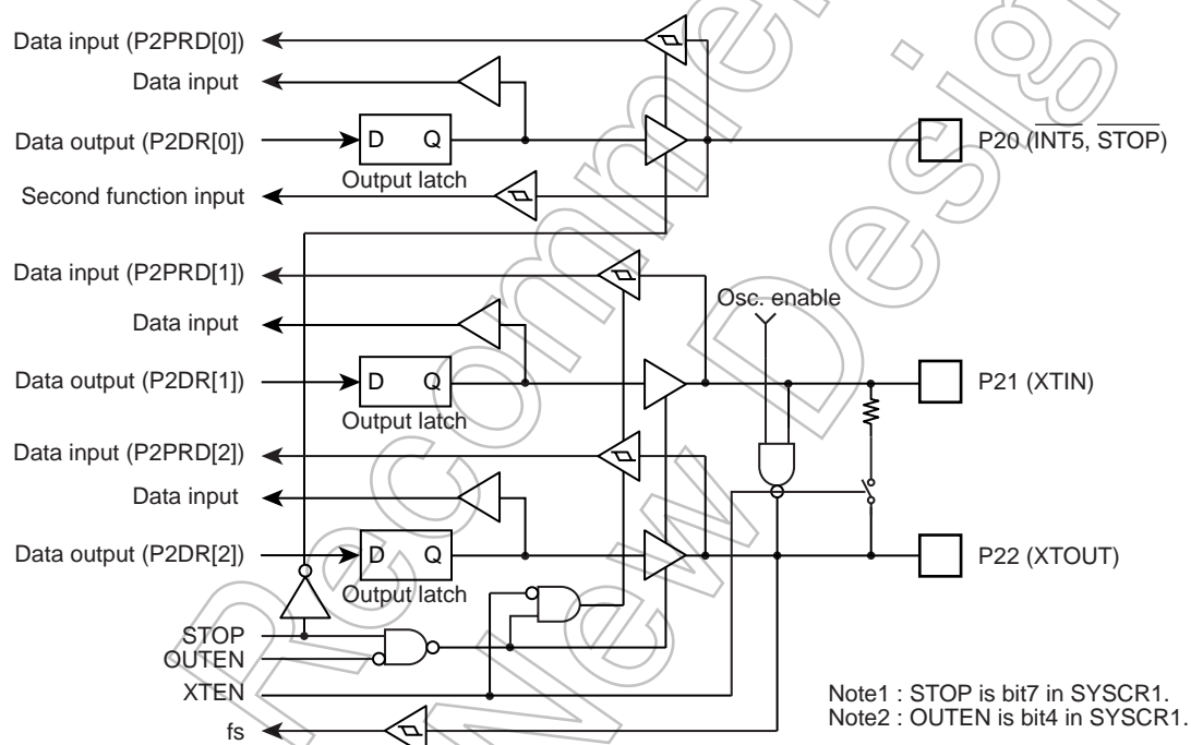
Figure 5-3 Port 2
