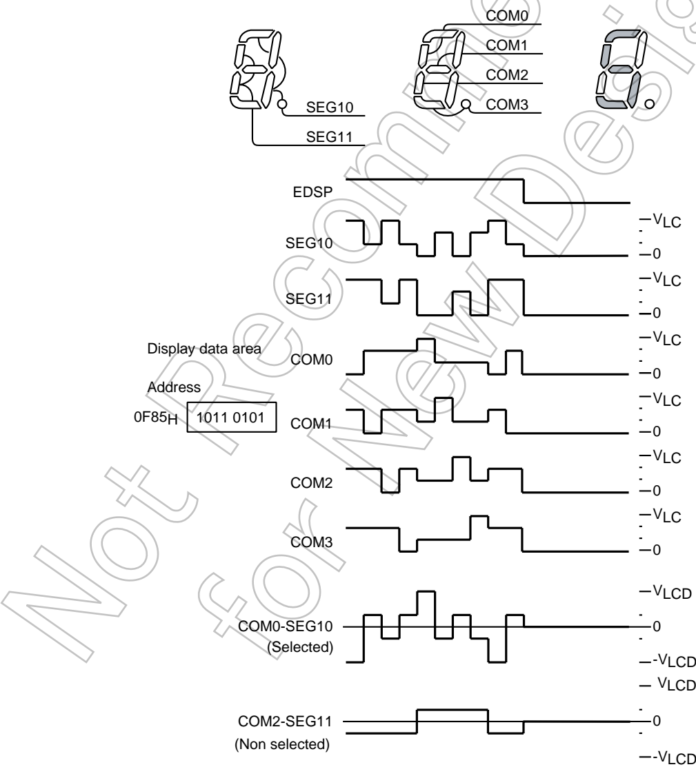
Figure 15-7 1/4 Duty (1/3 Bias) Drive
