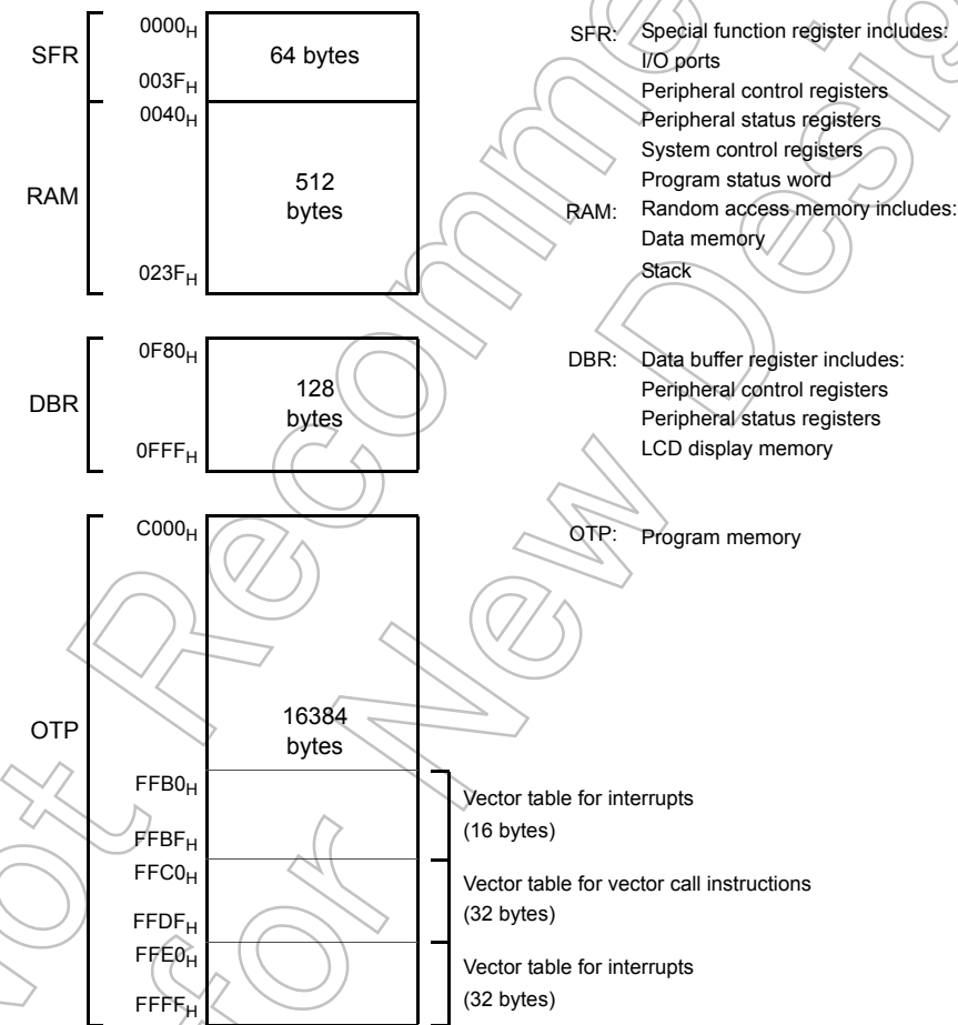
Figure 2-1 Memory Address Map
