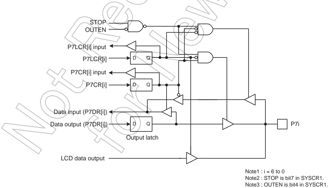
Figure 5-7 Port 7
