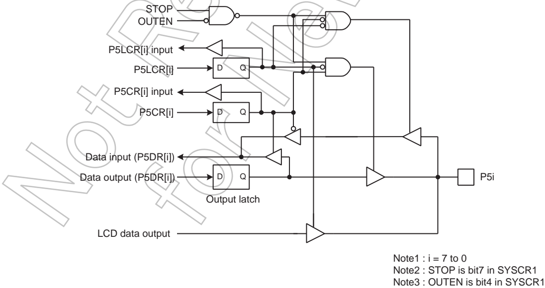
Figure 5-5 Port 5
