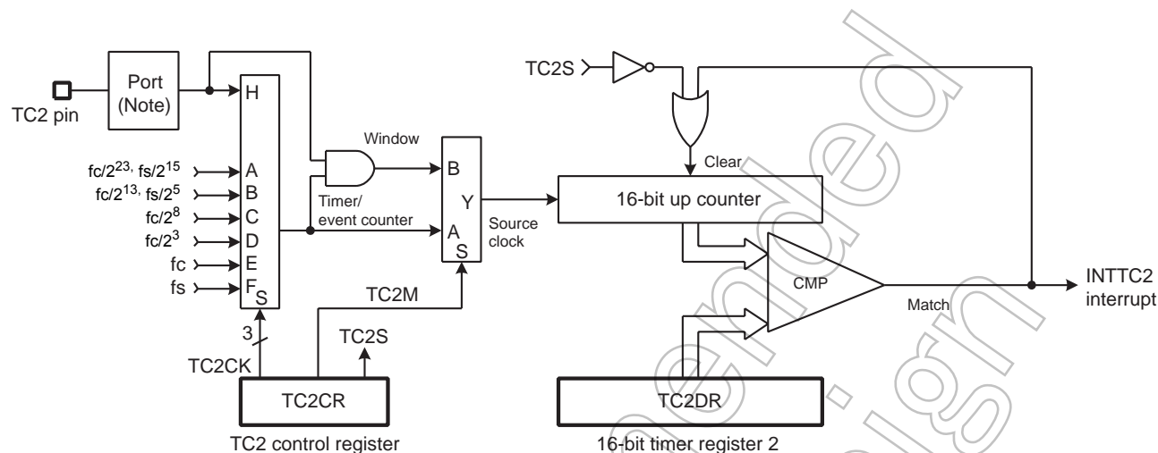
Figure 9-1 Timer/Counter2 (TC2)
