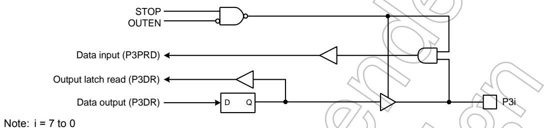
Figure 5-5 Port 3
