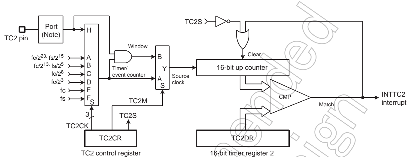
Figure 9-1 Timer/Counter2 (TC2)
