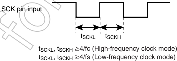
Figure 12-2 External Clock
