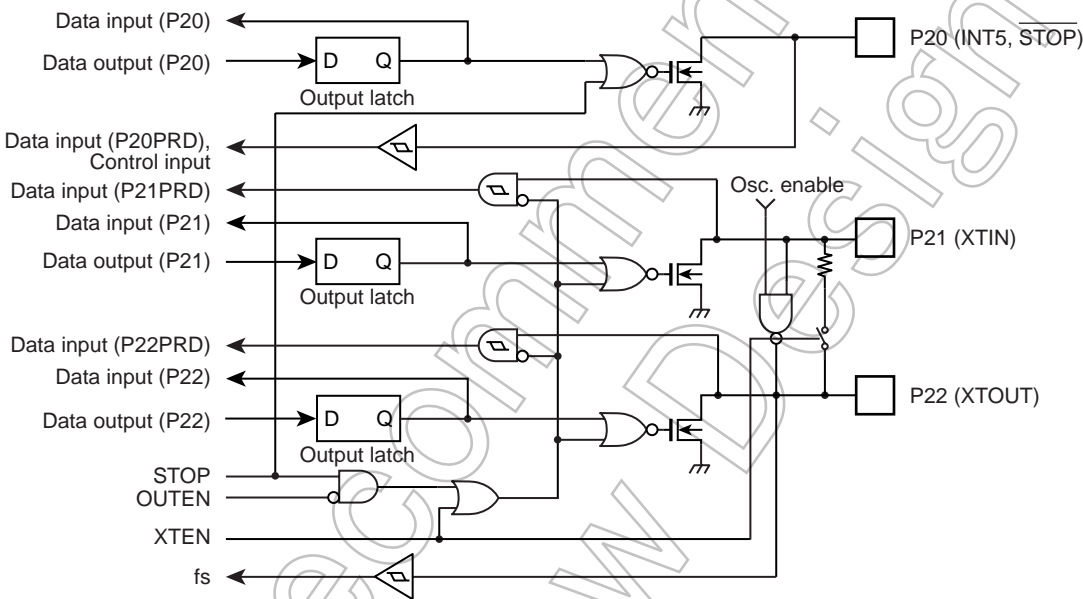
Figure 5-4 Port P2
