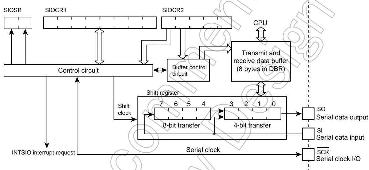
Figure 12-1 Serial Interface
