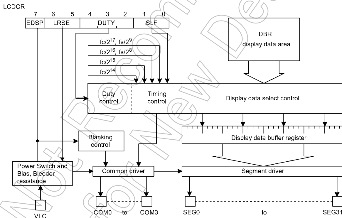
Figure 15-1 LCD Driver
