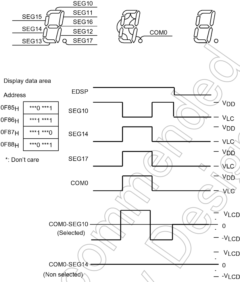
Figure 15-11 Static Drive
