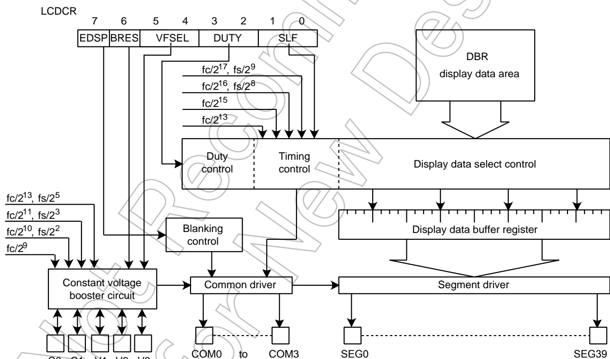
Figure 15-1 LCD Driver
