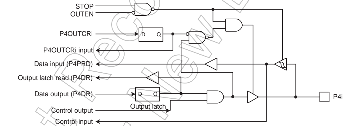
Figure 5-6 Port 4
