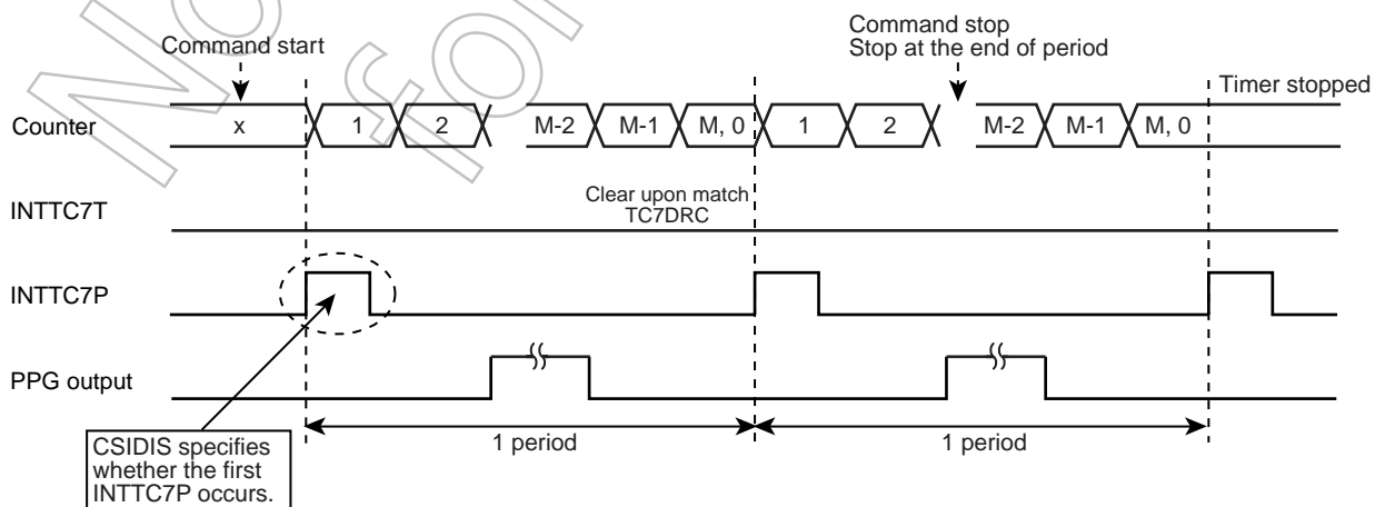
Figure 8-21 Period Interrupt
