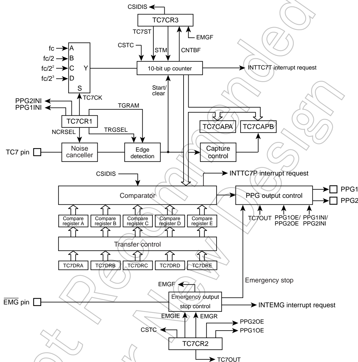
Figure 8-1 10-Bit Timer/Counter 7
