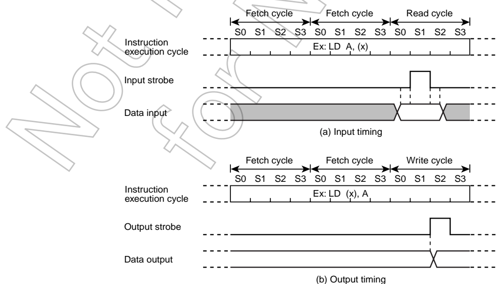
Figure 5-1 Input/Output Timing (Example)
