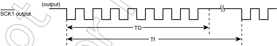
Figure 15-2 Frame time ( T_f ) and Data transfer time ( T_D )
