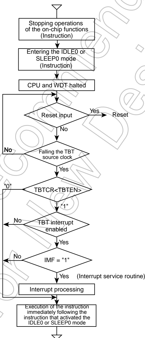
Figure 2-12 IDLE0 or SLEEP0 Mode
