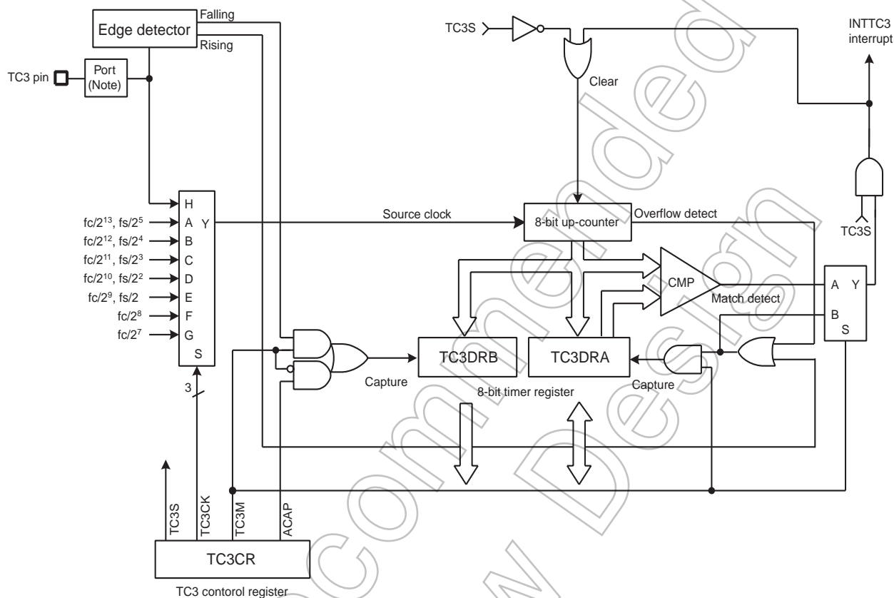
Figure 10-1 TimerCounter 3 (TC3)
