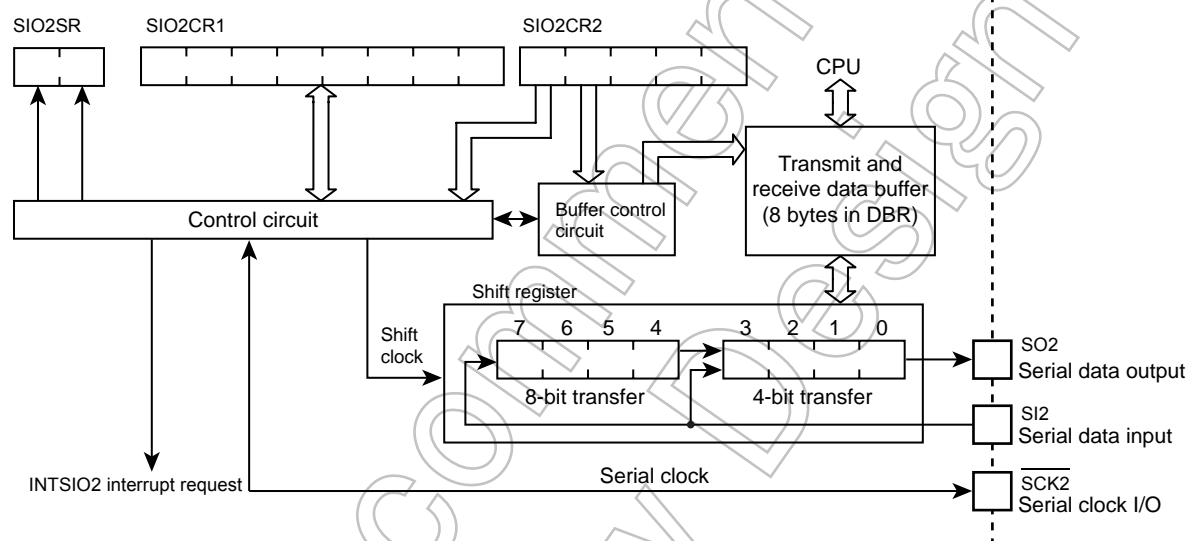
Figure 16-1 Serial Interface
