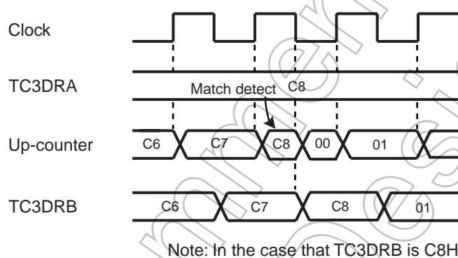
Figure 10-2 Auto-Capture Function
