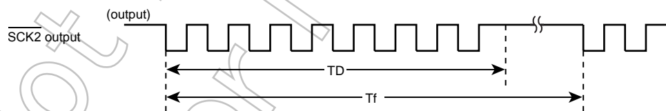
Figure 16-2 Frame time ( T_f ) and Data transfer time ( T_D )
