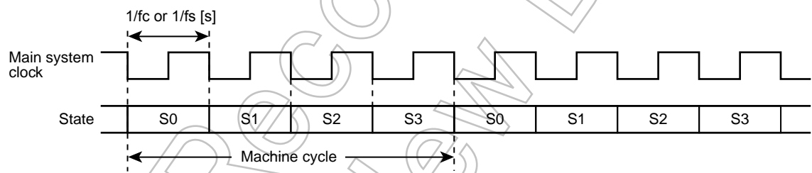
Figure 2-5 Machine Cycle
