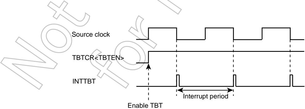
Figure 7-2 Time Base Timer Interrupt
