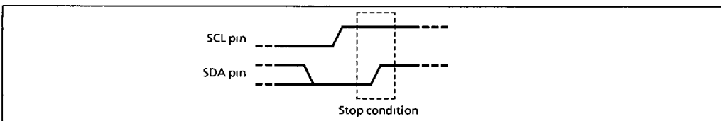
Figure 2-33. Stop Condition Generation
