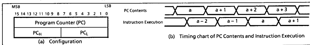
Figure 1-3. Program Counter
