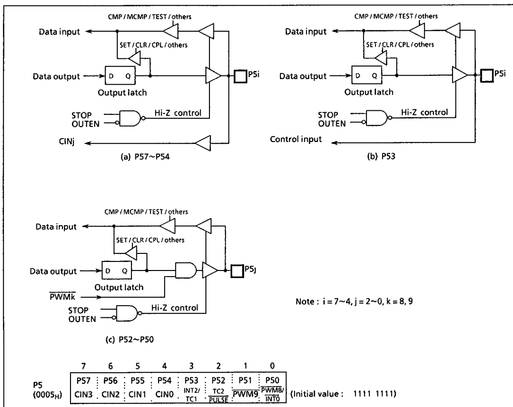
Figure 2-6. Ports P5
