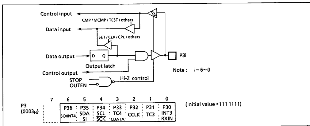
Figure 2-4 Port P3
