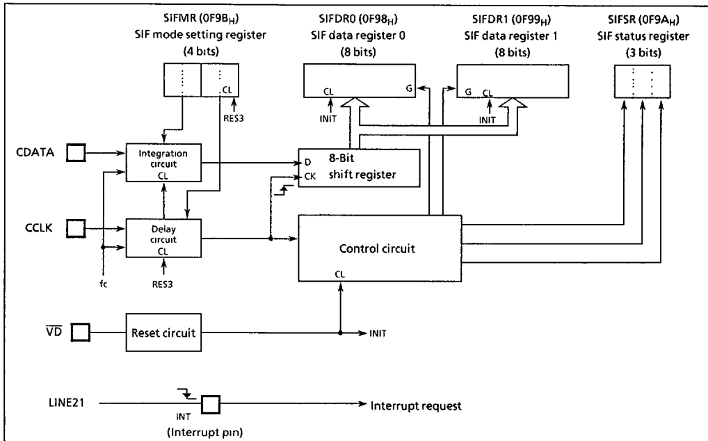
Figure 2-78. Slicer interface
