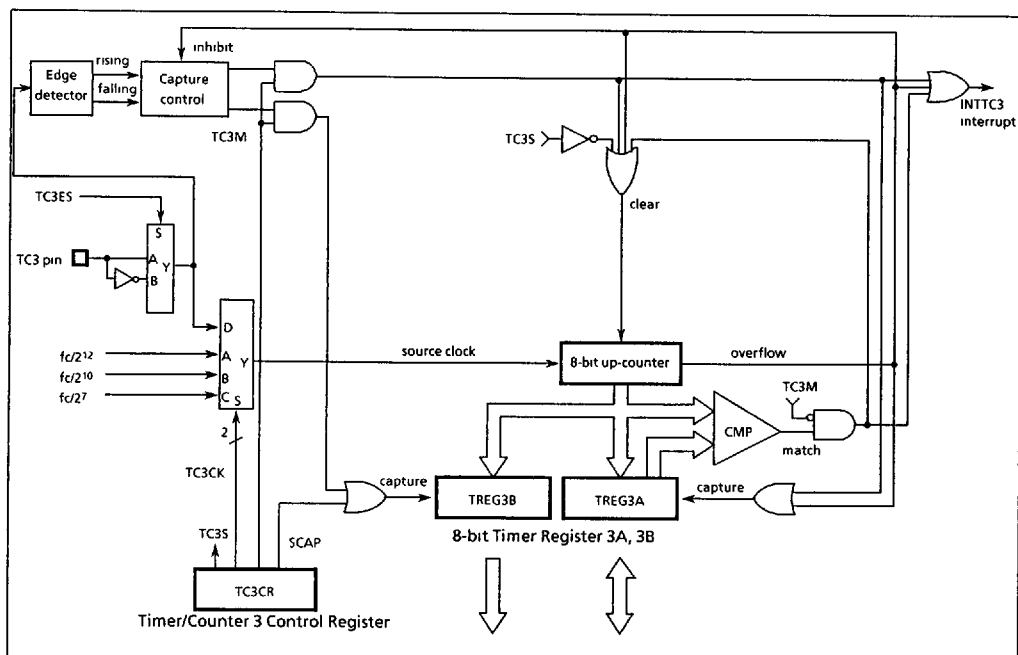
Figure 2-21. Timer/Counter 3
