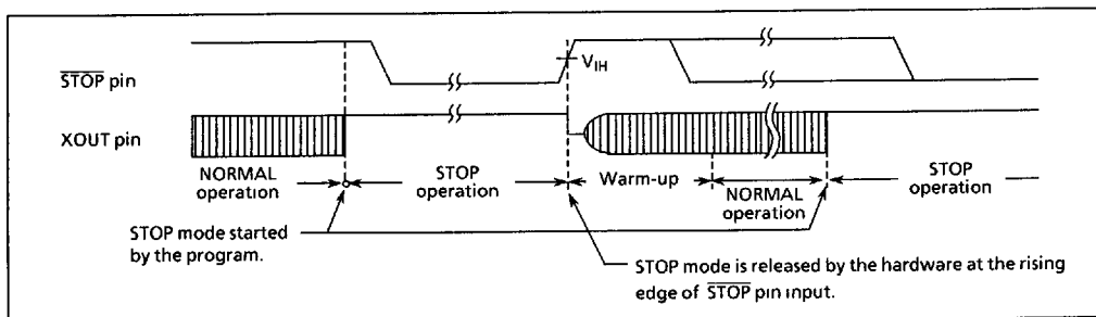
Figure 1-16. Edge-sensitive Release Mode
