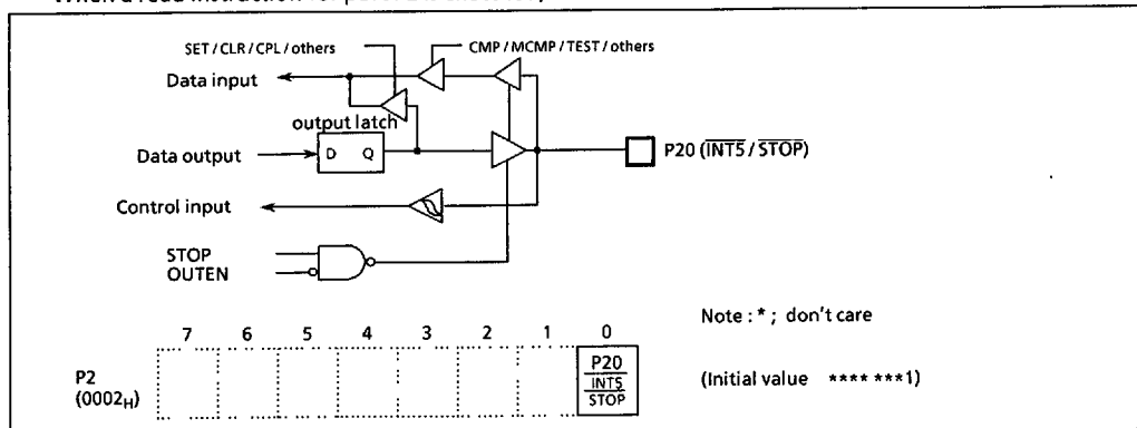
Figure 2-3 Port P2
