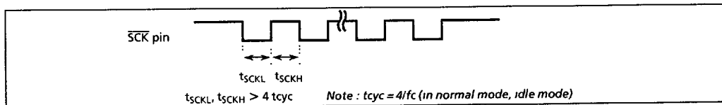
Figure 2-42. External Clock
