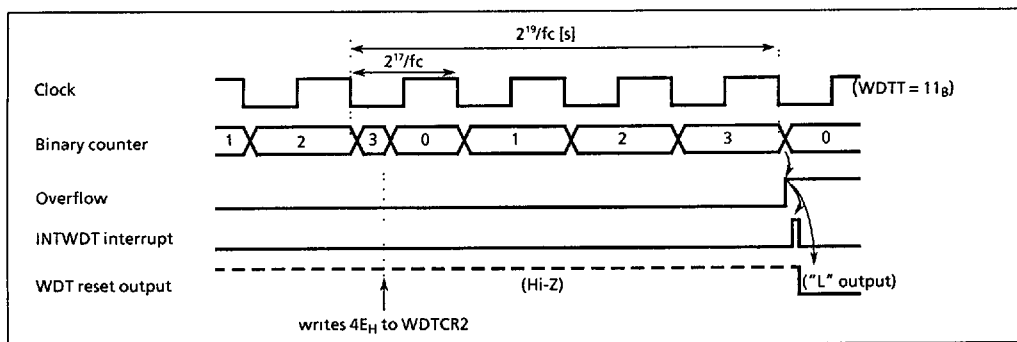
Figure 1-27. Watchdog Timer Interrupt / Reset
