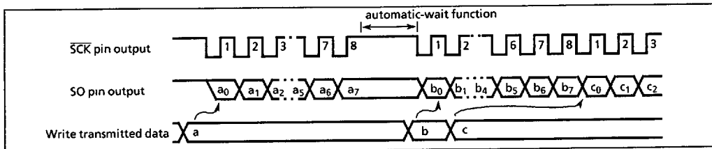
Figure 2-41. Automatic-wait Function
