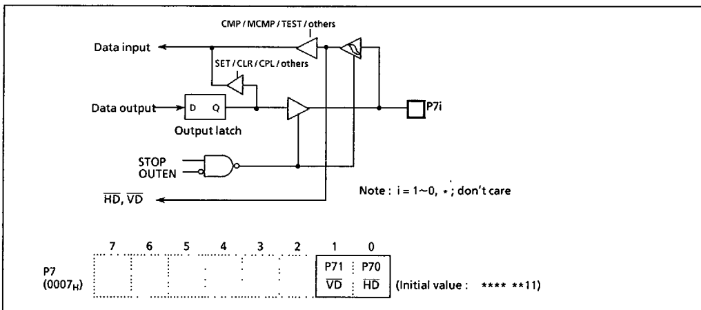
Figure 2-8. Ports P7
