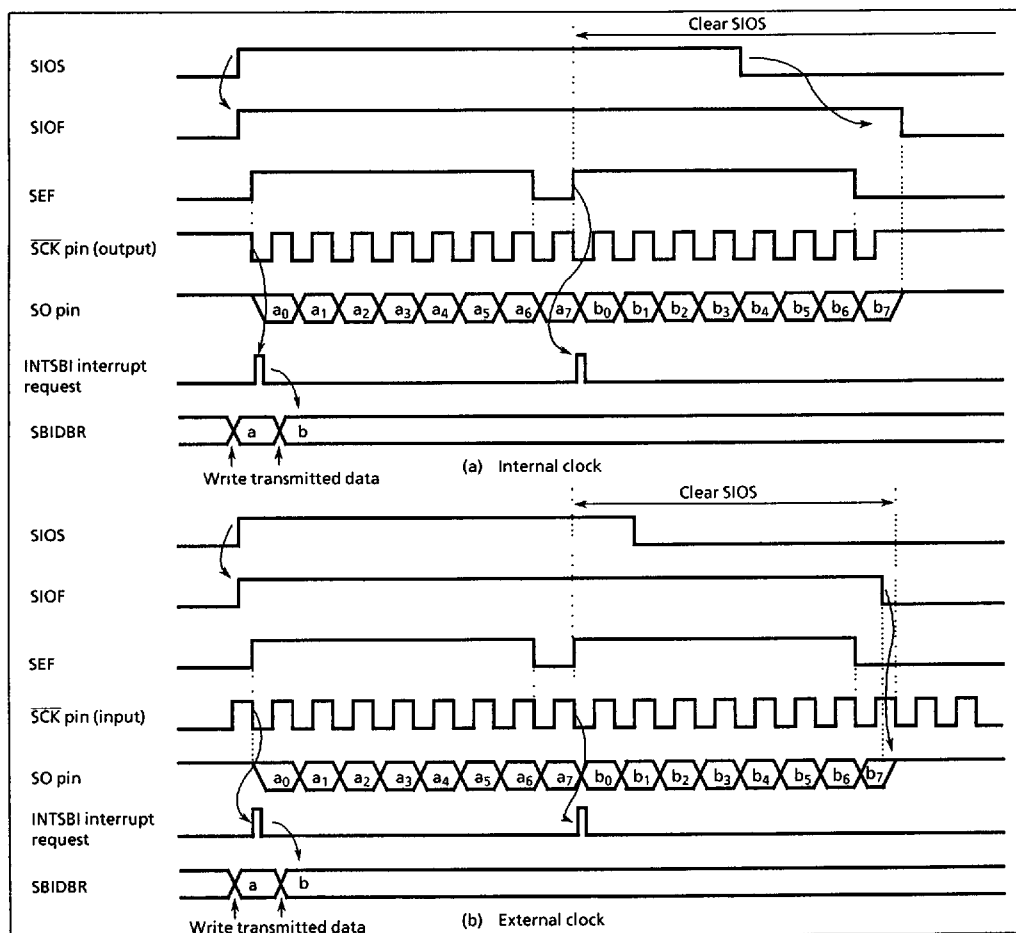
Figure 2-44. Transfer Mode
