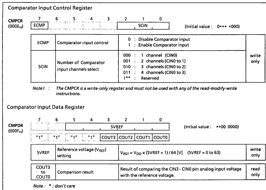
Figure 2-58. Comparator Input Control Register and Data Register
