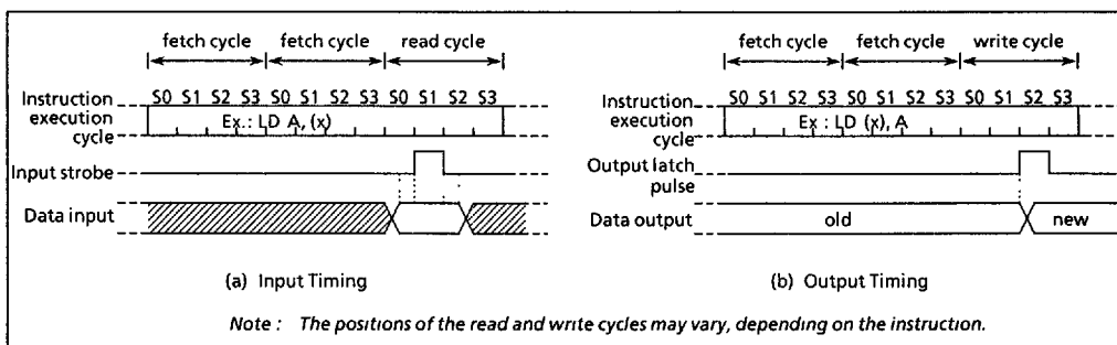
Figure 2-2. Input/Output Timing (Example)
