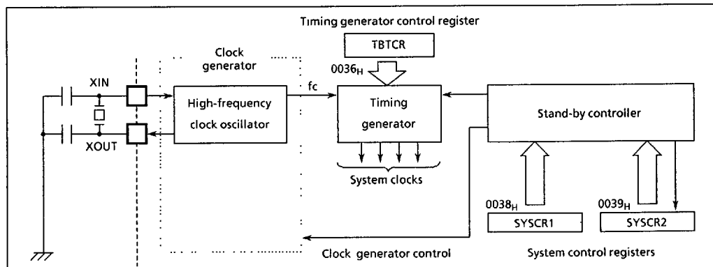
Figure 1-9. System Clock Controller
