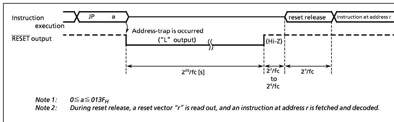
Figure 1-27. Address-Trap-Reset
