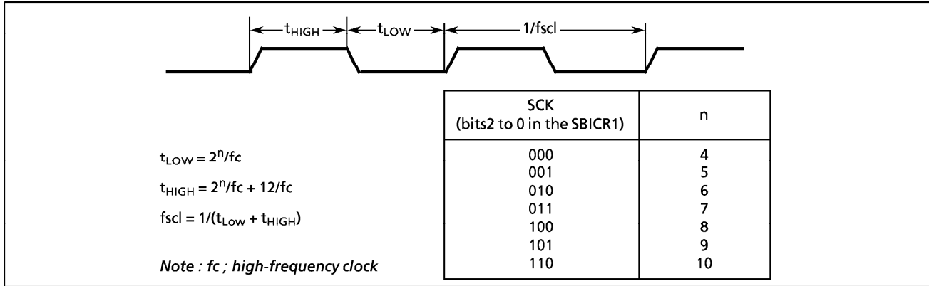
Figure 2-28. Clock Source
