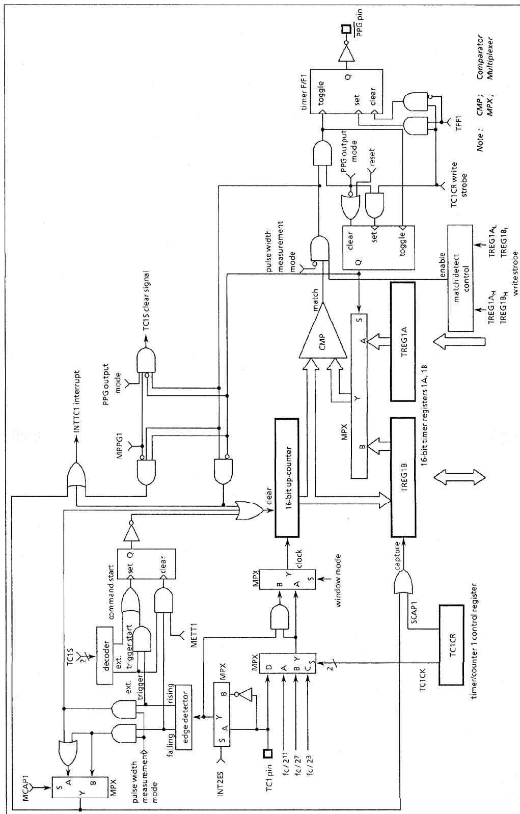
Figure 2-12. Timer/Counter 1
