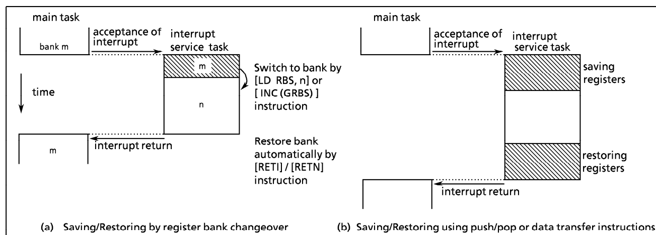
Figure 1-21. Saving/Restoring General-purpose Registers
