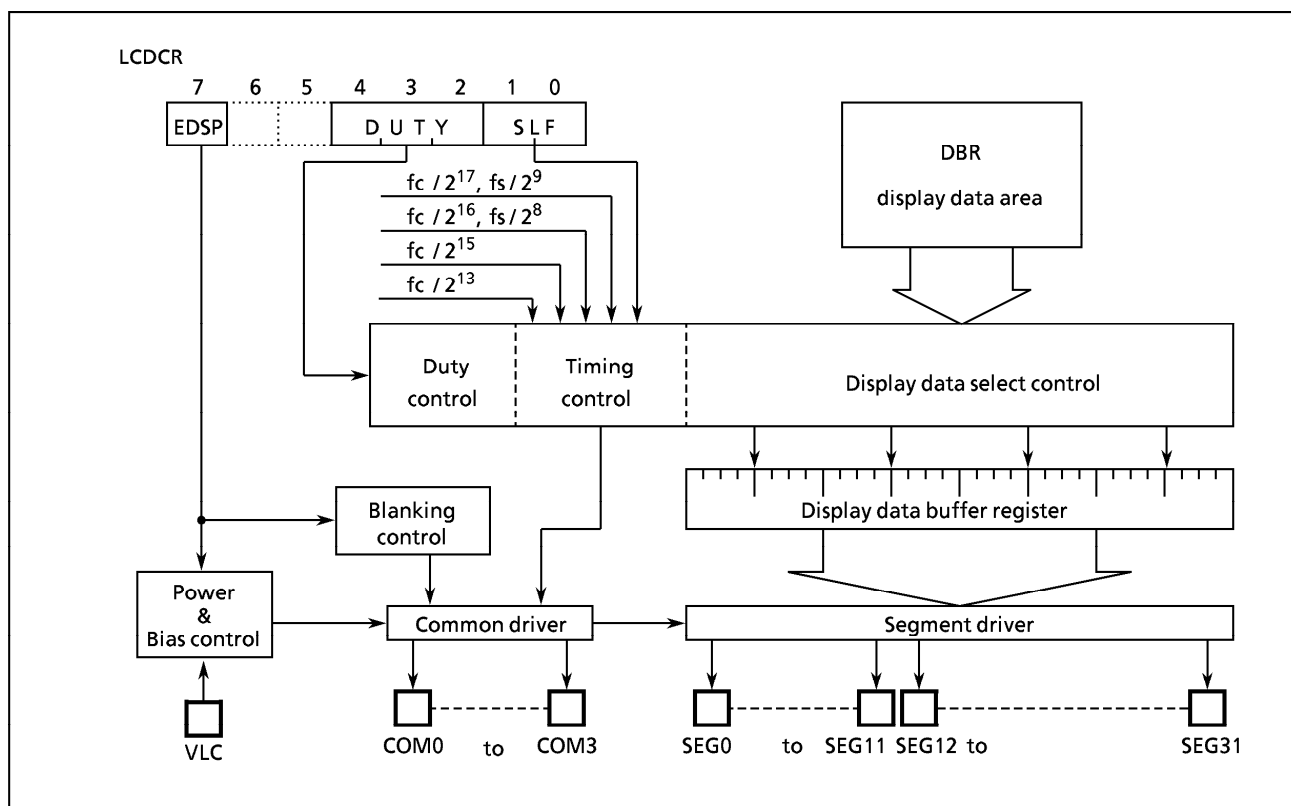
Figure 2-42. LCD driver
