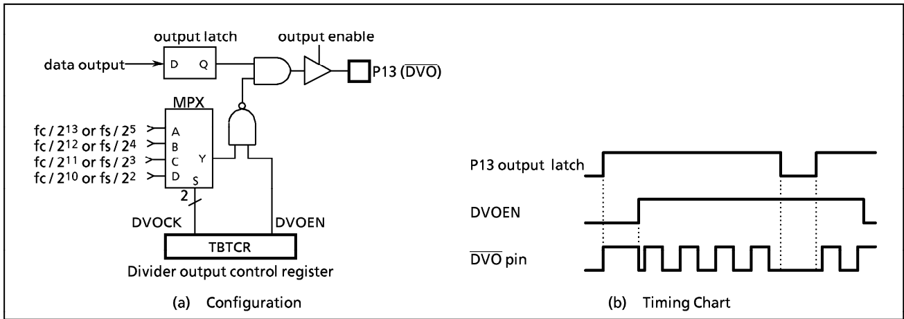
Figure 2-12. Divider Output
