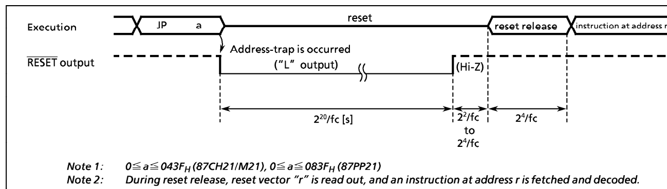
Figure 1-31. Address-Trap-Reset
