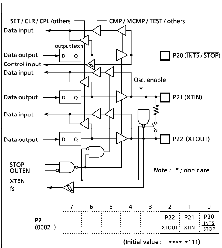
Figure 2-4. Port P2
