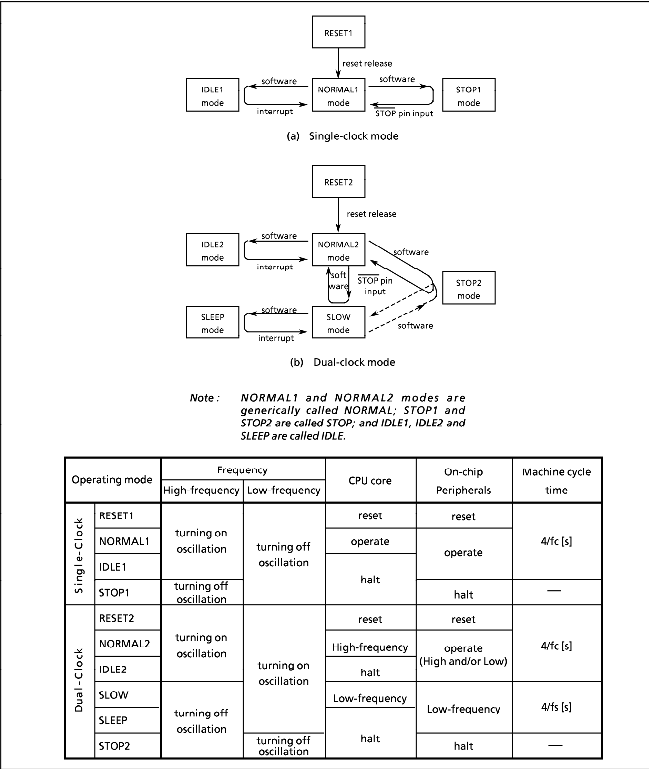
Figure 1-14. Operating Mode Transition Diagram
