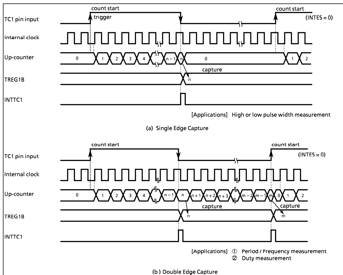
Figure 2-19. Pulse Width Measurement Mode Timing Chart
