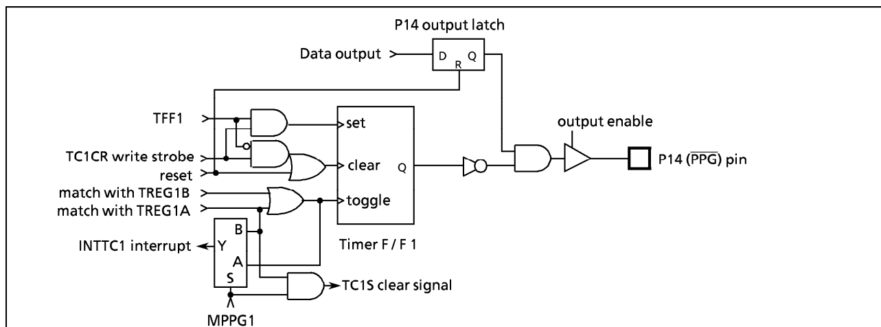
Figure 2-20. \overline{\text{PPG}} Output
