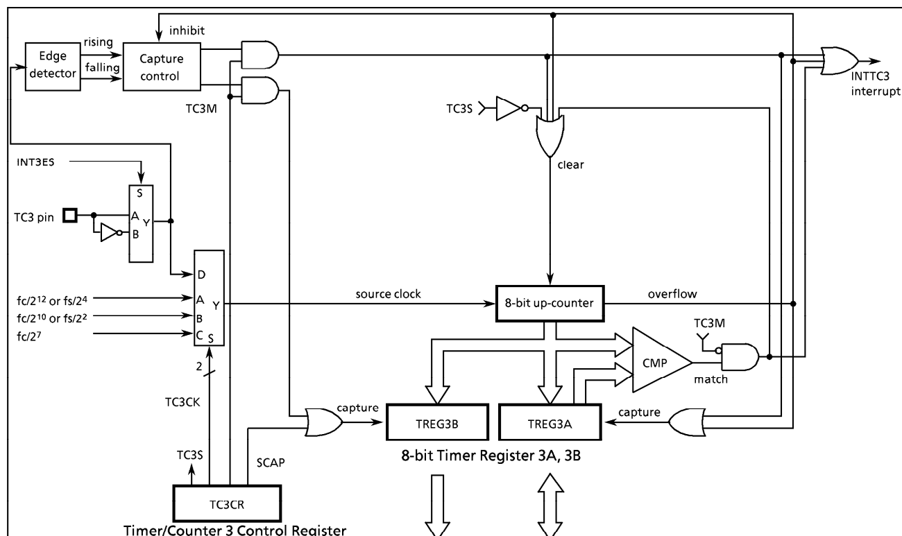
Figure 2-25. Timer/Counter 3
