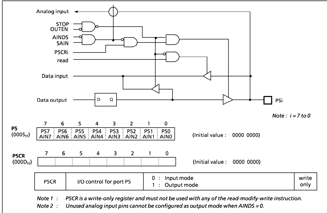
Figure 2-7. Port P5
