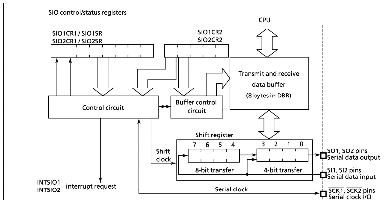
Figure 2-32. Serial Interfaces
