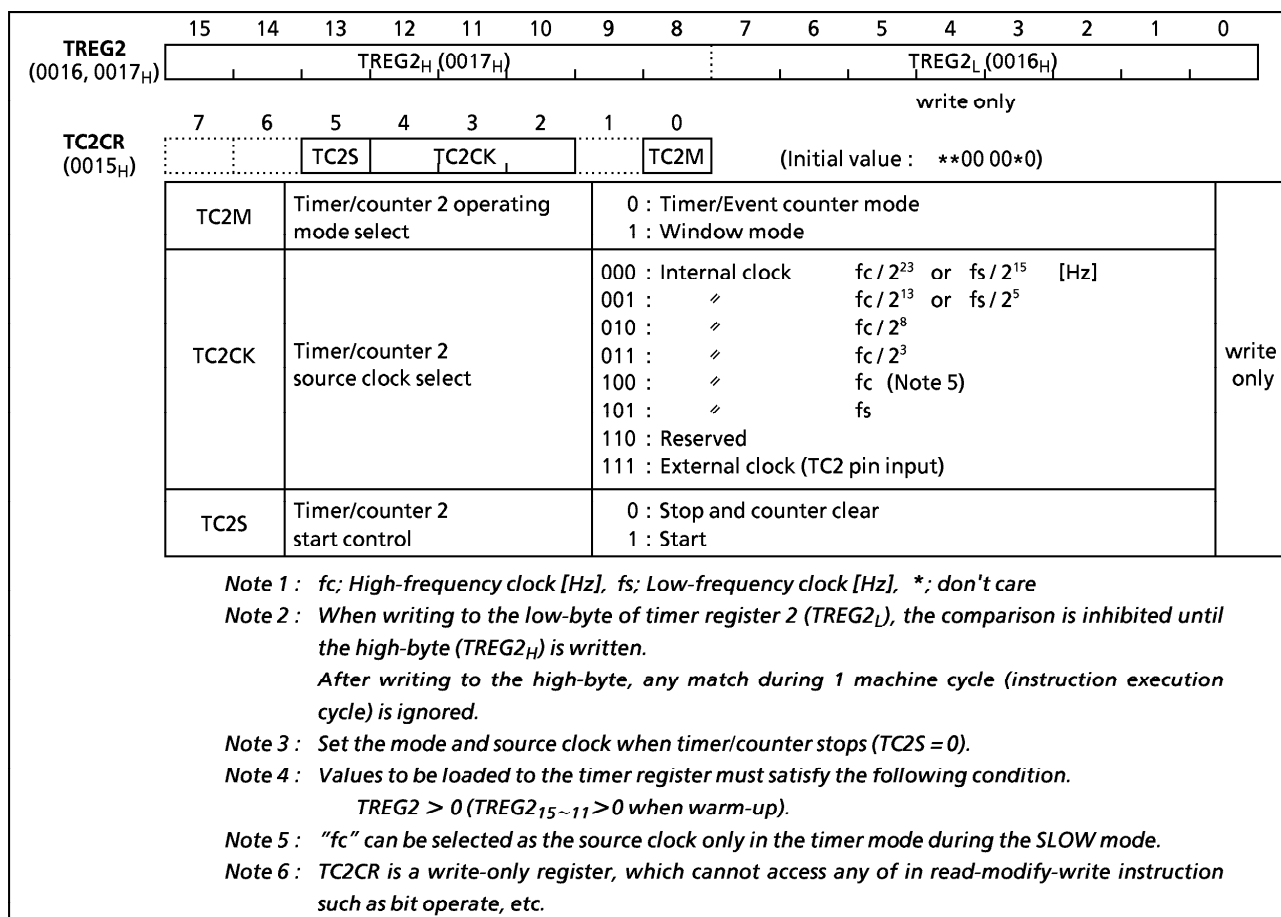
Figure 2-23. Timer Register 2 and TC2 Control Register
