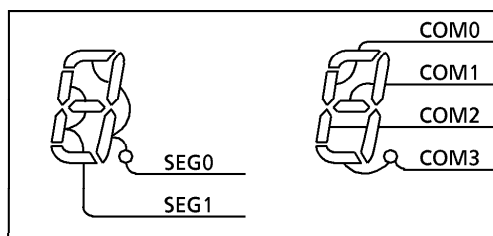
Figure 2-47. Example of COM, SEG Pin Connection (1/4 Duty)
