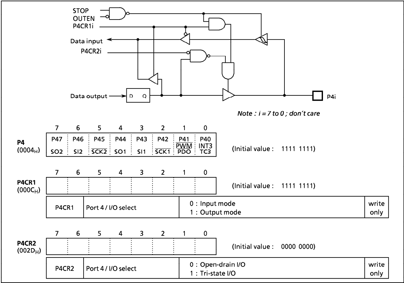
Figure 2-6. Port P4
