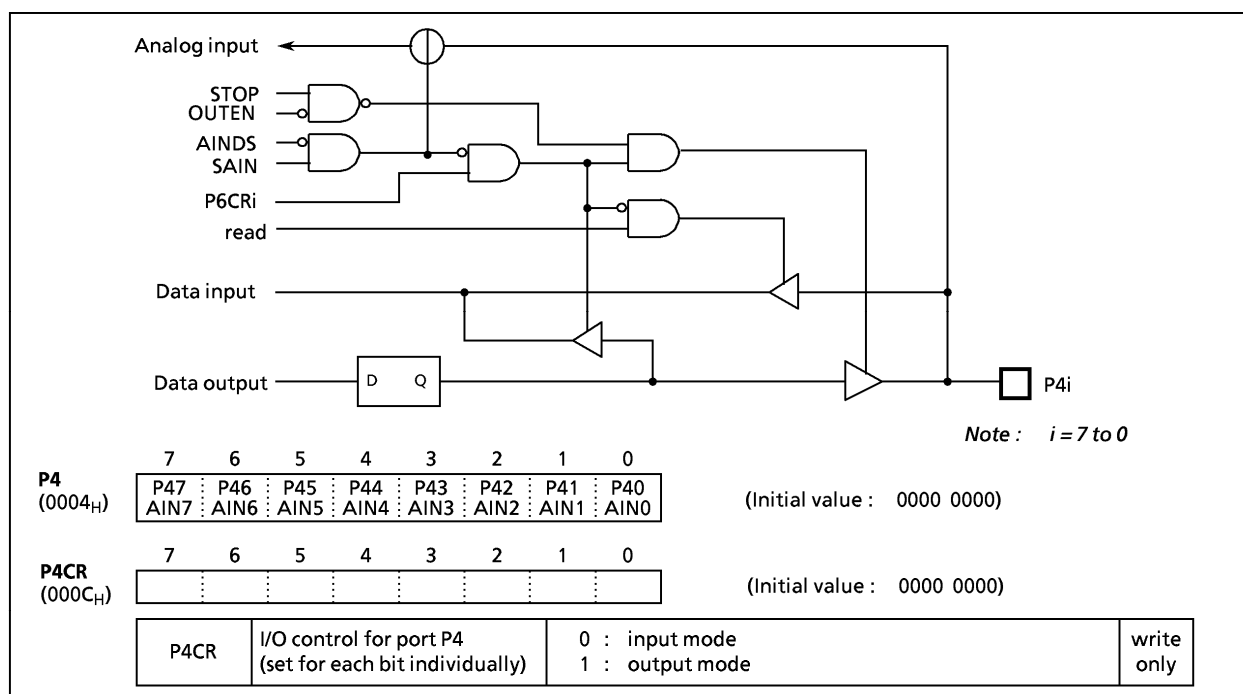
Figure 2-7. Port P4
