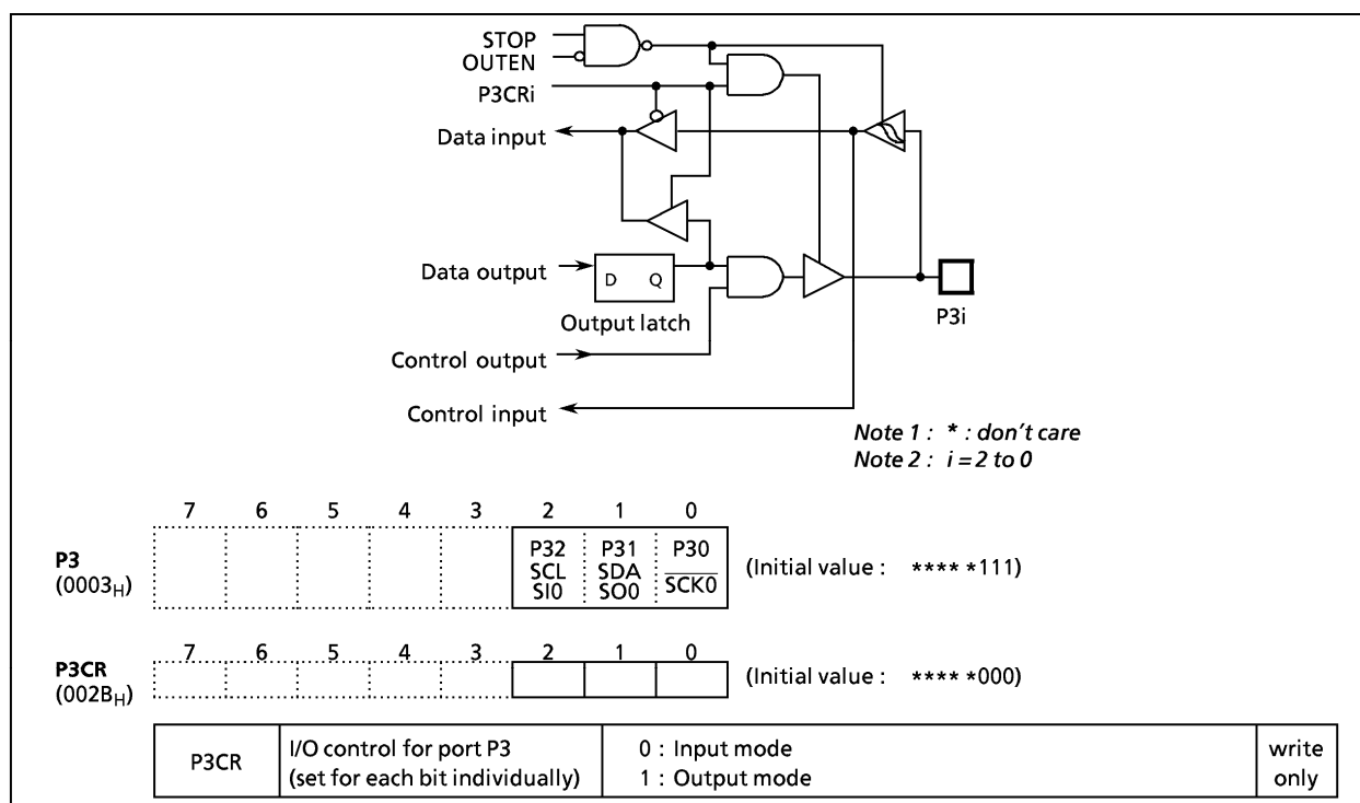
Figure 2-6. Port P3
