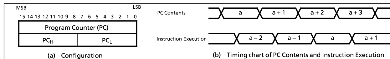
Figure 1-3. Program Counter
