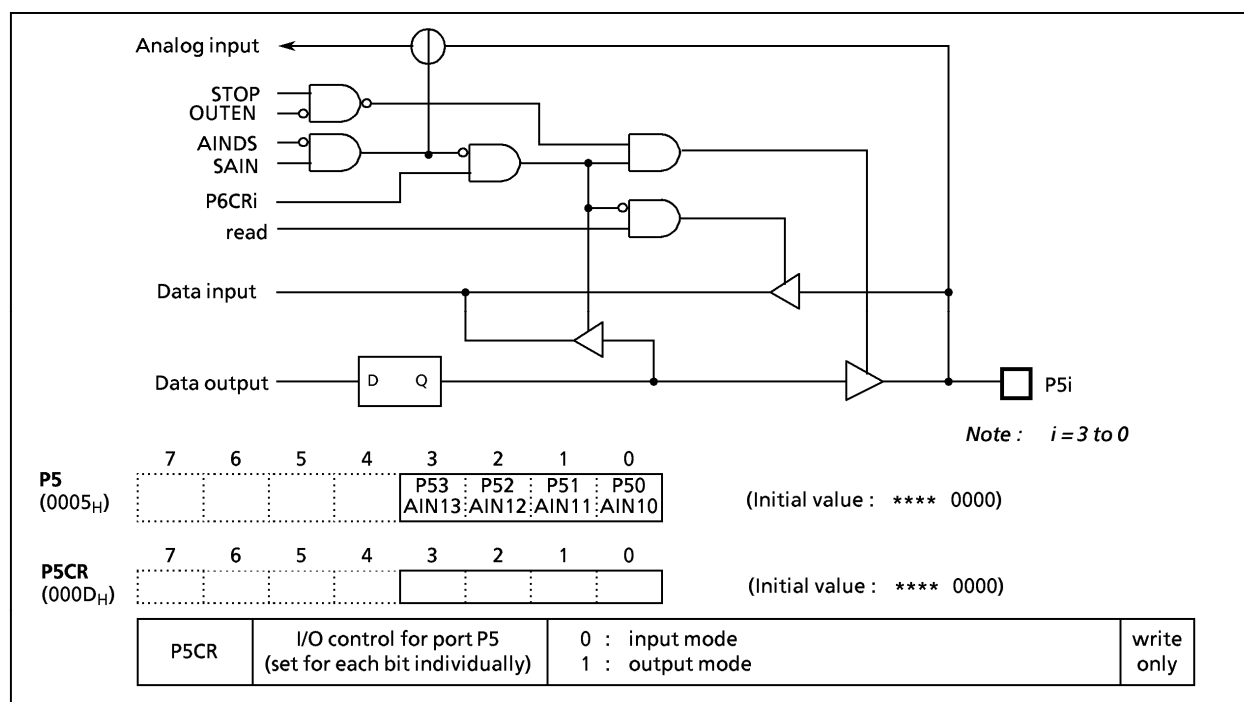
Figure 2-8. Port P5
