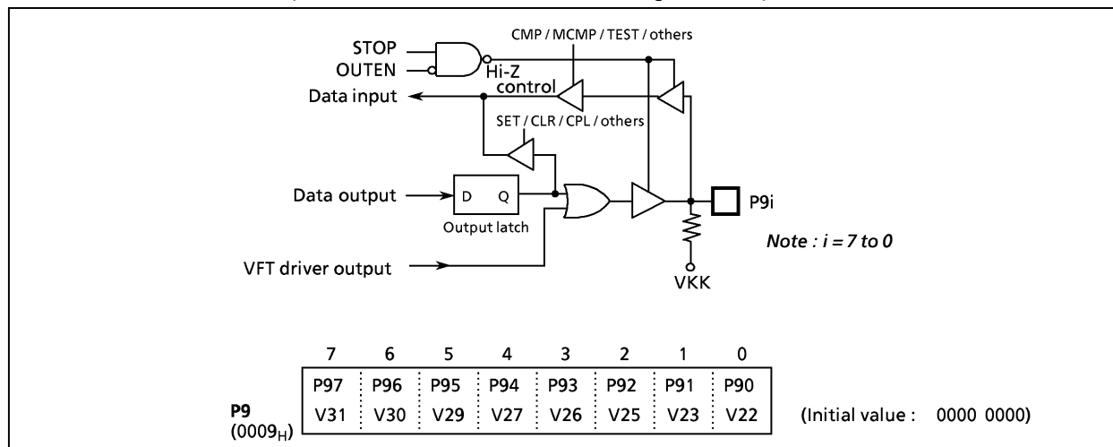
Figure 2-12. Port P9
