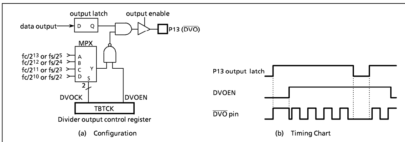
Figure 2-15. Divider Output
