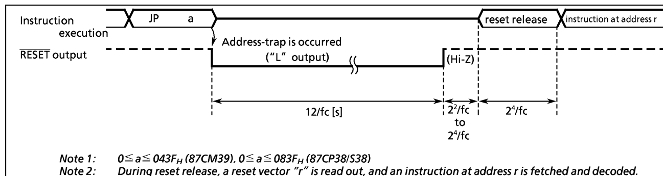
Figure 1-32. Address-Trap-Reset
