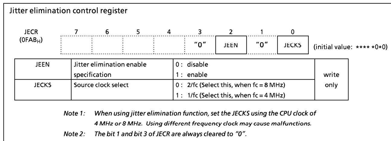
Figure 2-87. Jitter Elimination Control Register
