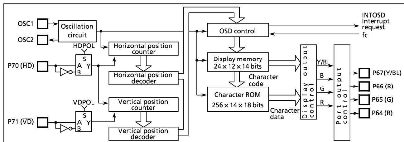
Figure 2-79. OSD Circuit
