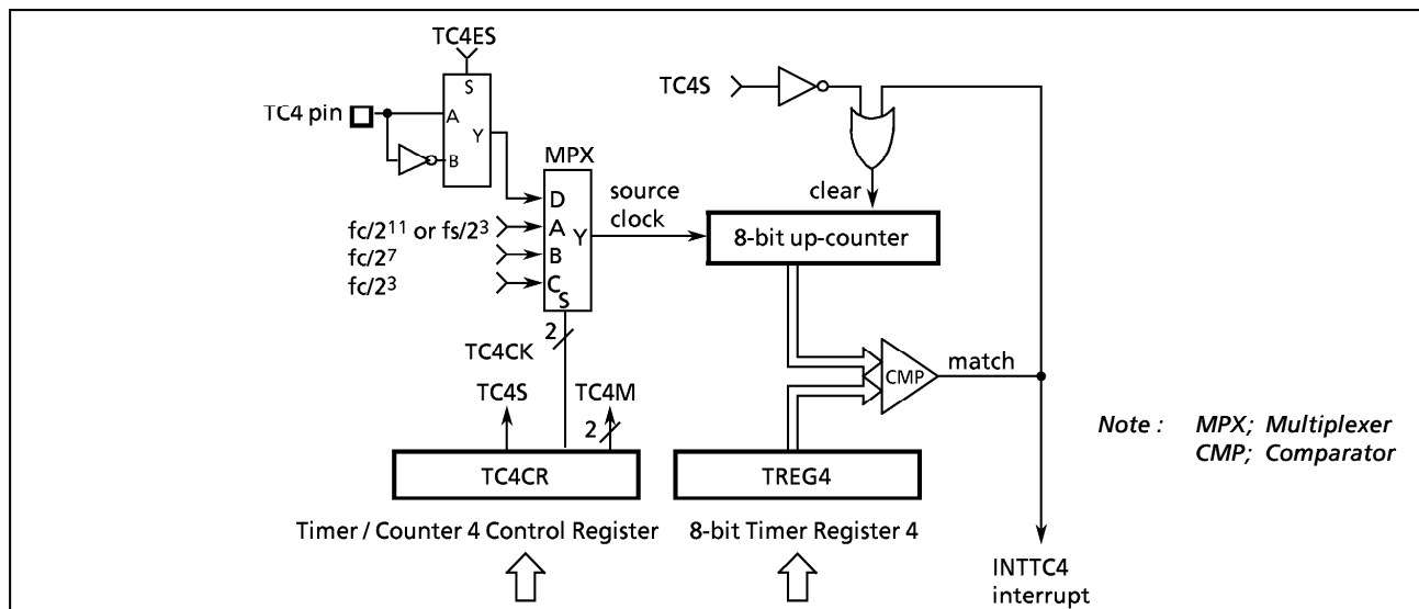
Figure 2-31. Timer / Counter 4
