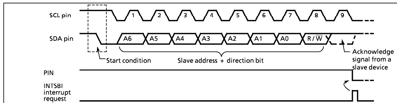
Figure 2-43. Start Condition Generation and Slave Address Transfer
