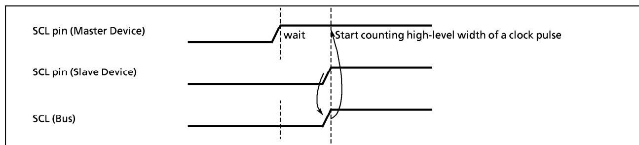
Figure 2-38. Clock Synchronization
