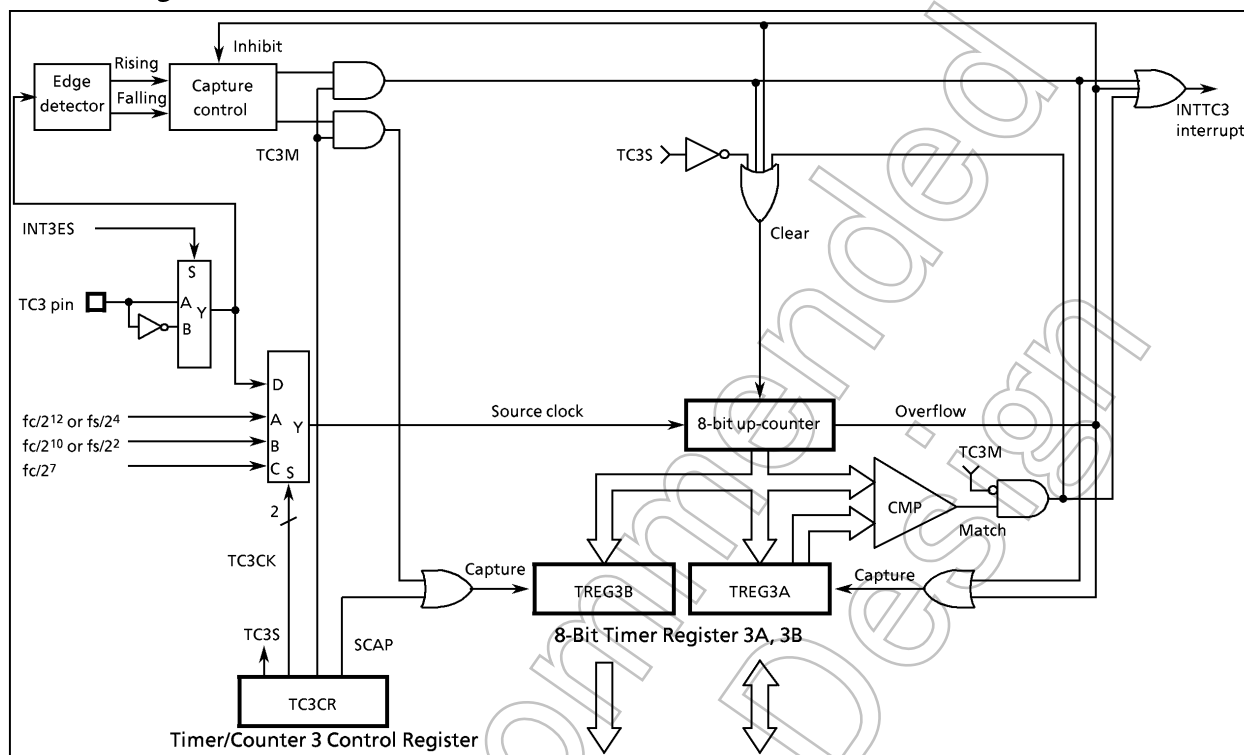
Figure 2-22. Timer/Counter 3
