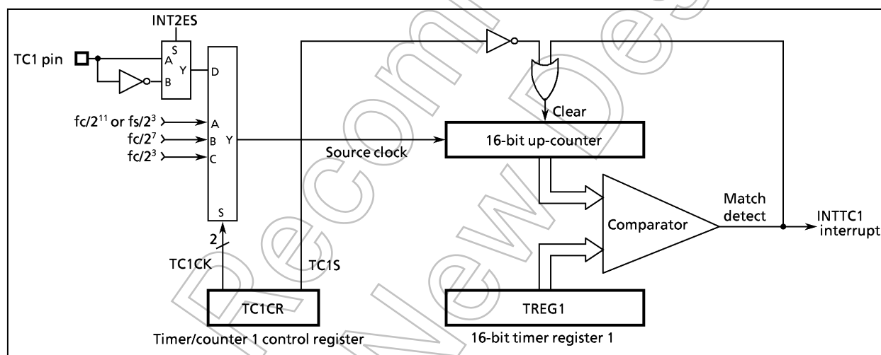
Figure 2-16. Timer/Couter 1
