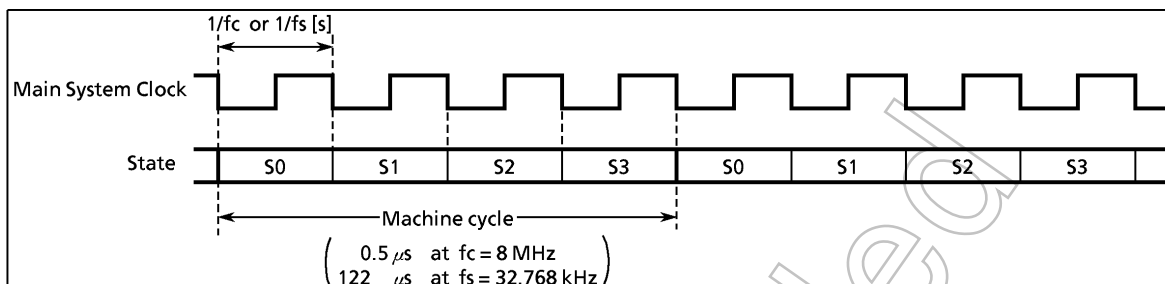
Figure 1-13. Machine Cycle
