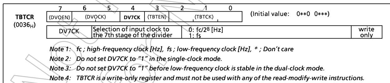
Figure 1-12. Timing Generator Control Register
