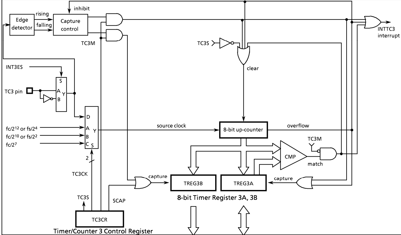
Figure 2-22. Timer/Counter 3
