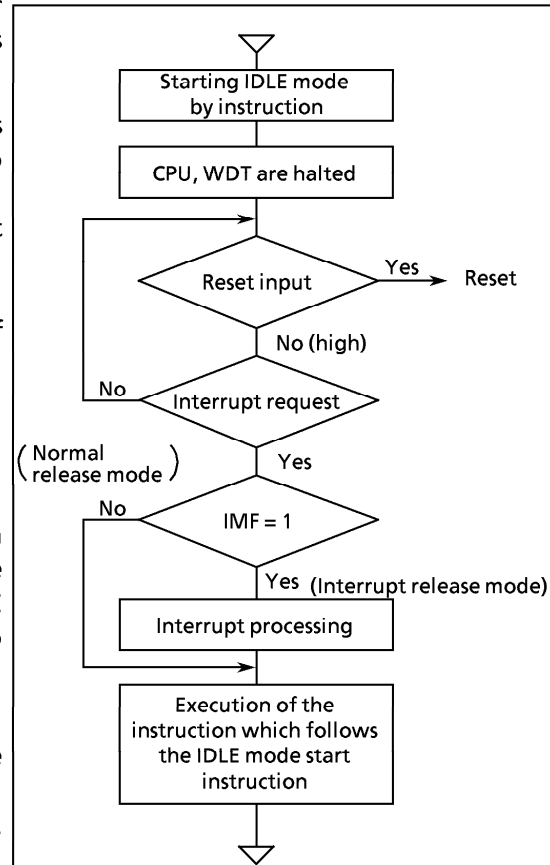
Figure 1-19. IDLE Mode
