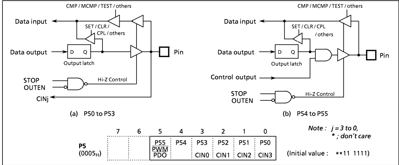
Figure 2-8. P5 Port
