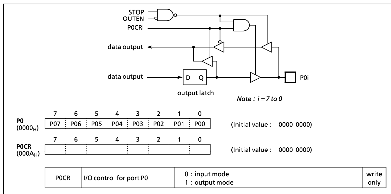
Figure 2-3. Port P0 and P0CR
