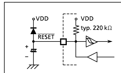
Figure 1-30. Simple Power-on-Reset Circuitry
