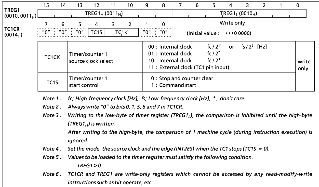
Figure 2-17. Timer Register 1 and TC1 Control Register
