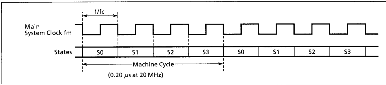
Figure 1-7. Machine Cycles
