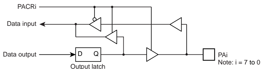
Figure 5-12 Port PA
