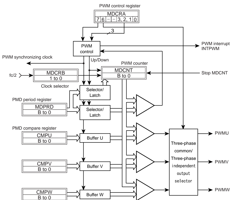
Figure 13-10 Pulse Width Modulation Circuit
