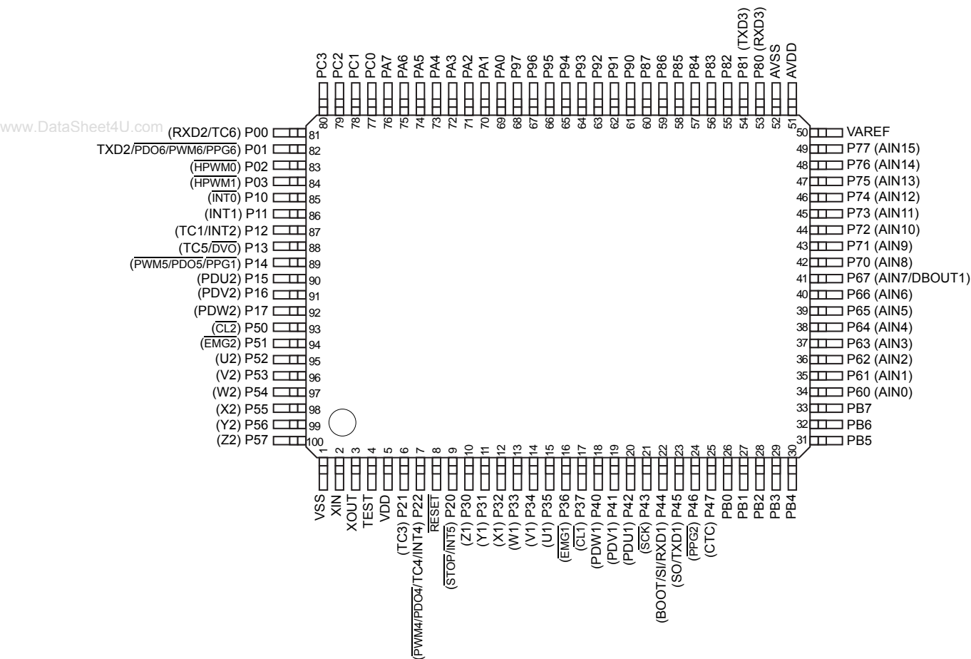
Figure 1-1 Pin Assignment
