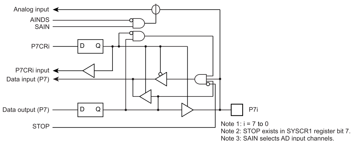
Figure 5-9 Port P7
