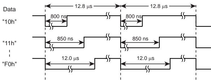
Figure 18-2 8-Bit Mode
