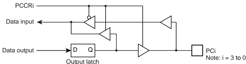
Figure 5-14 Port PC
