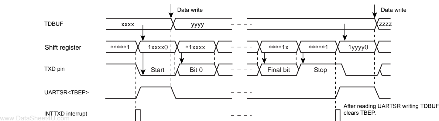
Figure 14-9 Generation of Transmit Data Buffer Empty
