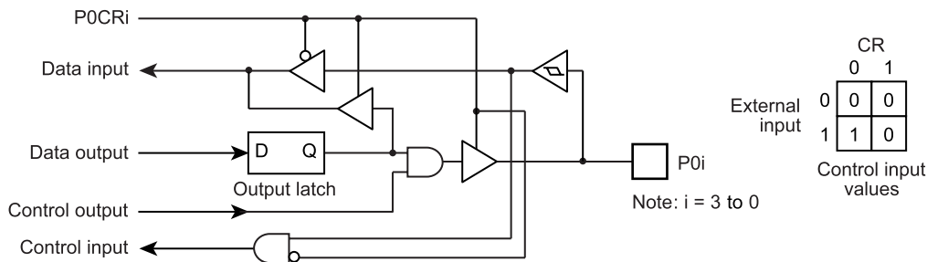
Figure 5-2 Port P0
