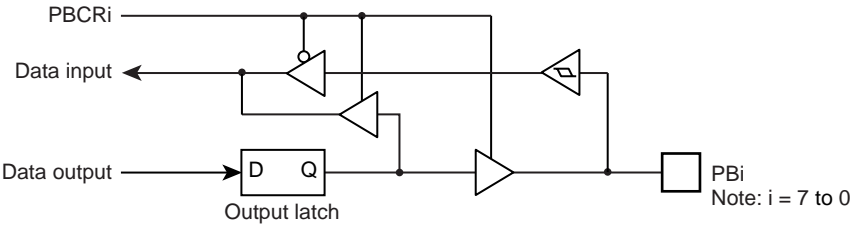
Figure 5-13 Port PB
