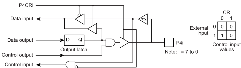
Figure 5-6 Port P4
