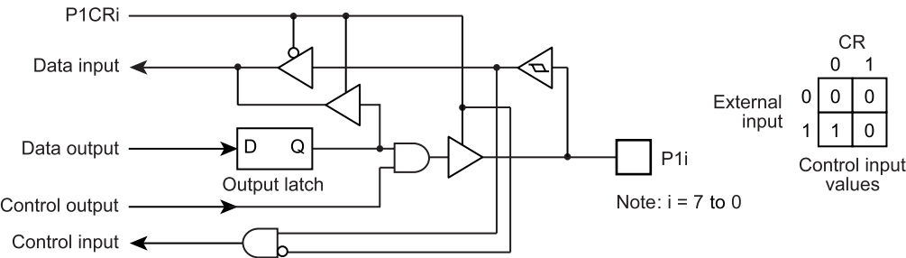
Figure 5-3 Port P1
