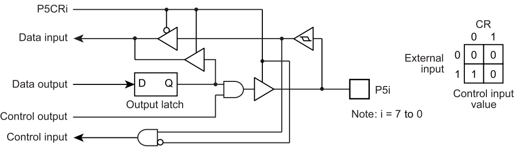
Figure 5-7 Port P5
