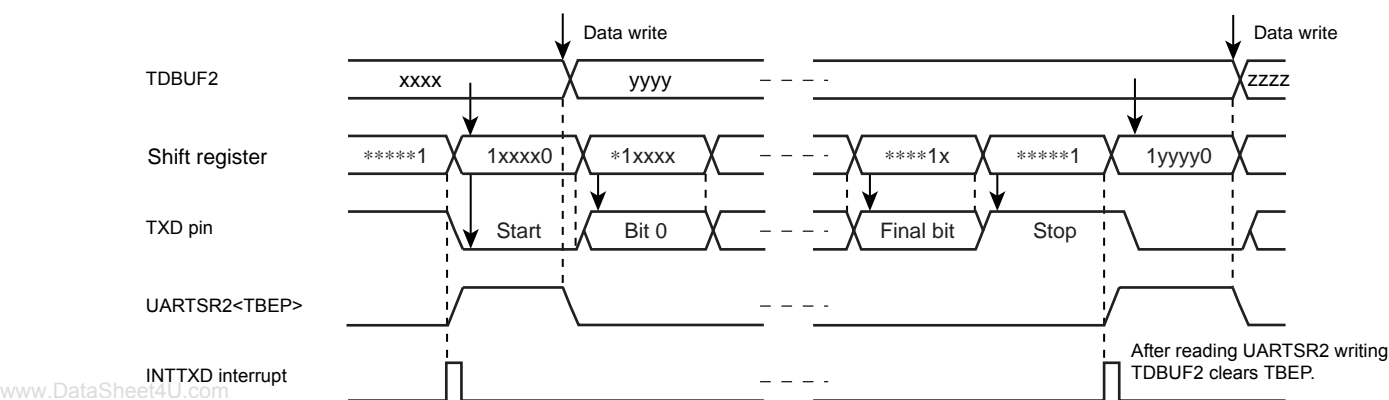
Figure 15-9 Generation of Transmit Data Buffer Empty
