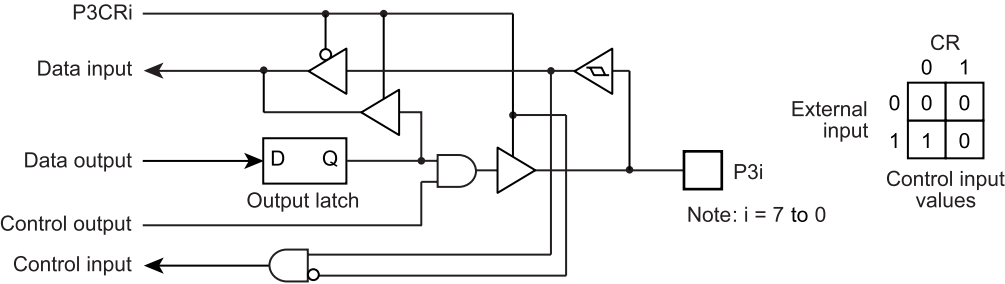
Figure 5-5 Port P3
