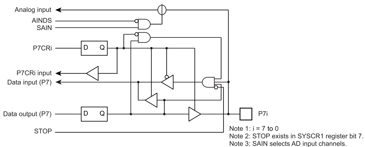
Figure 5-9 Port P7
