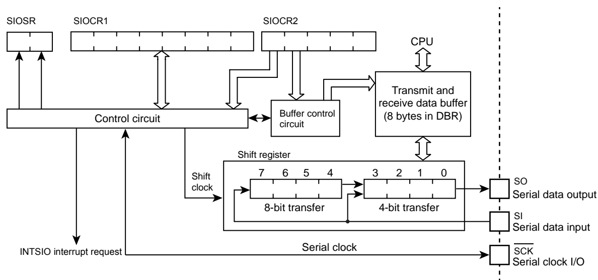
Figure 16-1 Serial Interface
