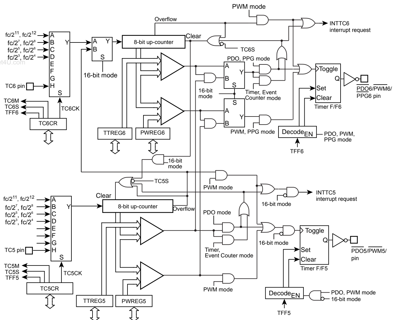
Figure 12-1 8-Bit TimerCounter 5, 6
