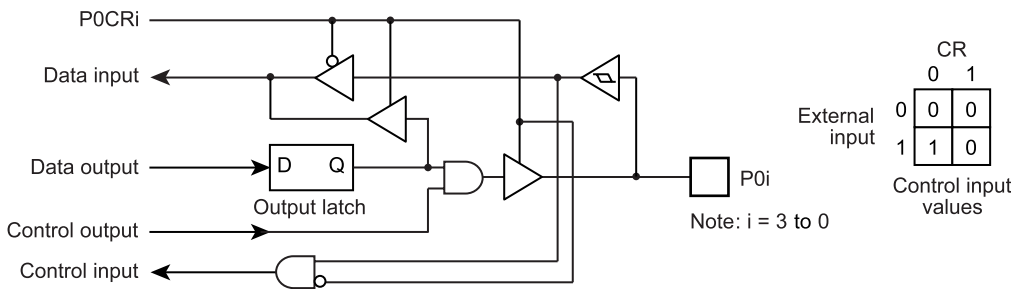
Figure 5-2 Port P0
