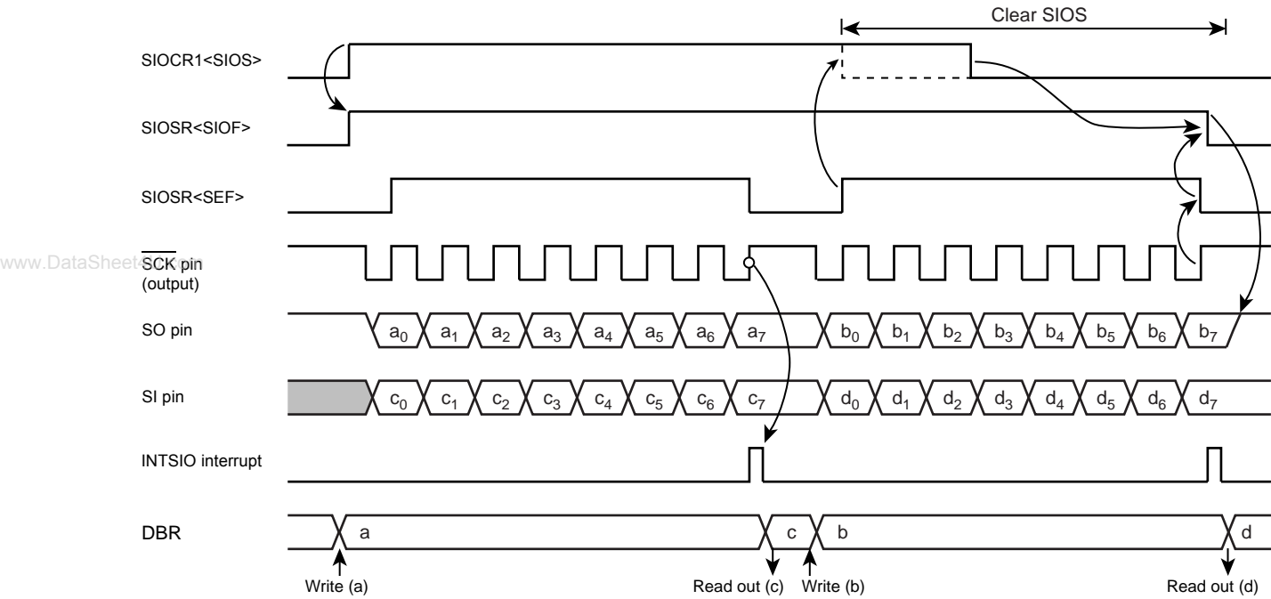
Figure 16-11 Transfer / Receive Mode (Example: 8bit, 1word transfer, Internal clock)
