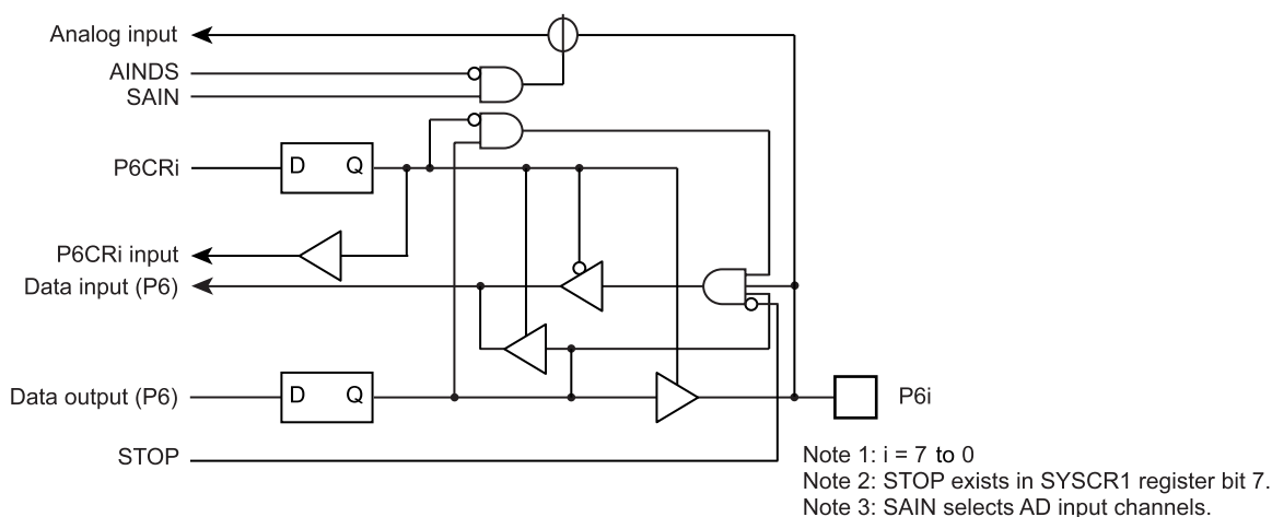
Figure 5-8 Port P6
