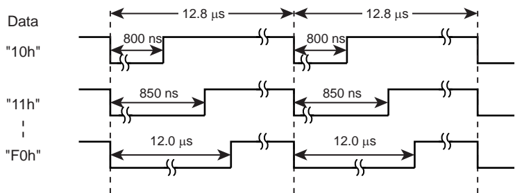
Figure 18-2 8-Bit Mode
