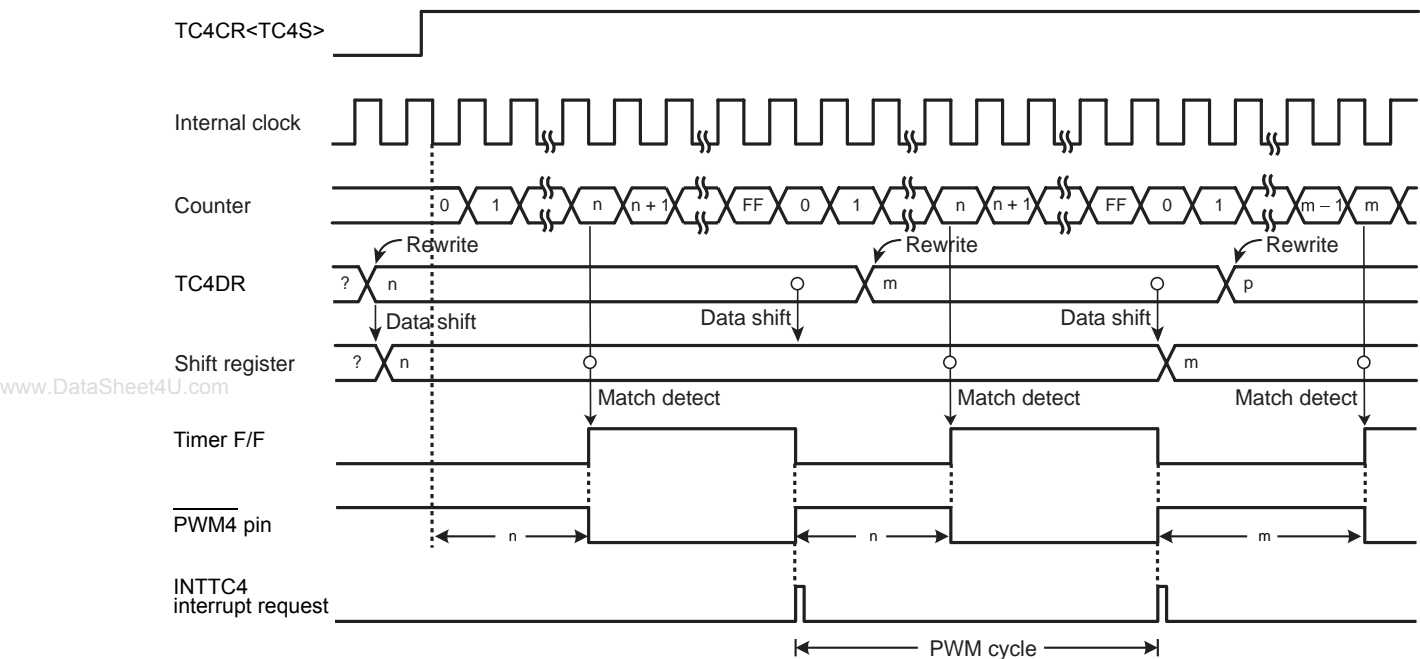
Figure 11-3 PWM output Mode Timing Chart (TC4)
