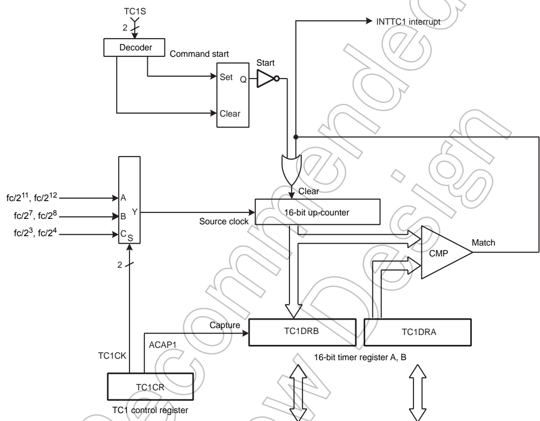
Figure 8-1 TimerCounter 1 (TC1)
