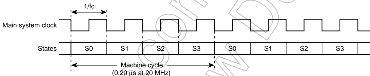
Figure 2-5 Machine Cycles
