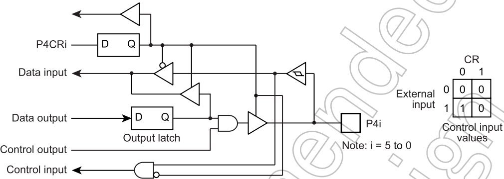
Figure 5-4 Port P4
