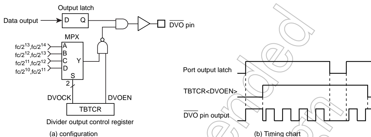
Figure 7-3 Divider Output
