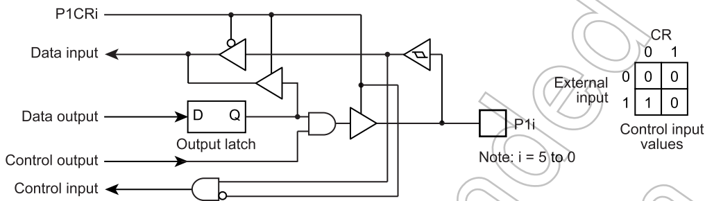
Figure 5-2 Port P1
