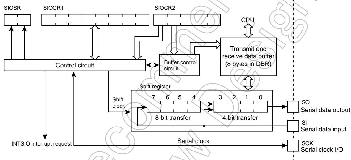
Figure 14-1 Serial Interface
