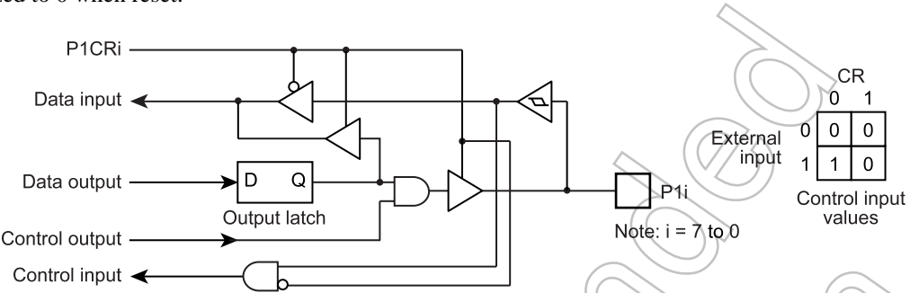
Figure 5-3 Port P1
