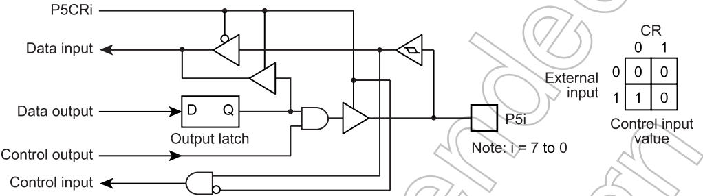
Figure 5-7 Port P5
