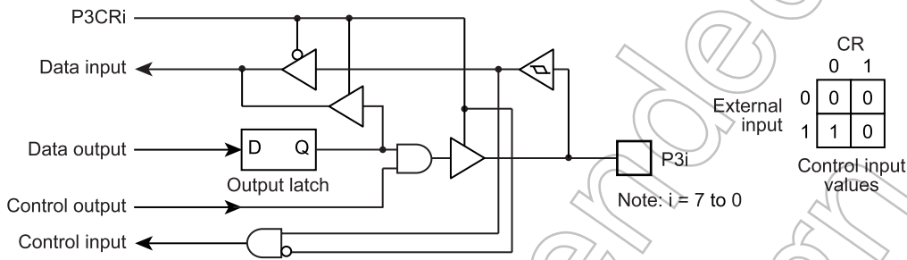
Figure 5-5 Port P3
