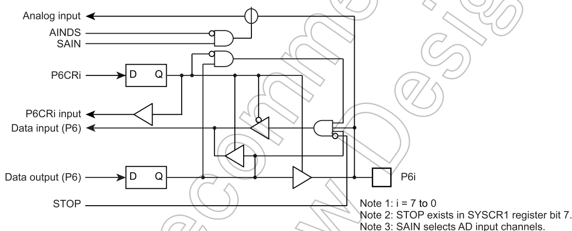
Figure 5-8 Port P6
