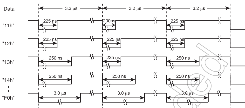
Figure 17-4 6-Bit Mode
