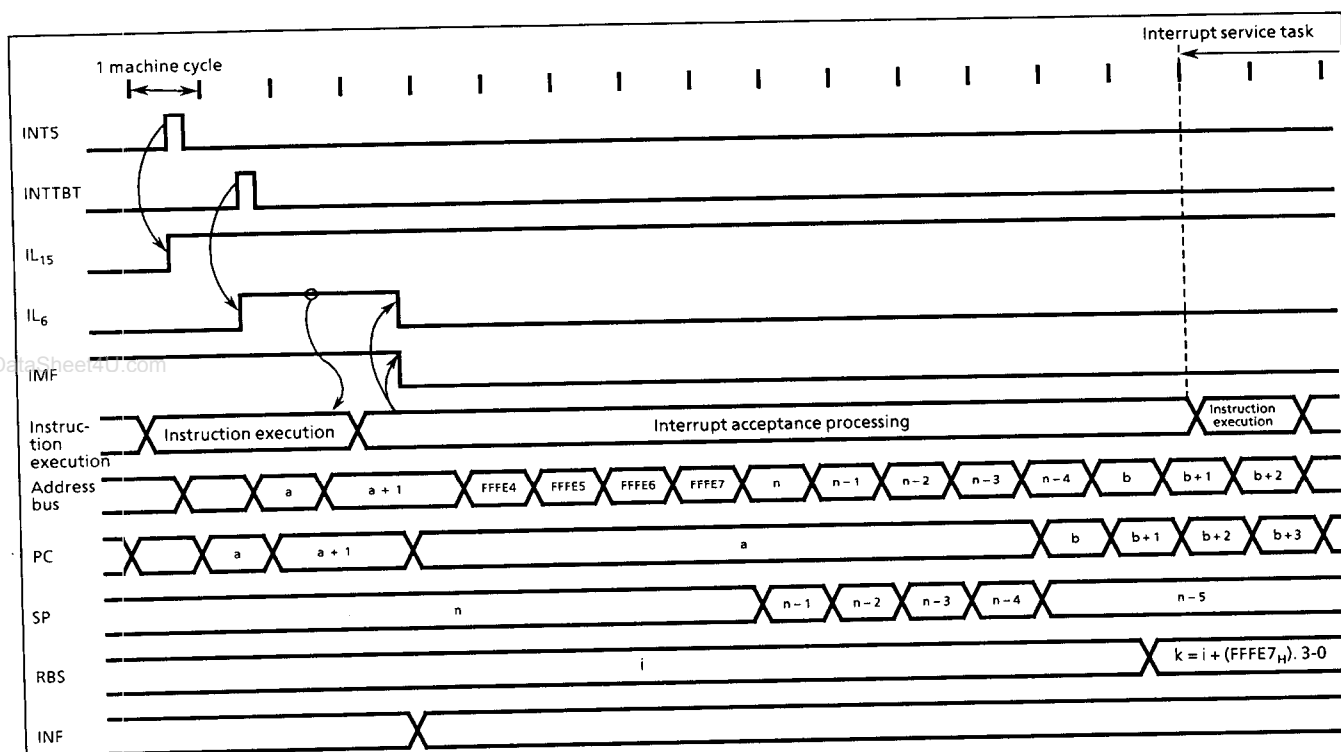
(a) Interrupt acceptance processing
