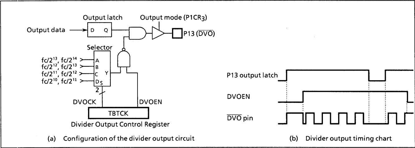
Figure 2-20. Divider Output
