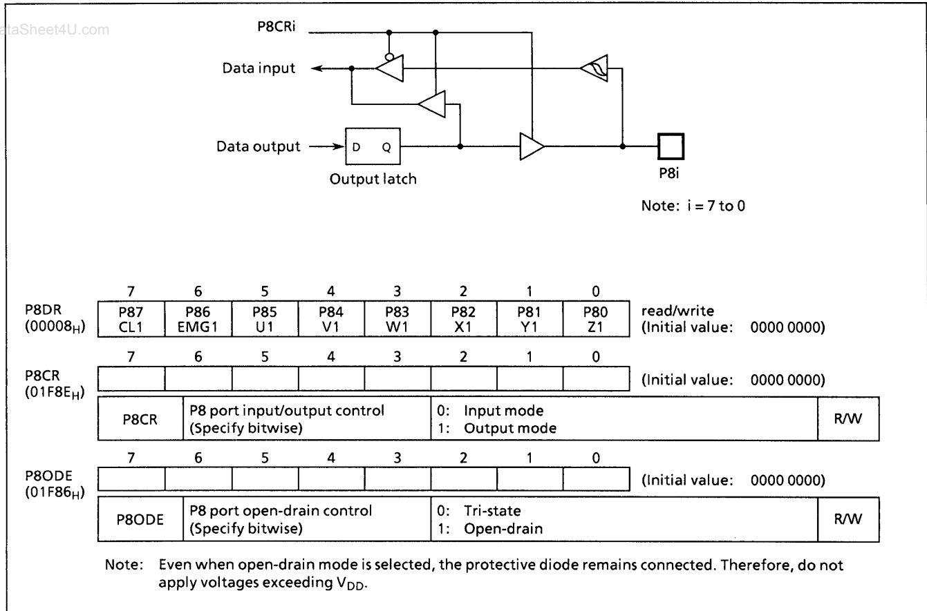
Figure 2-11. Port P8 and P8 Port Input/Output Registers
