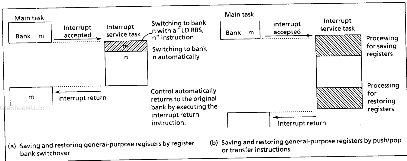
Figure 1-18. Saving and Restoring General-purpose Registers in Interrupt Processing
