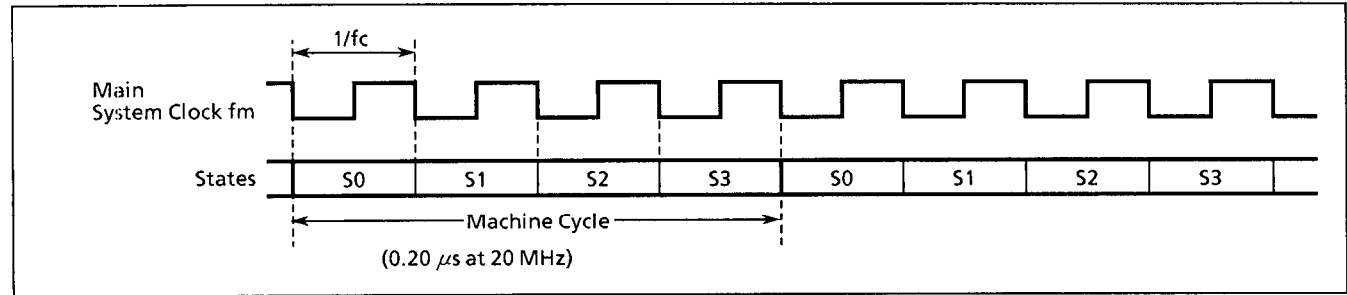
Figure 1-7. Machine Cycles
