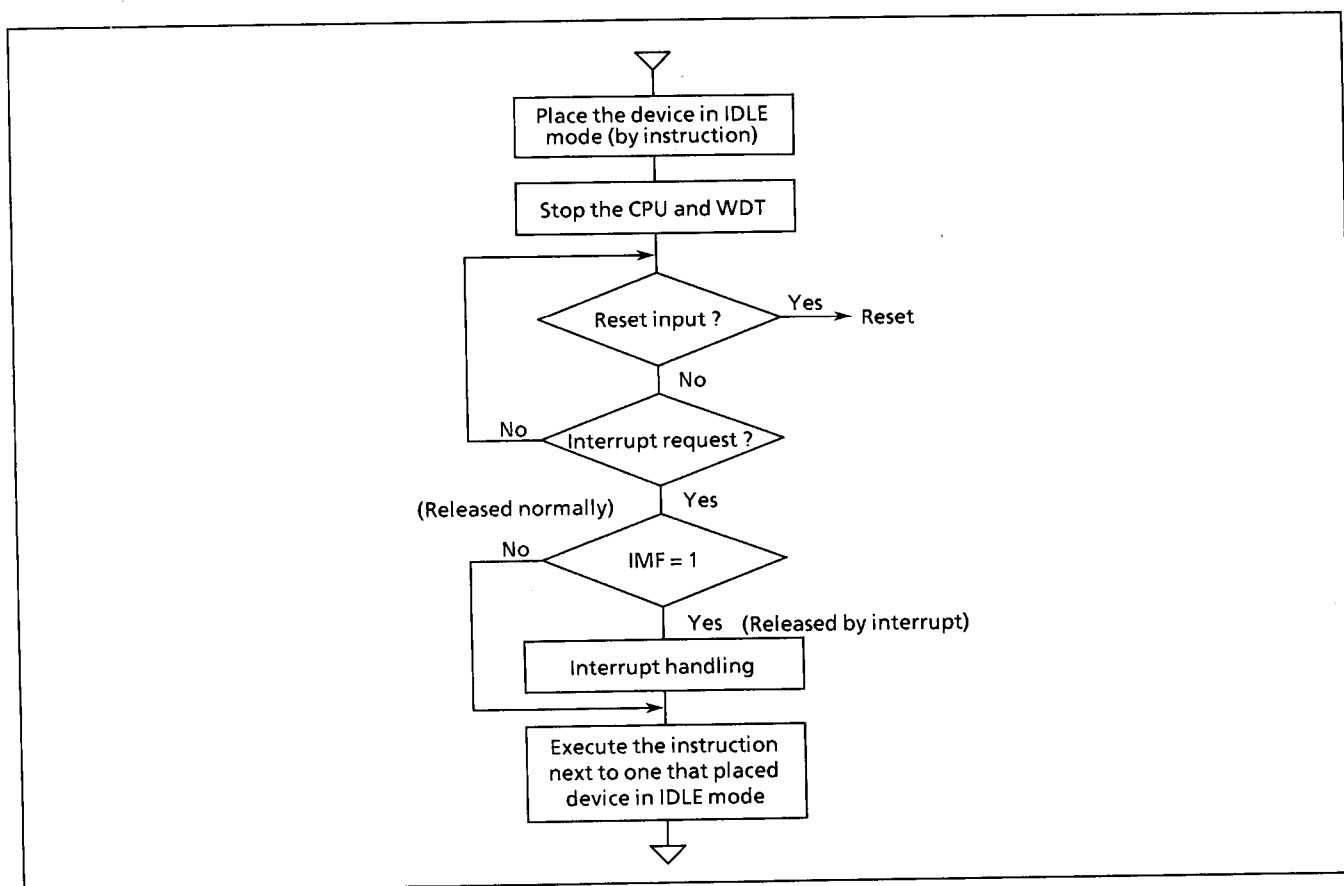
Figure 1-13. IDLE Mode
