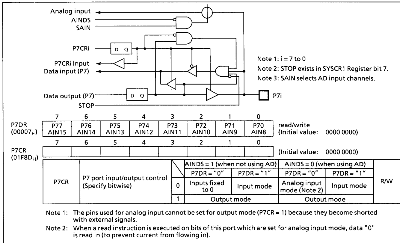
Figure 2-10. Port P7 and P7 Port Input/Output Registers
