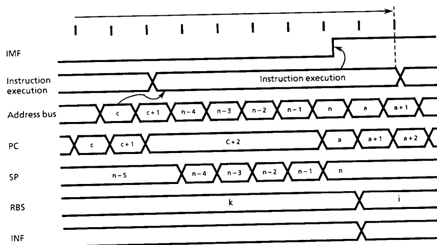
(b) Interrupt return instruction timing chart
