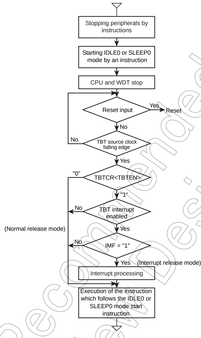
Figure 2-11 IDLE0 and SLEEP0 Modes
