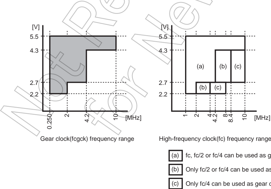
Figure 22-1 Clock gear (fcgck) and High-frequency clock (fc)
