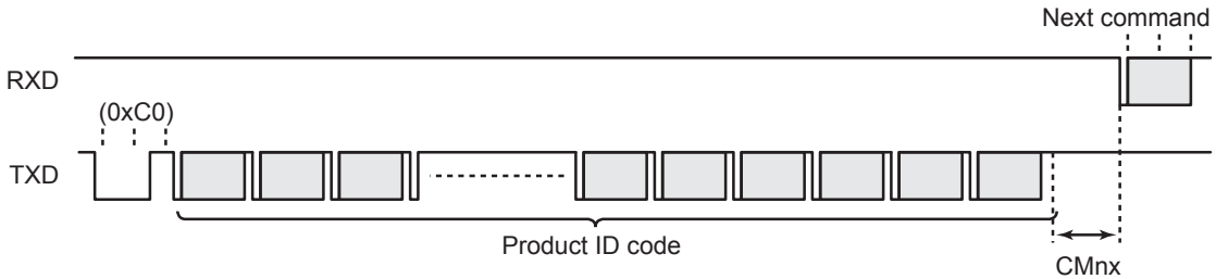
Figure 22-11 Product ID Code Output Command
