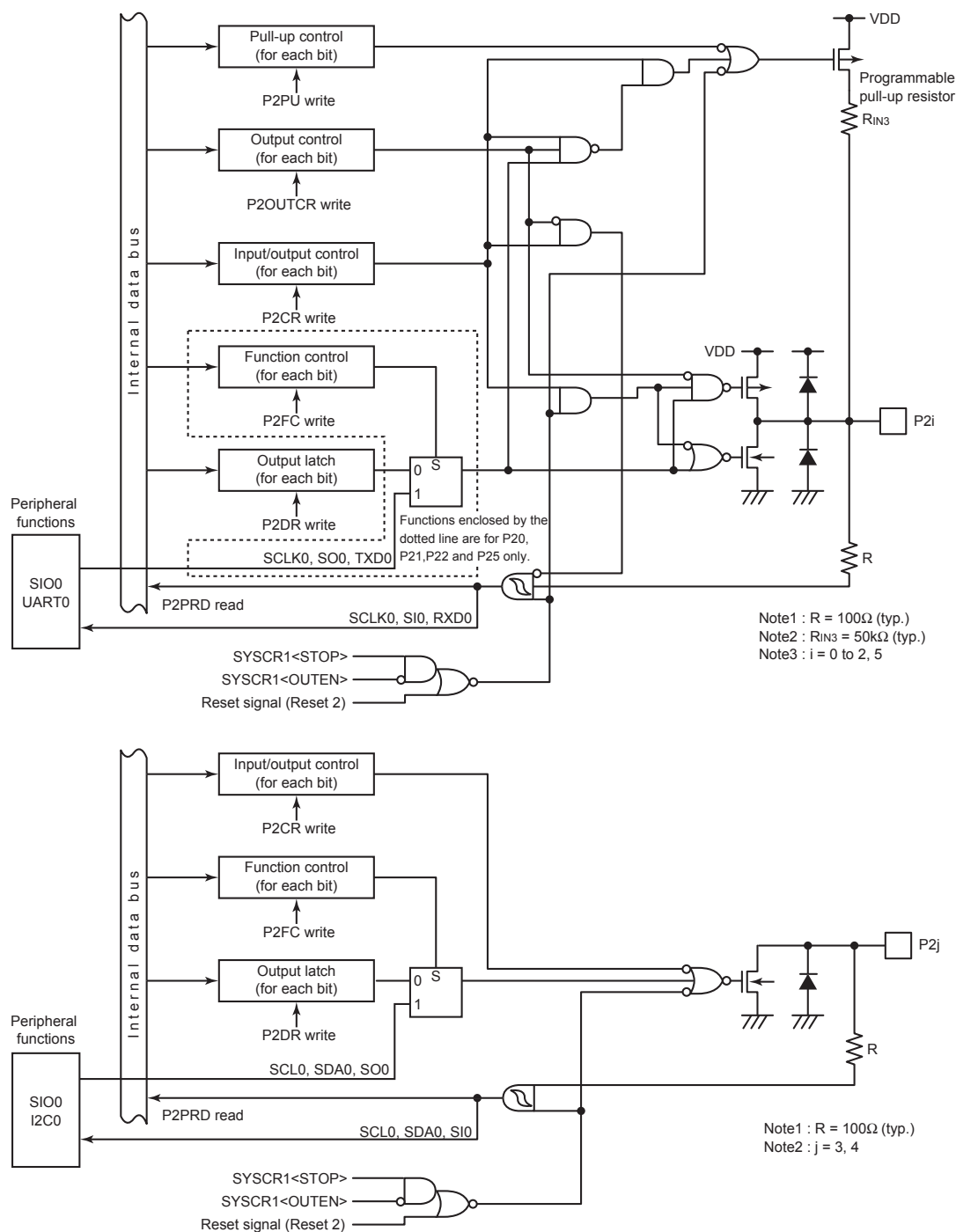
Figure 8-5 Port P2
