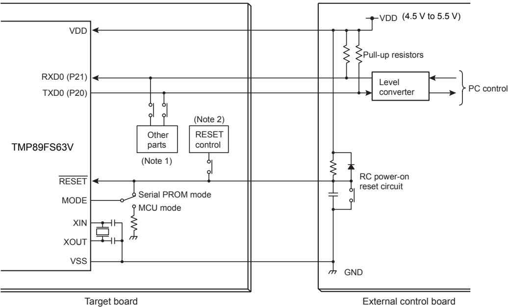
Figure 22-2 Example Connections for On-board Writing
