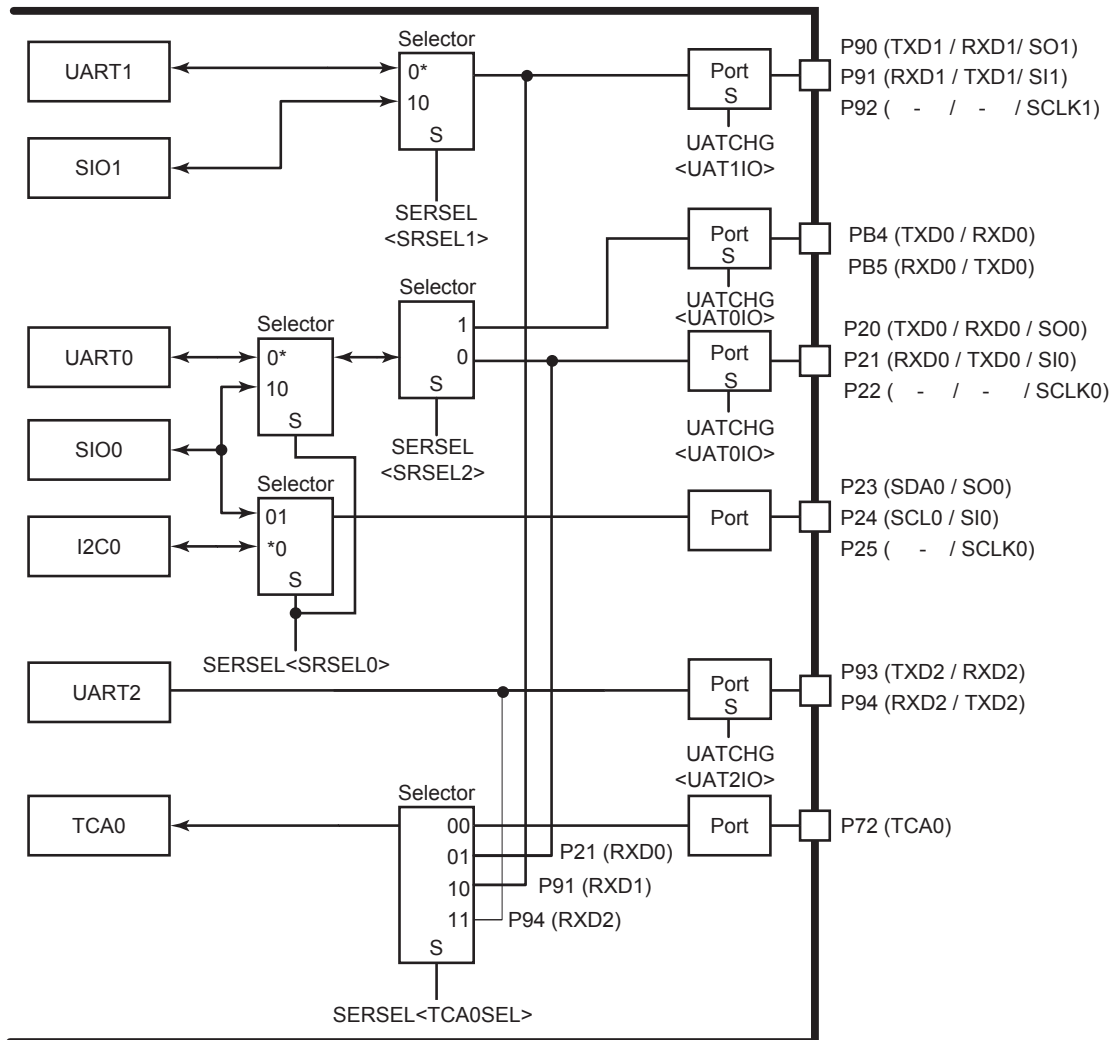
Figure 8-12 Serial Interface Selecting Function
