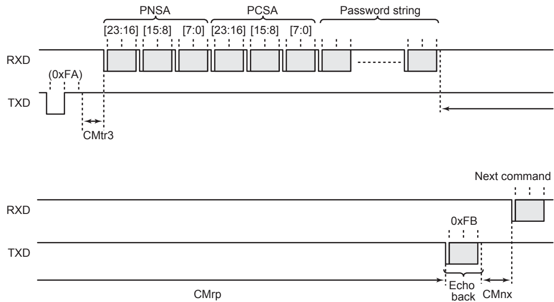
Figure 22-14 Flash Memory Security Setting Command
