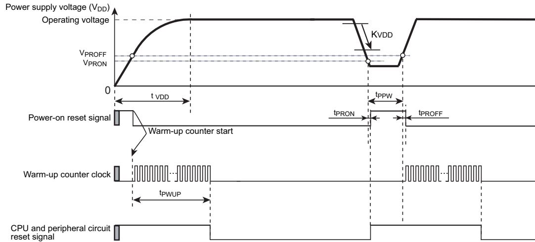
Figure 25-6 Power-on Reset Operation Timing
