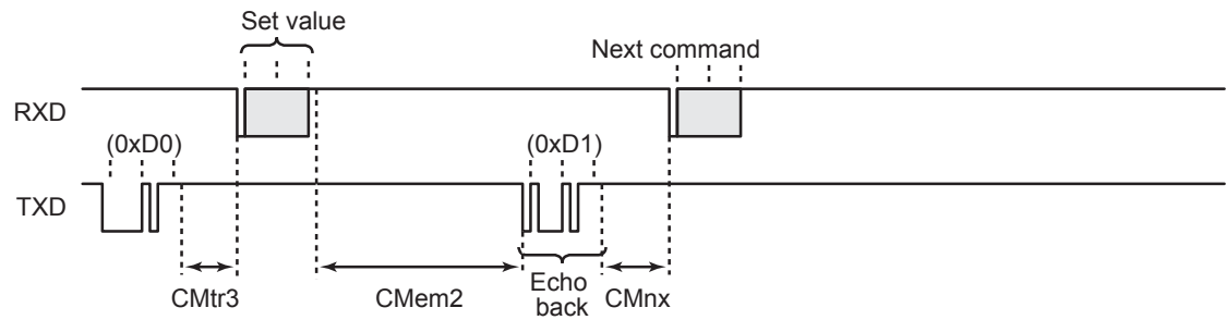
Figure 22-13 Mask ROM Emulation Setting Command
