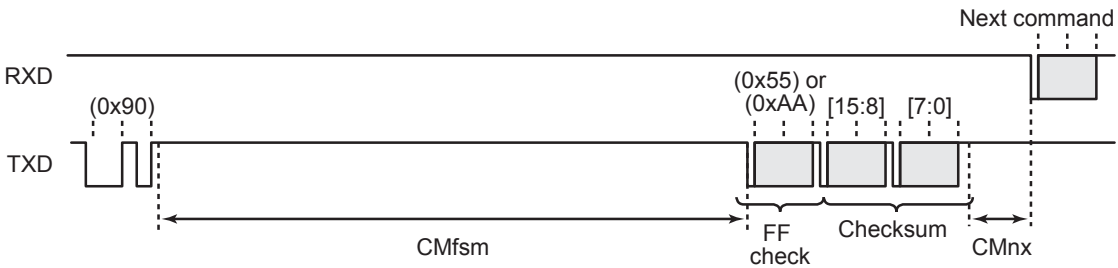
Figure 22-10 Flash Memory SUM Output Command
