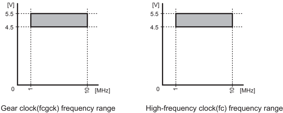
Figure 25-3 Clock gear (fcgck) and High-frequency clock (fc)
