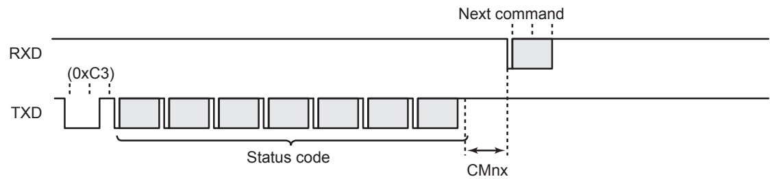
Figure 22-12 Flash Memory Status Output Command
