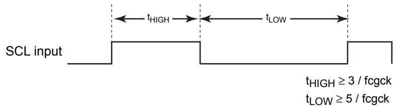
Figure 18-7 SCL Input
