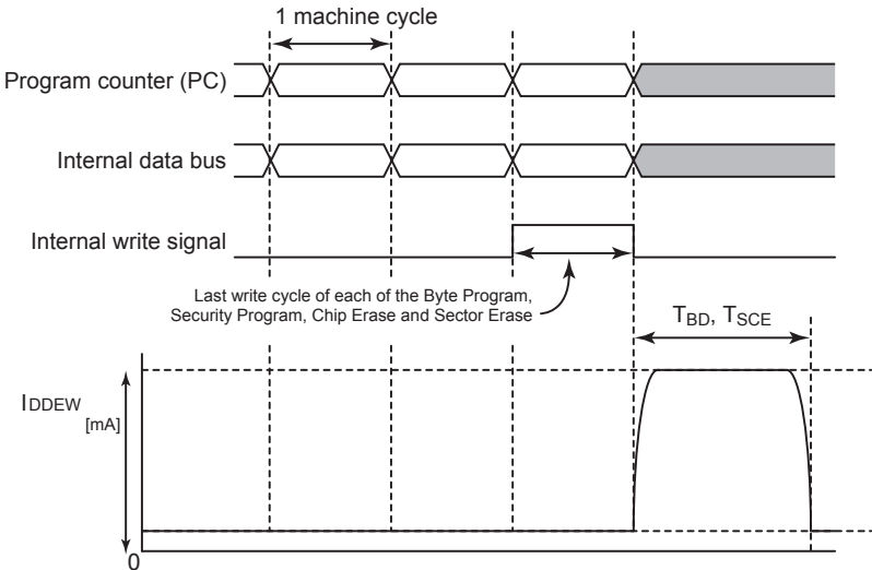
Figure 25-5 Current When an Erase or Write is Being Performed on the Flash Memory
