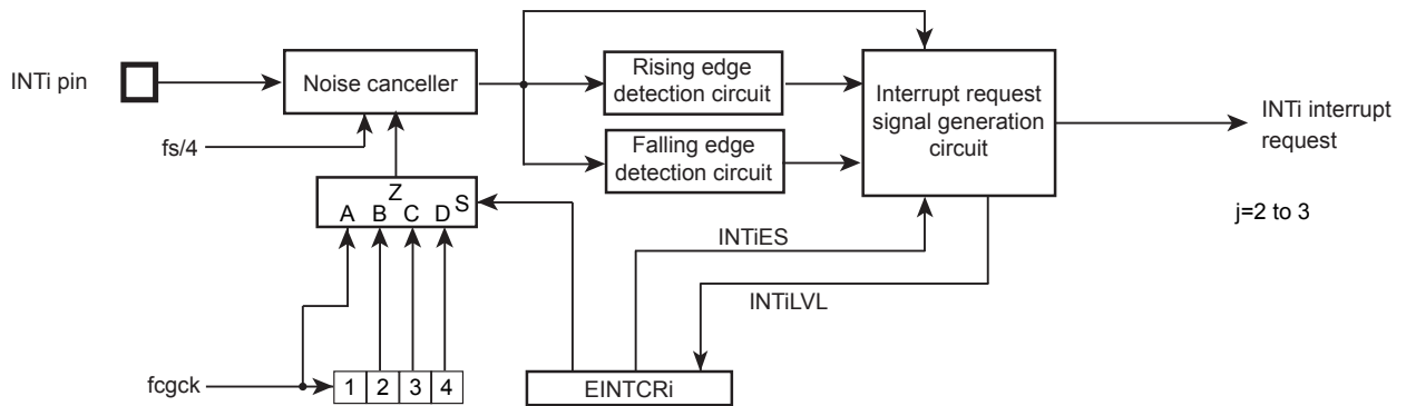
Figure 4-2 External Interrupts 2/3
