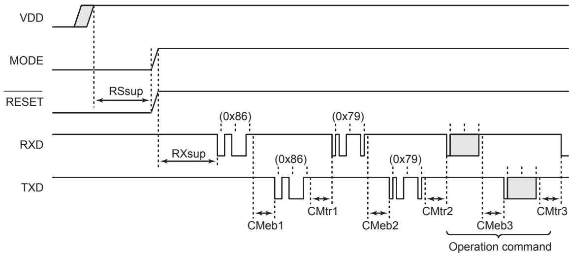
Figure 22-6 Reset Timing
