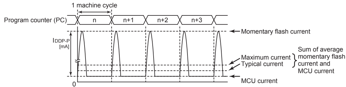
Figure 25-4 Intermittent Operation of Flash Memory
