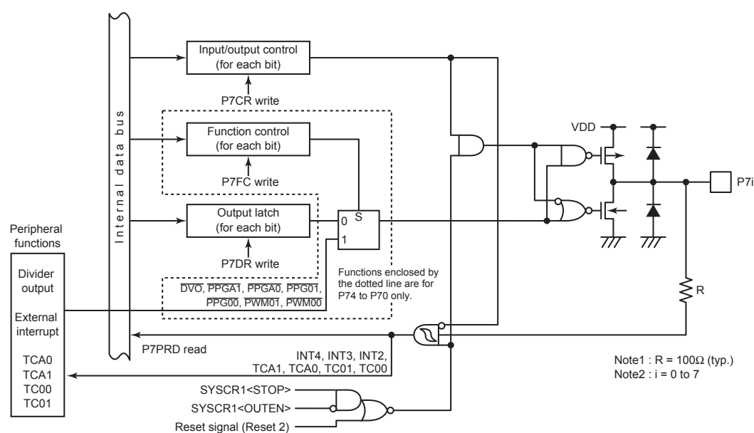
Figure 8-8 Port P7
