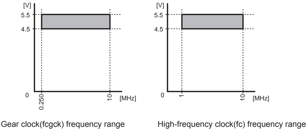
Figure 25-1 Clock gear (fcgck) and High-frequency clock (fc)
