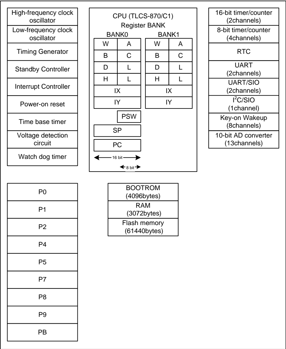
Figure 1-2 Block Diagram
