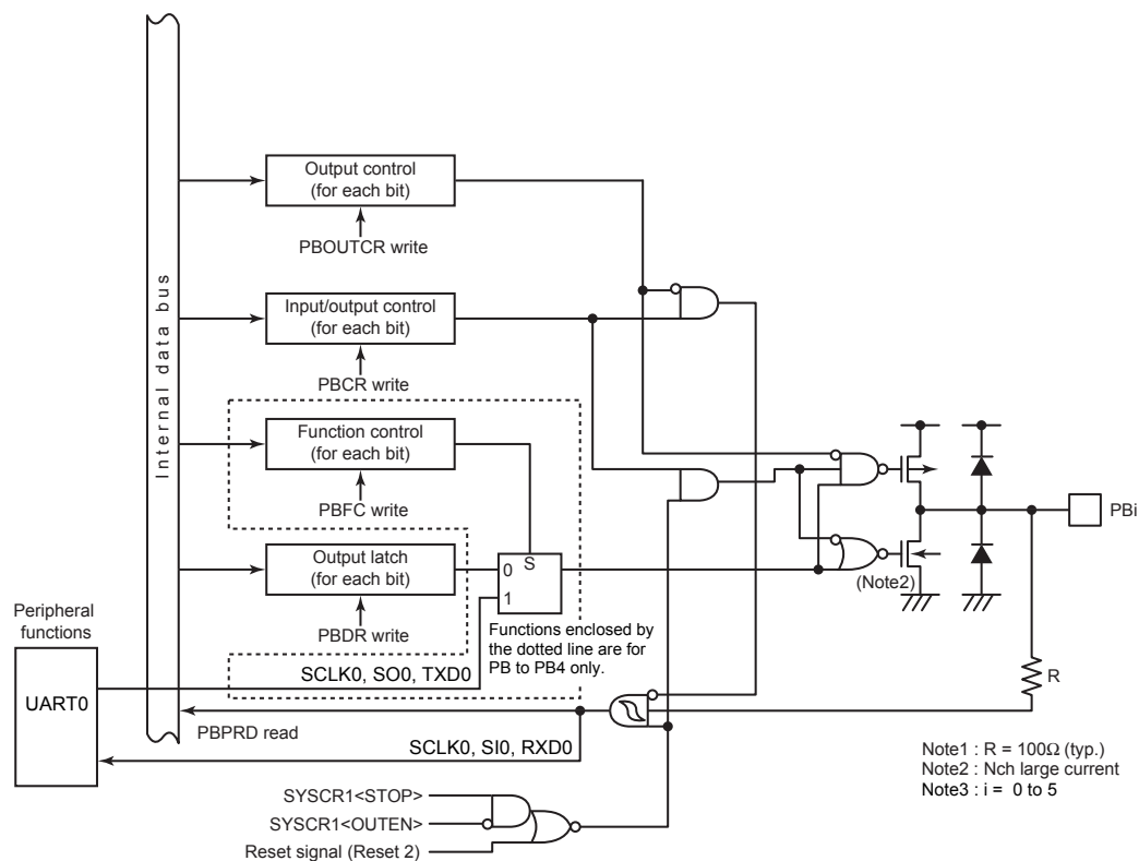
Figure 8-11 Port PB
