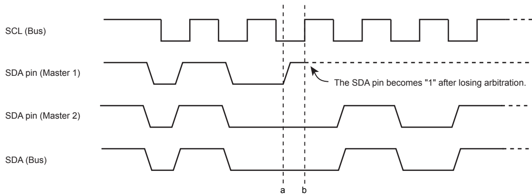
Figure 18-12 Arbitration Lost
