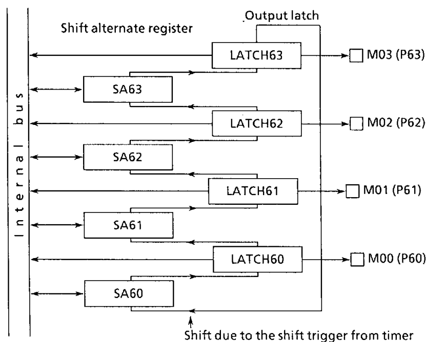
Figure 3.8 (5) Pattern Generation Mode Block Diagram (Port 6)
