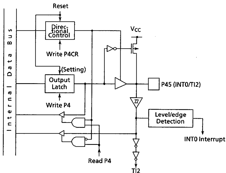
Figure 3.5 (11) Port 4 (P45)
