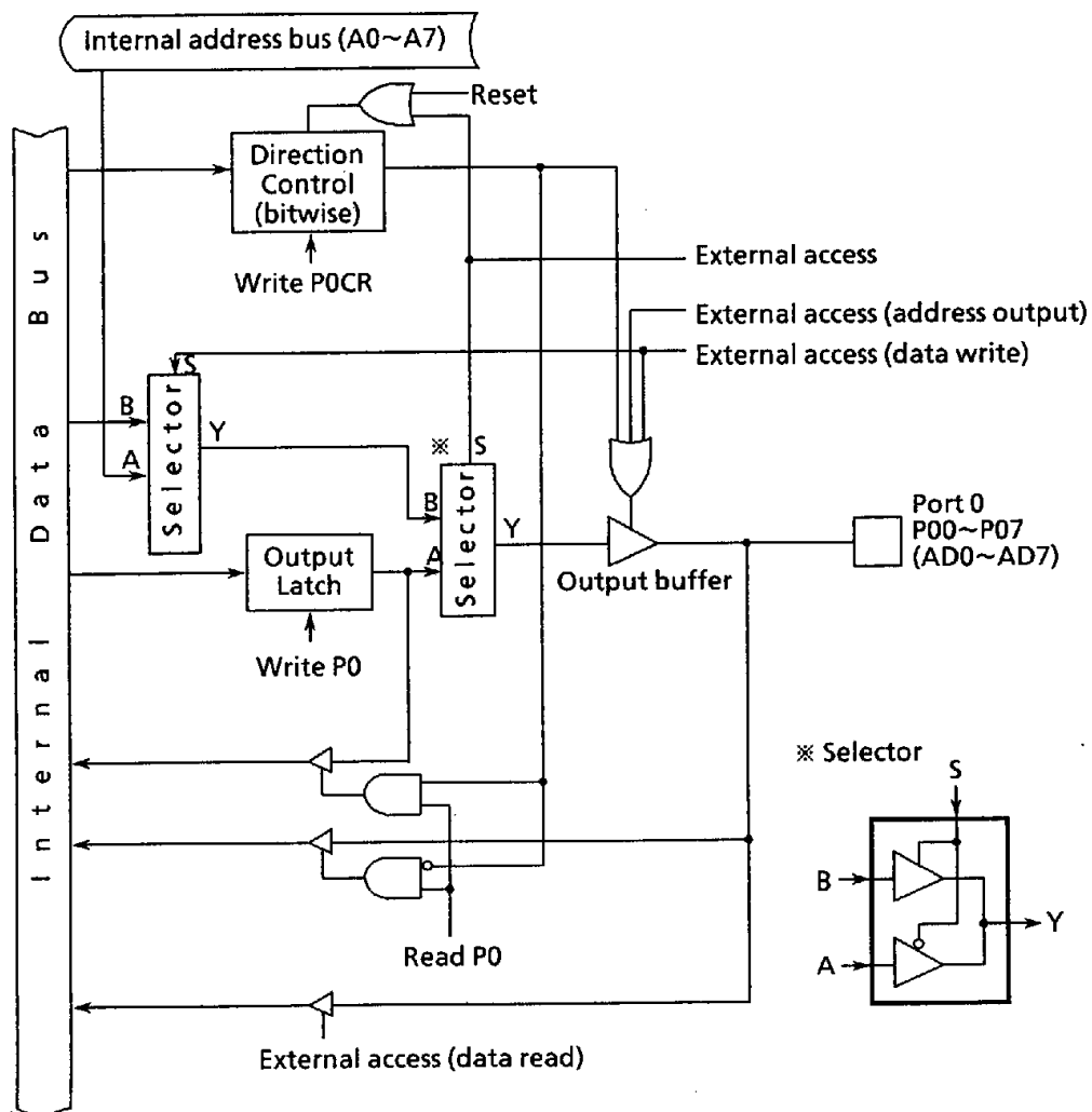
Figure 3.5 (1) Port 0 (P00~P07)
