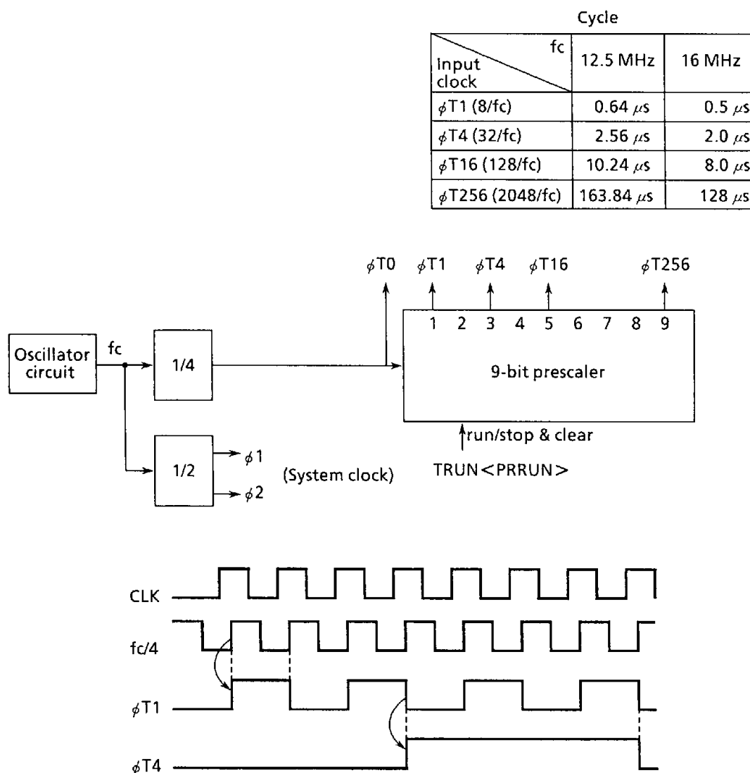
Figure 3.6 (2) Prescaler
