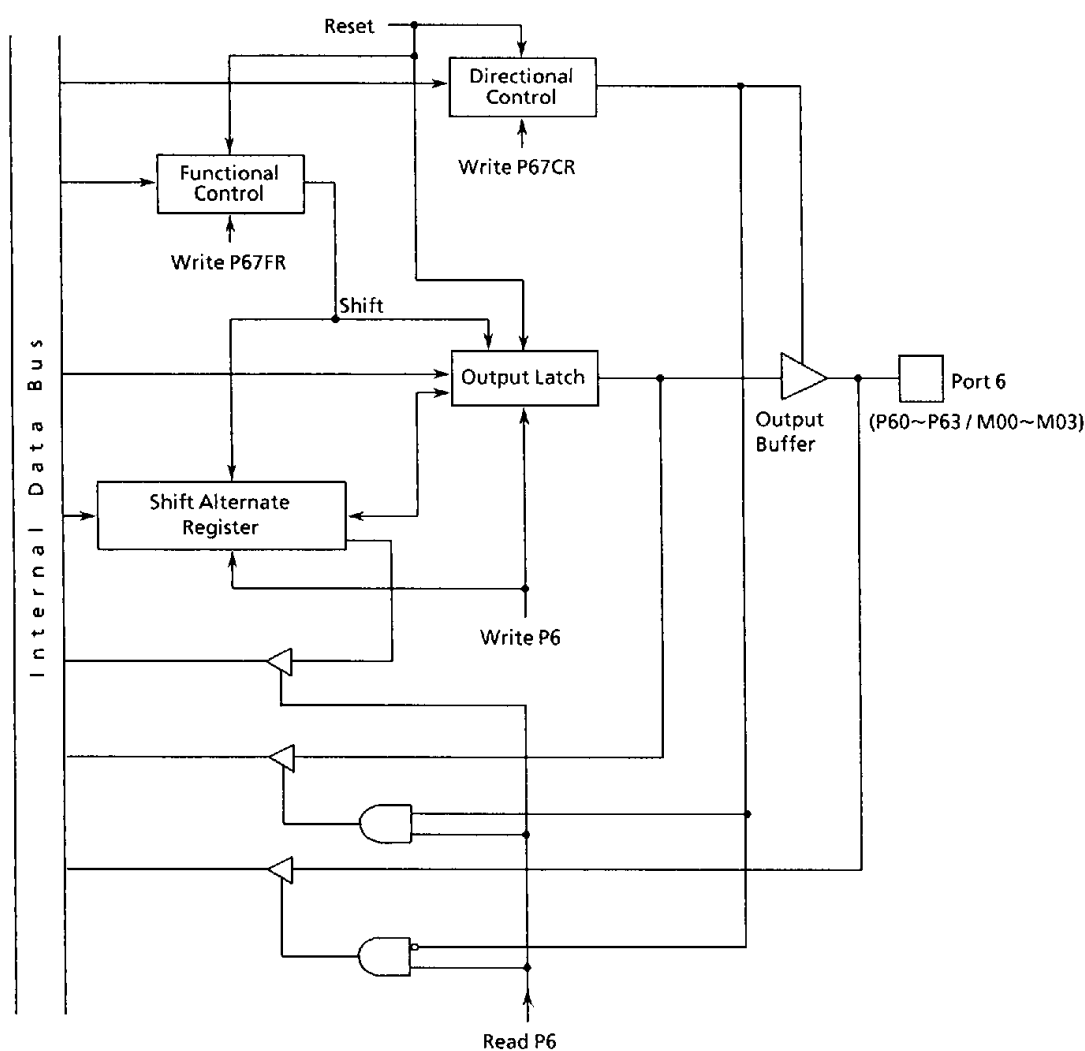
Figure 3.5 (16) Port 6
