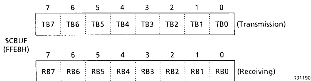
Figure 3.9 (4) Serial Transmission/Receiving Buffer Registers (SCBUF)
