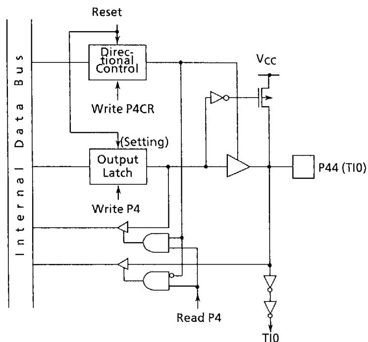
Figure 3.5 (10) Port 4 (P44)
