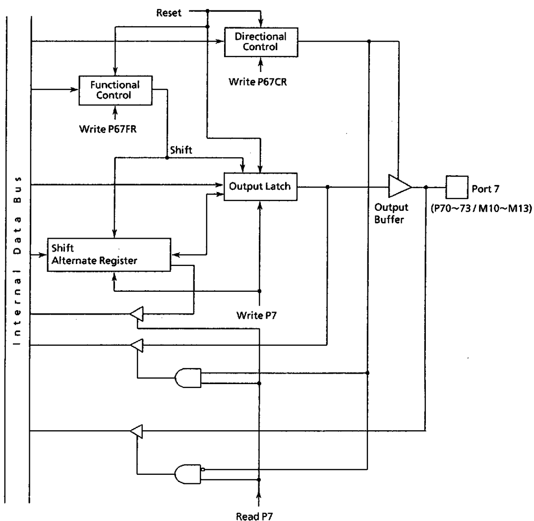
Figure 3.5 (17) Port 7
