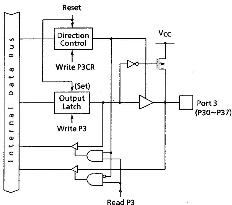
Figure 3.5 (7) Port 3
