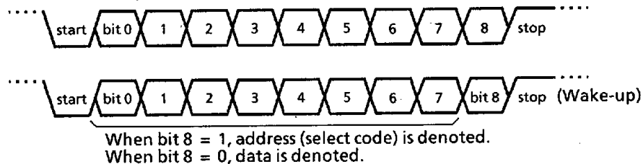
Figure 3.9 (1) Data Formats
