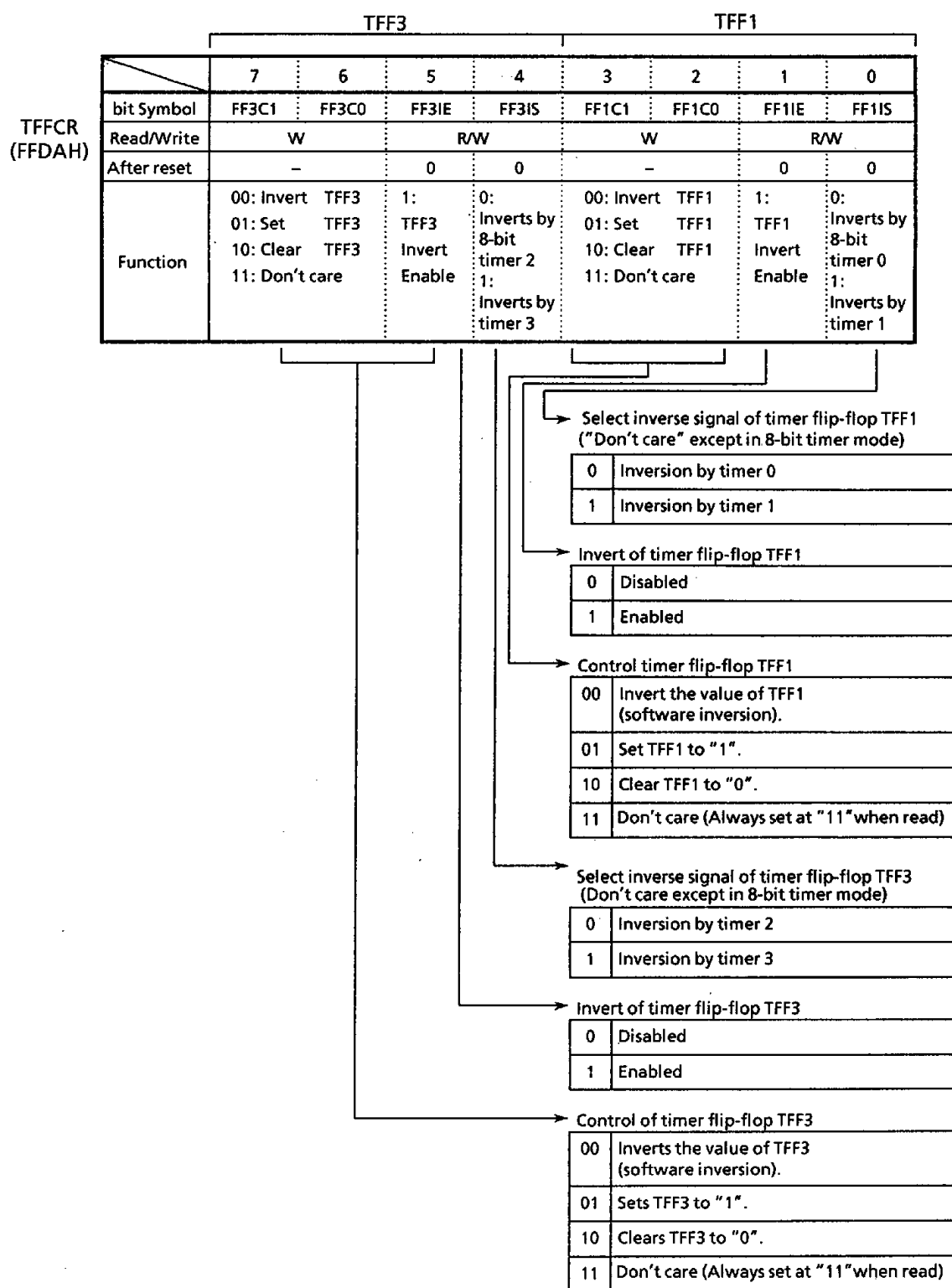
Figure 3.6 (6) 8-Bit Timer Flip-flop Control Register (TFFCR)
