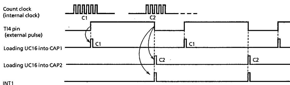
Figure 3.7 (7) Pulse Width Measurement
