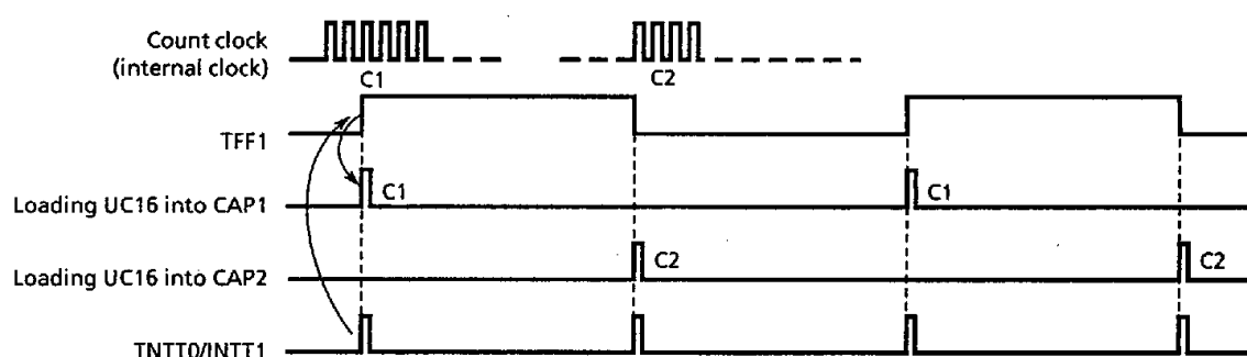
Figure 3.7 (6) Frequency Measurement
