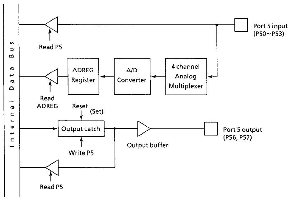
Figure 3.5 (14) Port 5
