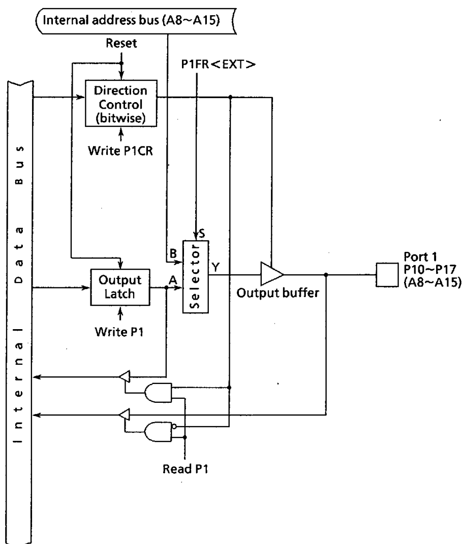
Figure 3.5 (3) Port 1 (P10~P17)
