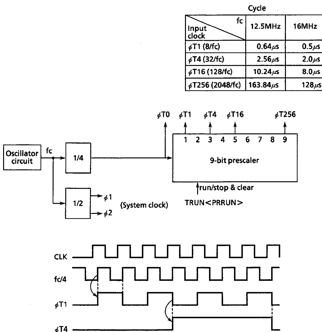
Figure 3.6 (2) Prescaler
