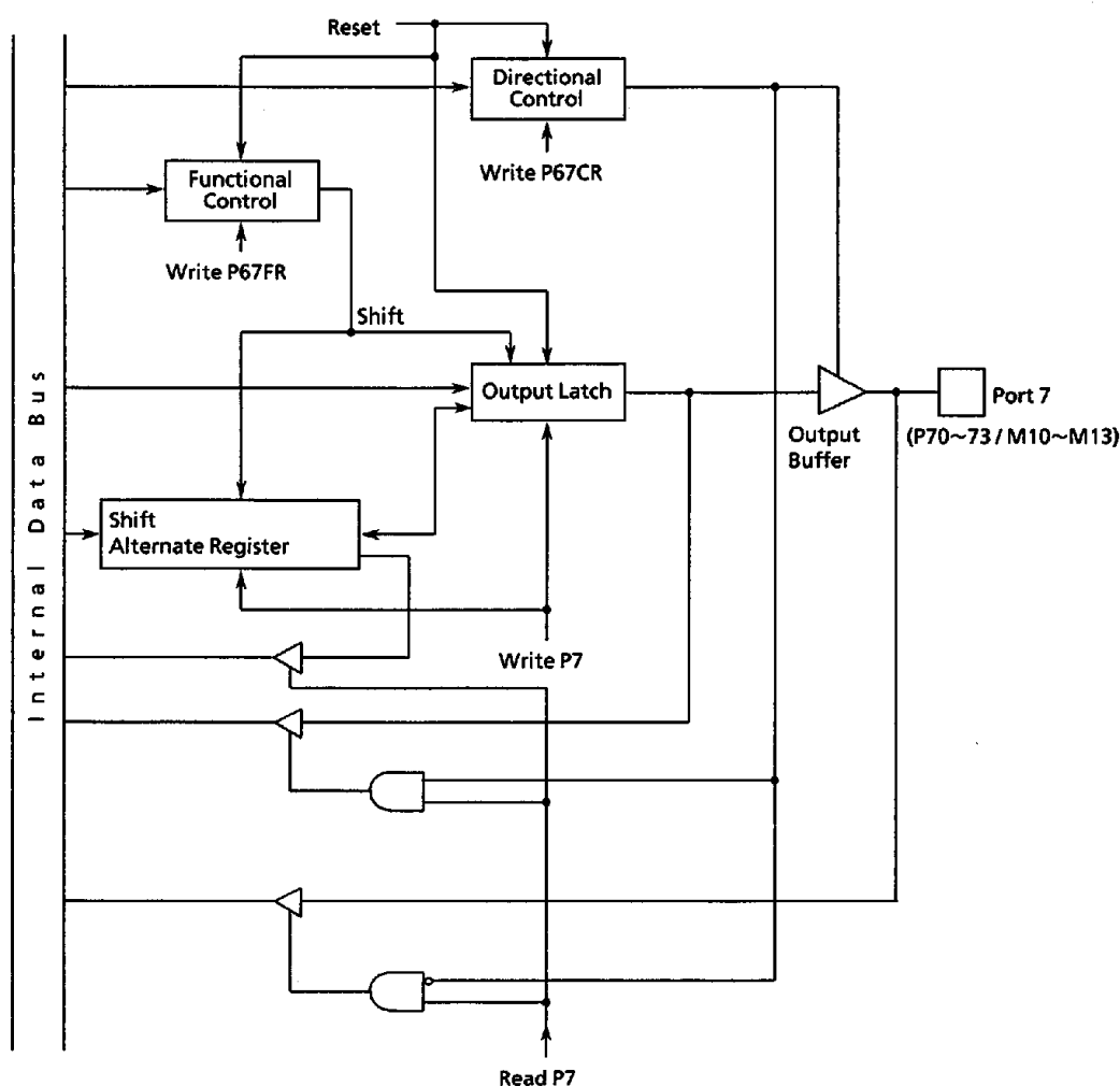
Figure 3.5 (17) Port 7
