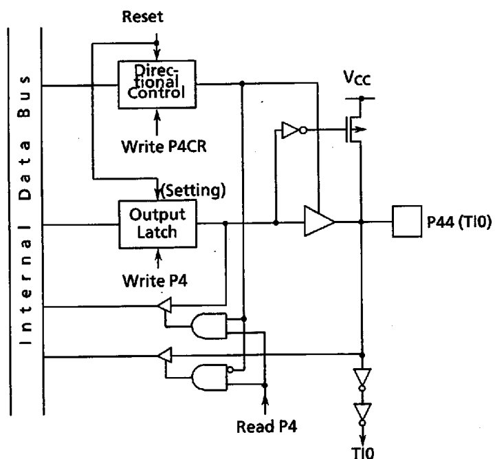
Figure 3.5 (10) Port 4 (P44)
