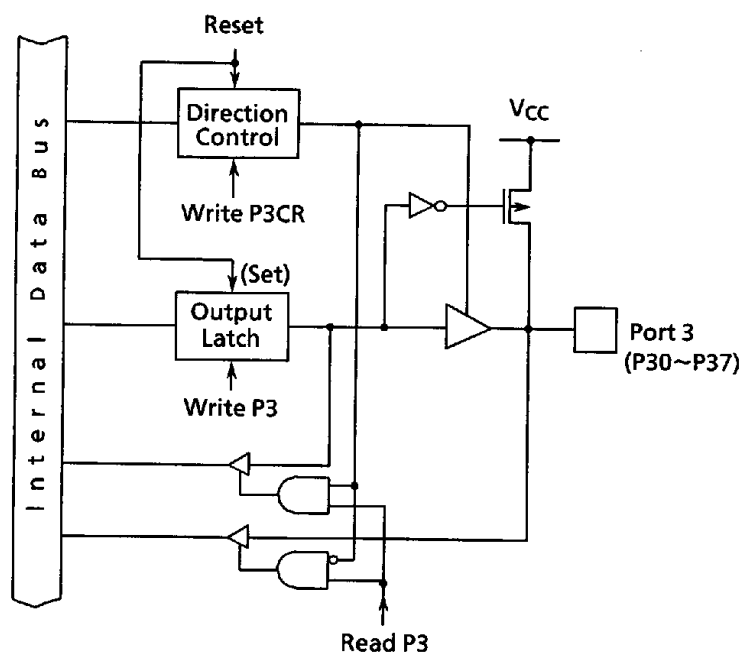
Figure 3.5 (7) Port 3
