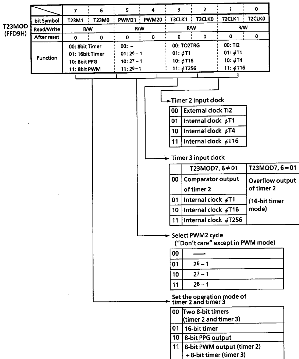
Figure 3.6 (5) Timer 2/Timer 3 Mode Register (T23MOD)
