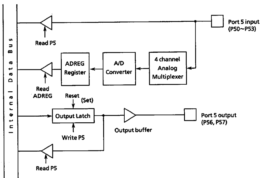
Figure 3.5 (14) Port 5
