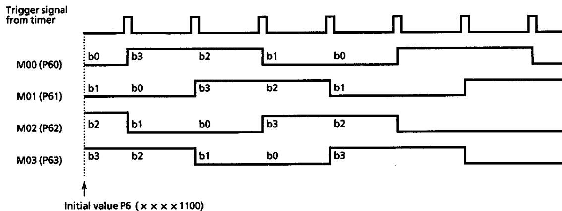
Figure 3.8 (7) Output Waveforms of 4-Phase 2-step Excitation (Normal Rotation)
