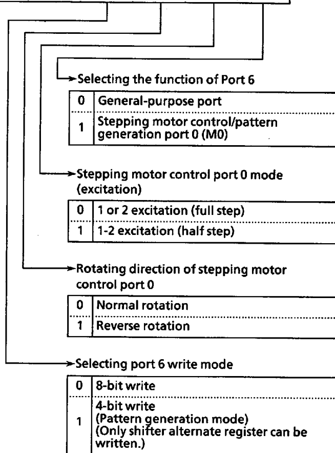
Figure 3.8 (2a) Port 6 and Port 7 Function Control Register (P67FR)
