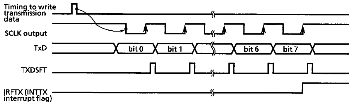
Figure 3.9 (9) Transmitting Operation in I/O Interface Mode (SCLK Output Mode)
