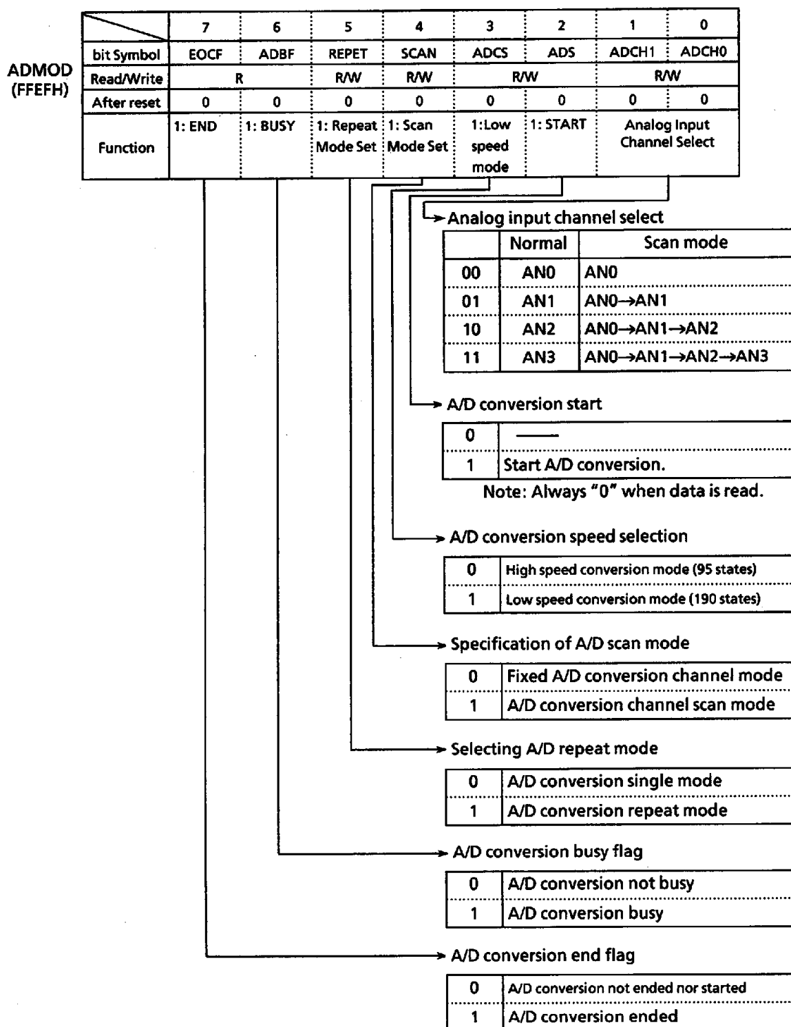
Figure 3.10 (2) A/D Conversion Mode Register (ADMOD)
