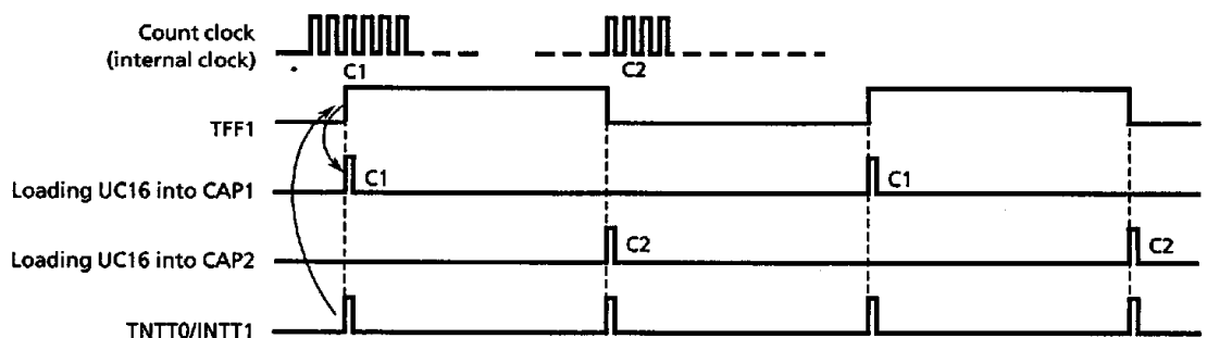
Figure 3.7 (6) Frequency Measurement
