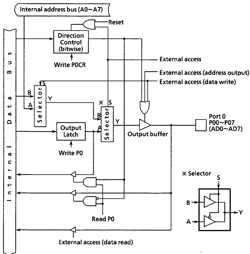
Figure 3.5 (1) Port 0 (P00~P07)
