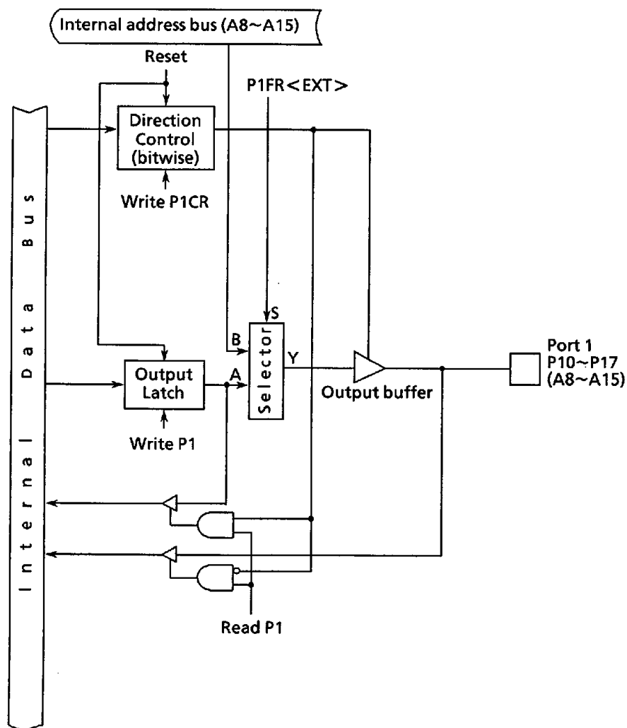
Figure 3.5 (3) Port 1 (P10~P17)
