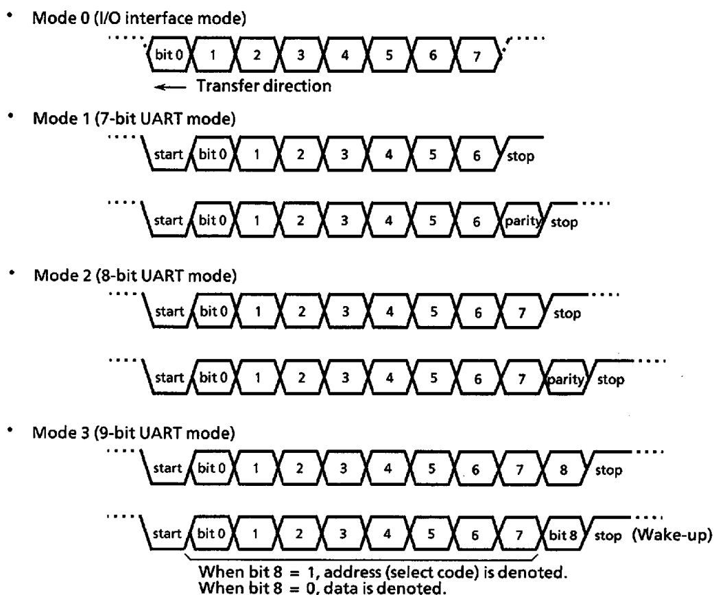
Figure 3.9 (1) Data Formats
