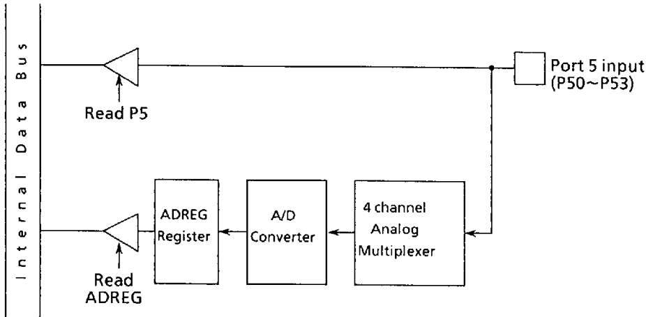
Figure 3.5 (12) Port 5
