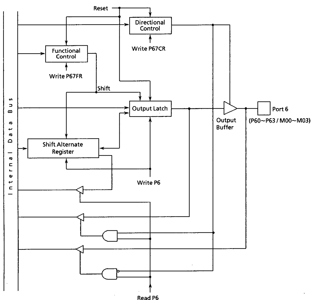
Figure 3.5 (14) Port 6
