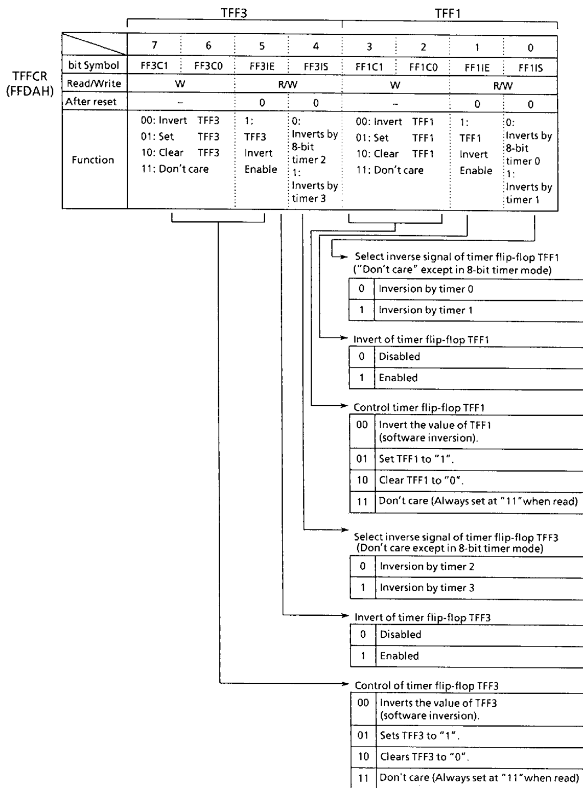
Figure 3.8 (6) 8-Bit Timer Flip-Flop Control Register (TFFCR)
