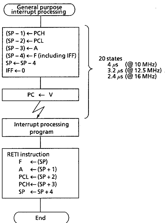
Figure 3.3 (2) General Purpose Interrupt Processing
