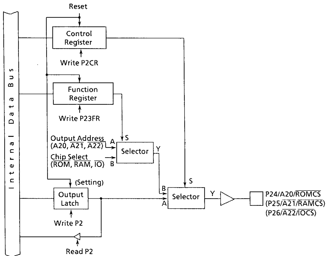
Figure 3.5 (2) Port 2 (P24~P26)
