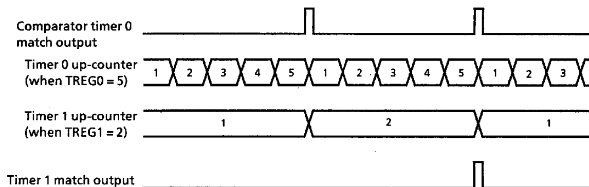
Figure 3.8 (10)
