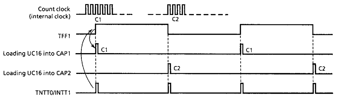
Figure 3.9 (6) Frequency Measurement
