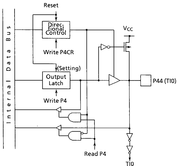
Figure 3.5 (8) Port 4 (P44)
