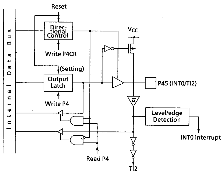
Figure 3.5 (9) Port 4 (P45)
