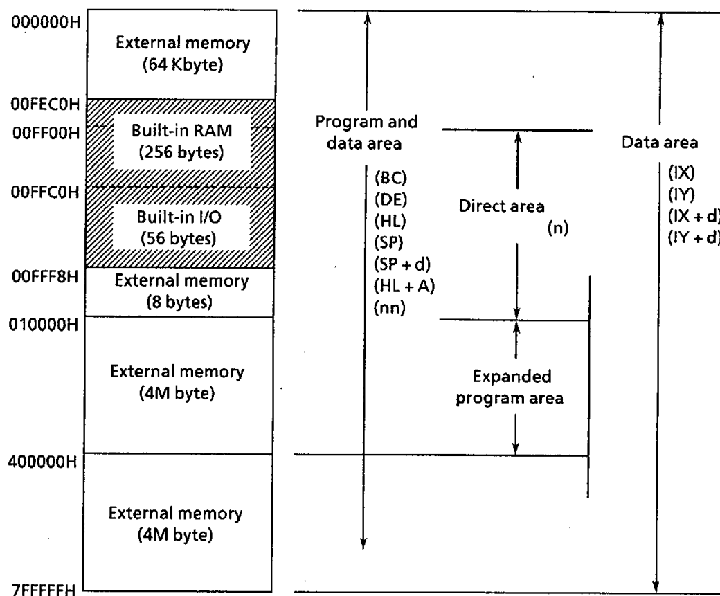
Figure 3.2 Memory Map
