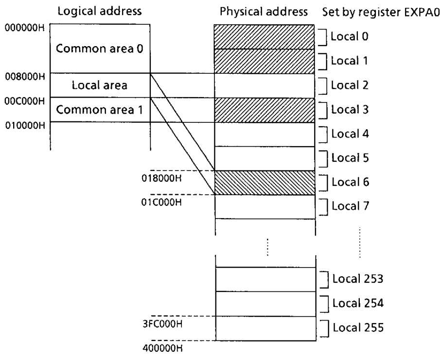
Figure 3.6 (2) Memory Map Using the Program Space Extension Function
