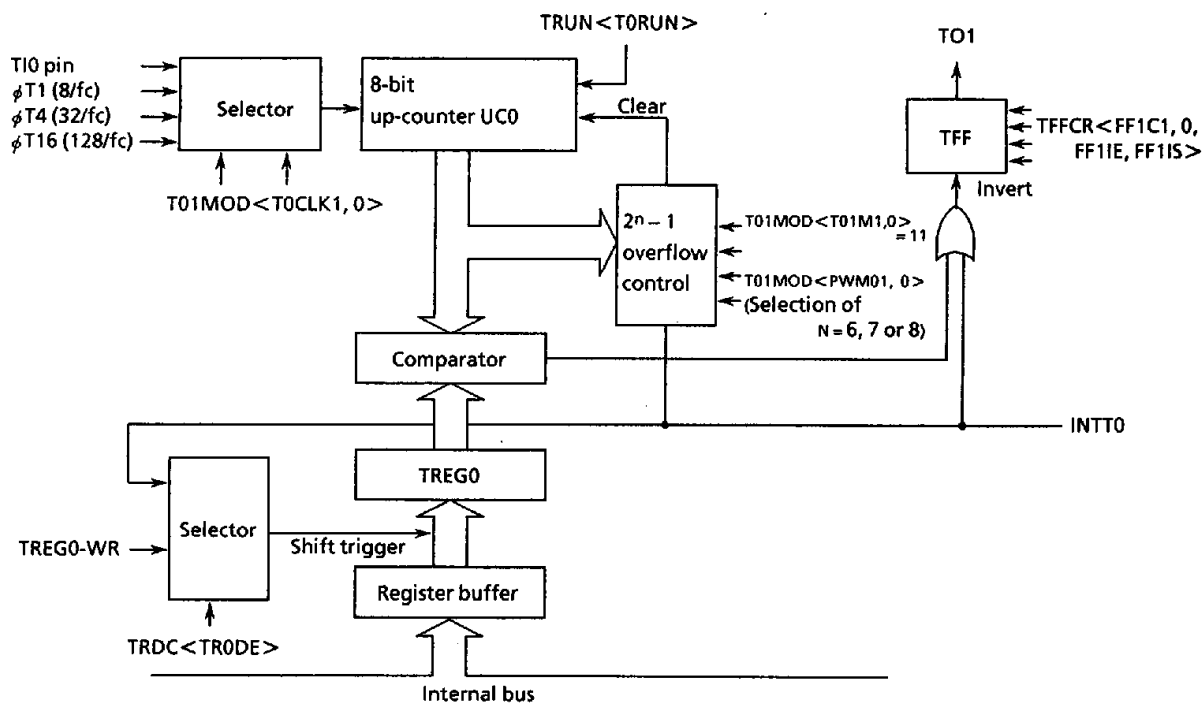
Figure 3.8 (13) Block Diagram of 8-Bit PWM Mode
