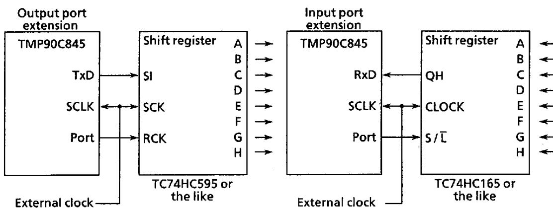
Figure 3.11 (8) I/O Interface Mode
