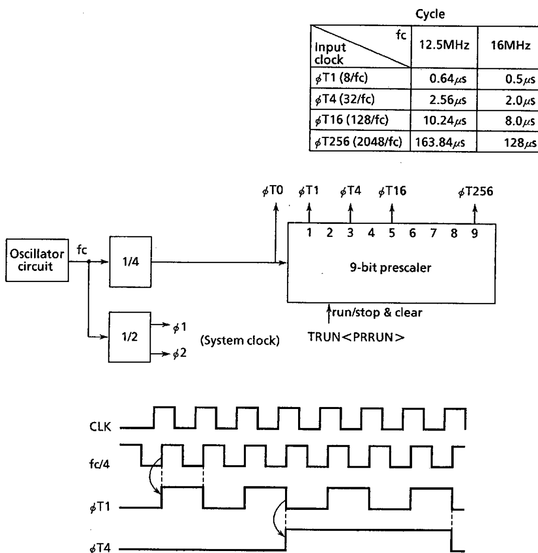
Figure 3.8 (2) Prescaler
