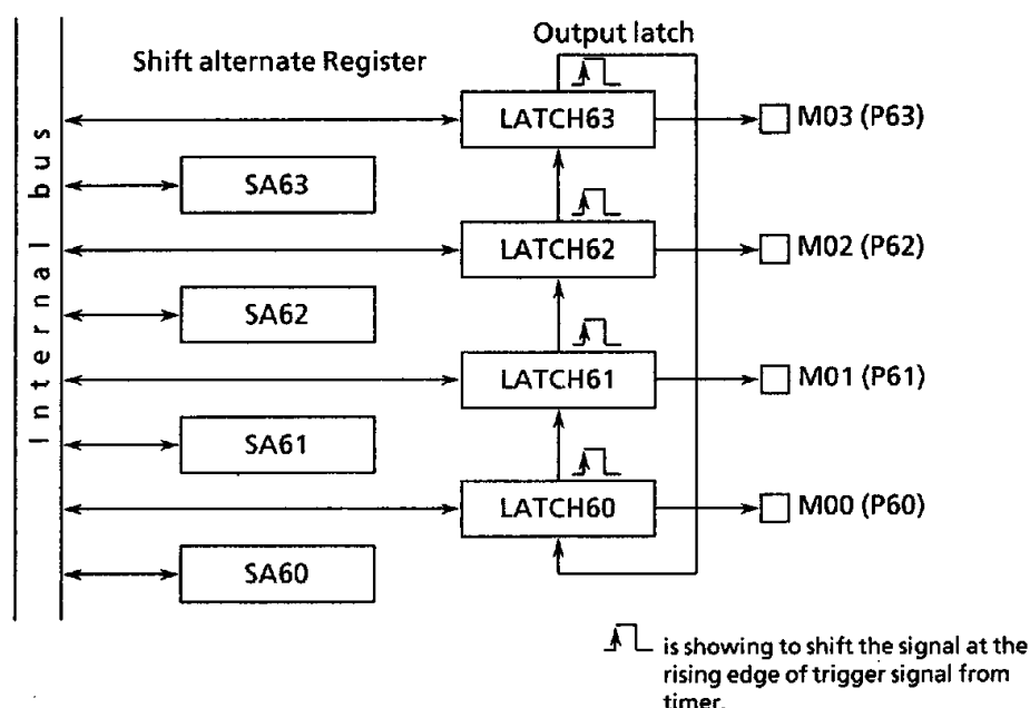
Figure 3.10 (8) Block Diagram of 4-Phase 1-step Excitation/2-step Excitation (Normal Rotation)
