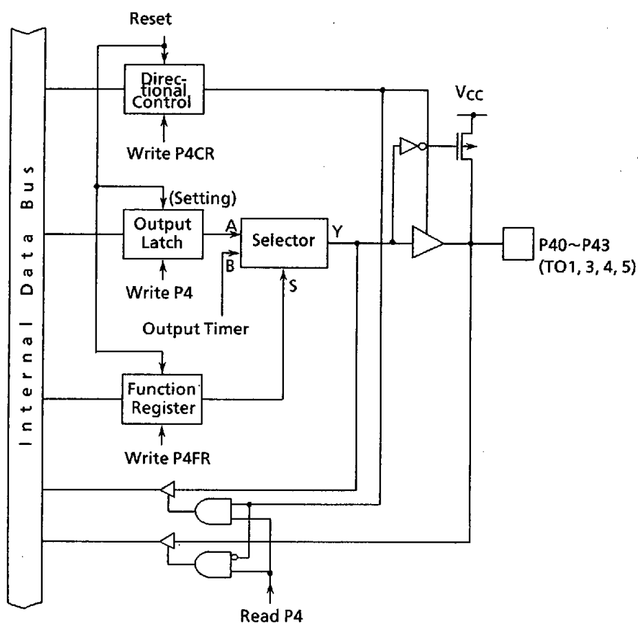
Figure 3.5 (7) Port 4 (P40~P43)
