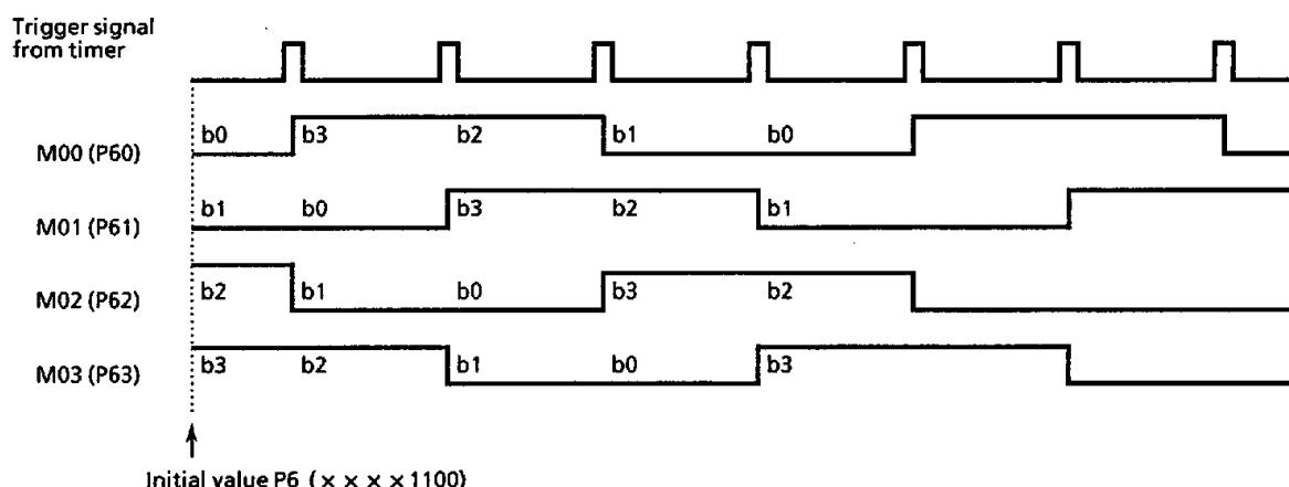
Figure 3.10 (7) Output Waveforms of 4-Phase 2-step Excitation (Normal Rotation)
