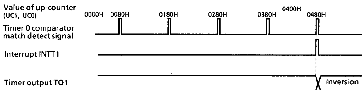
Figure 3.8 (11)
