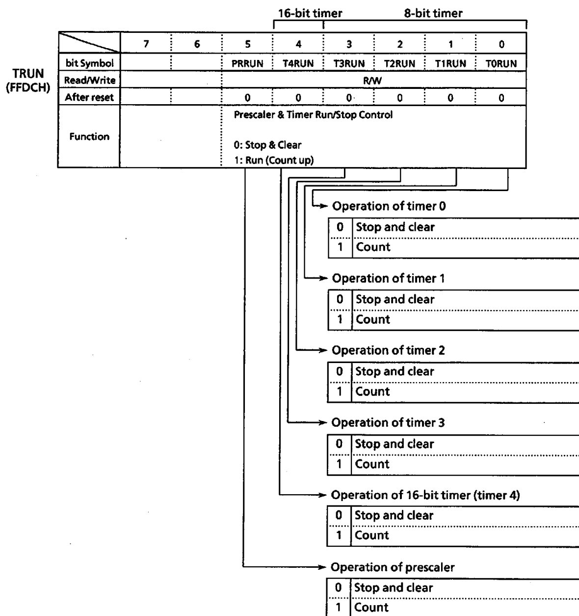
Figure 3.8 (7) Timer Operation Control Register (TRUN)
