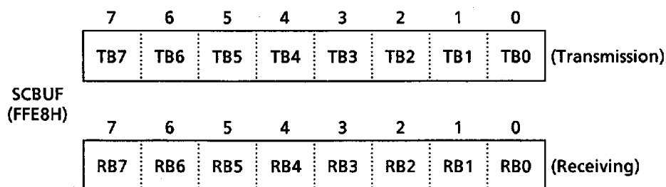
Figure 3.11 (4) Serial Transmission/Receiving Buffer Registers (SCBUF)
