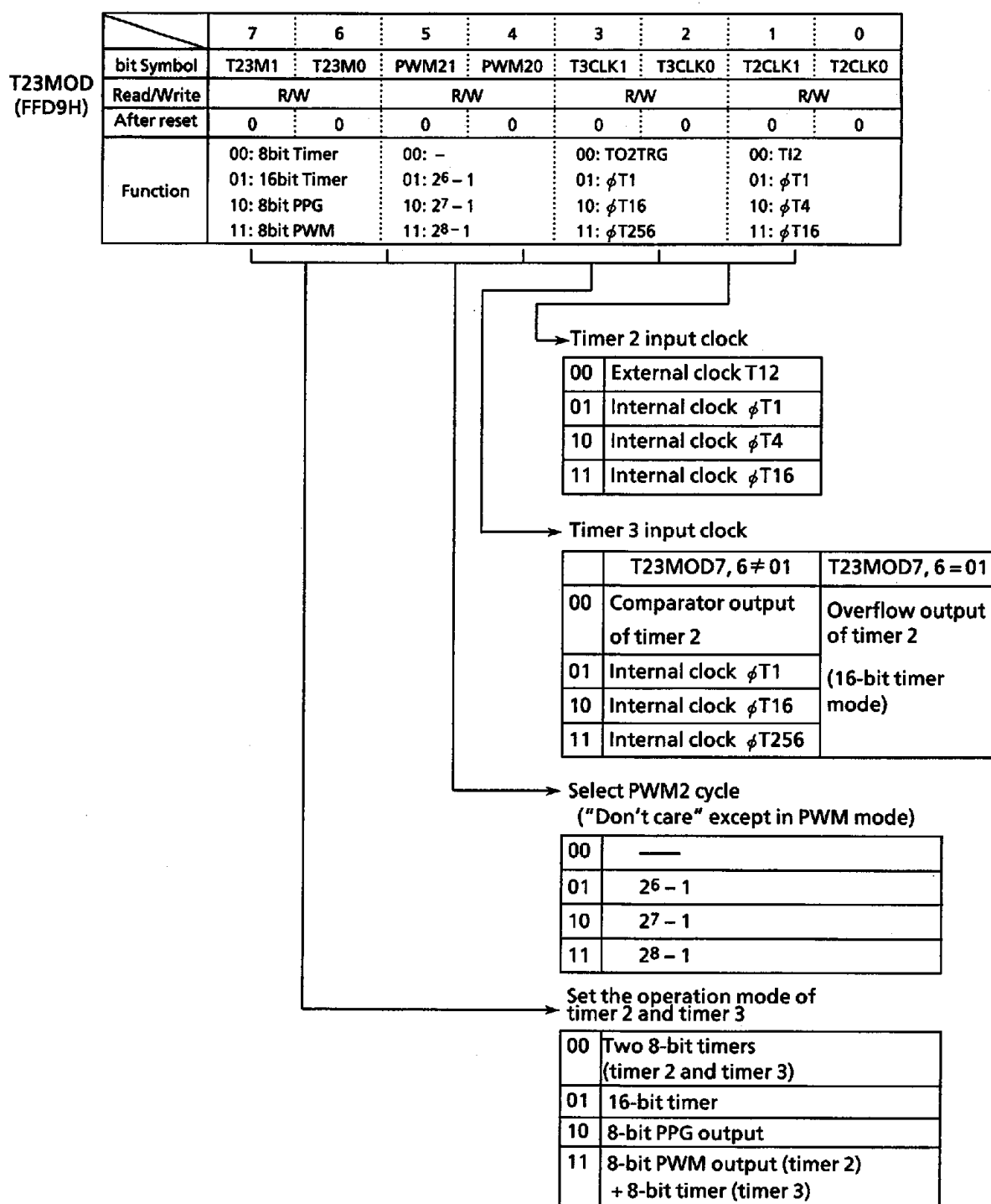
Figure 3.8 (5) Timer 2/Timer 3 Mode Register (T23MOD)
