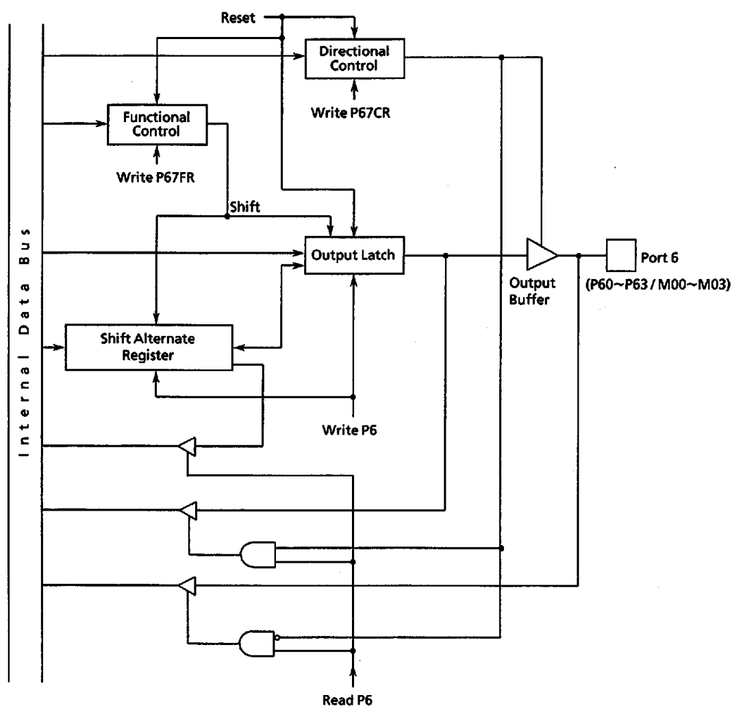
Figure 3.5 (14) Port 6
