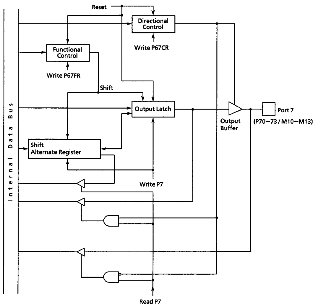
Figure 3.5 (15) Port 7
