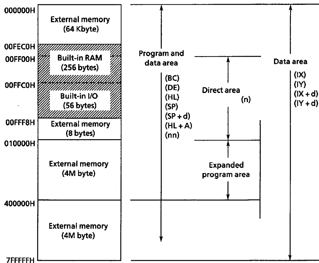
Figure 3.2 Memory Map
