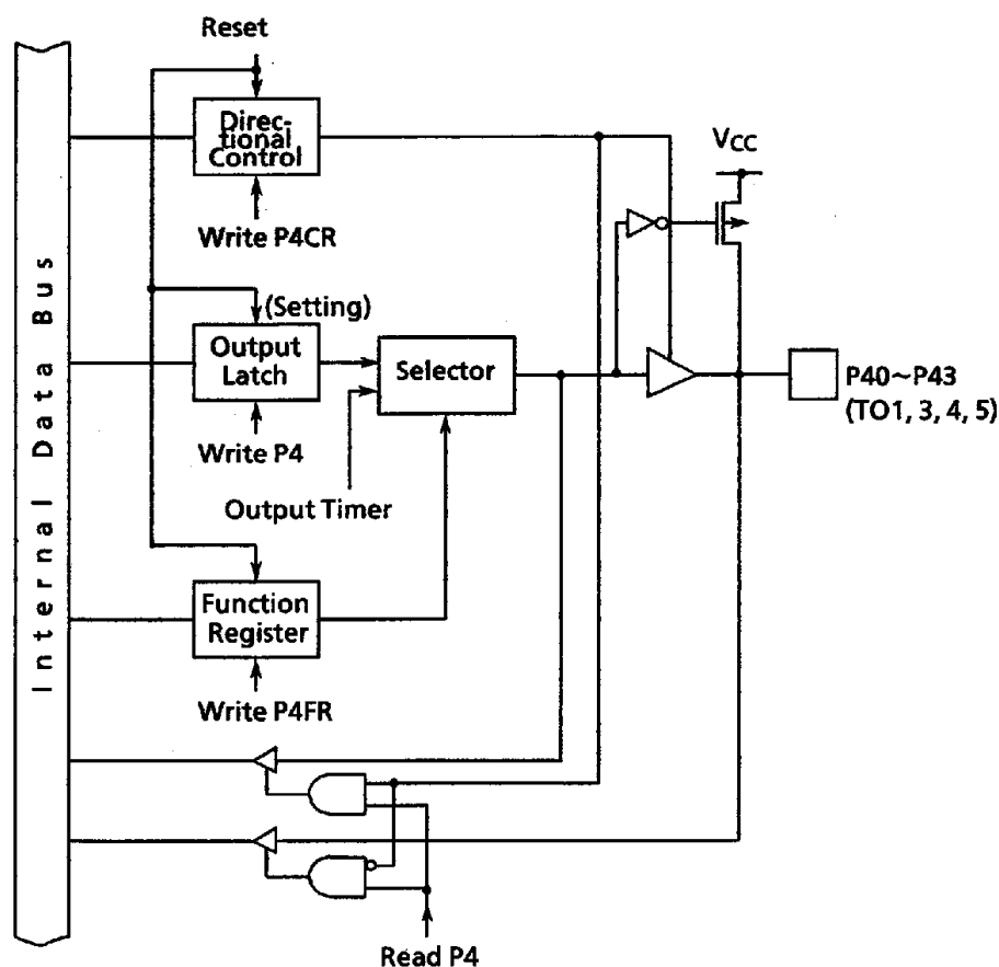
Figure 3.5 (7) Port 4 (P40~P43)
