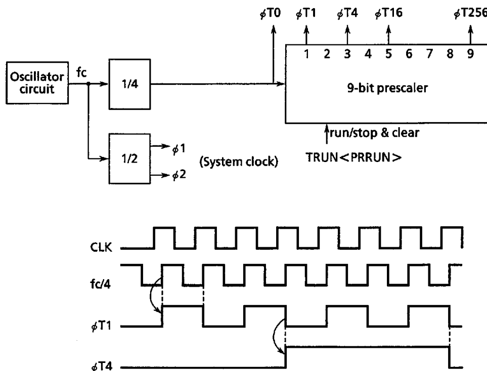
Figure 3.8 (2) Prescaler
