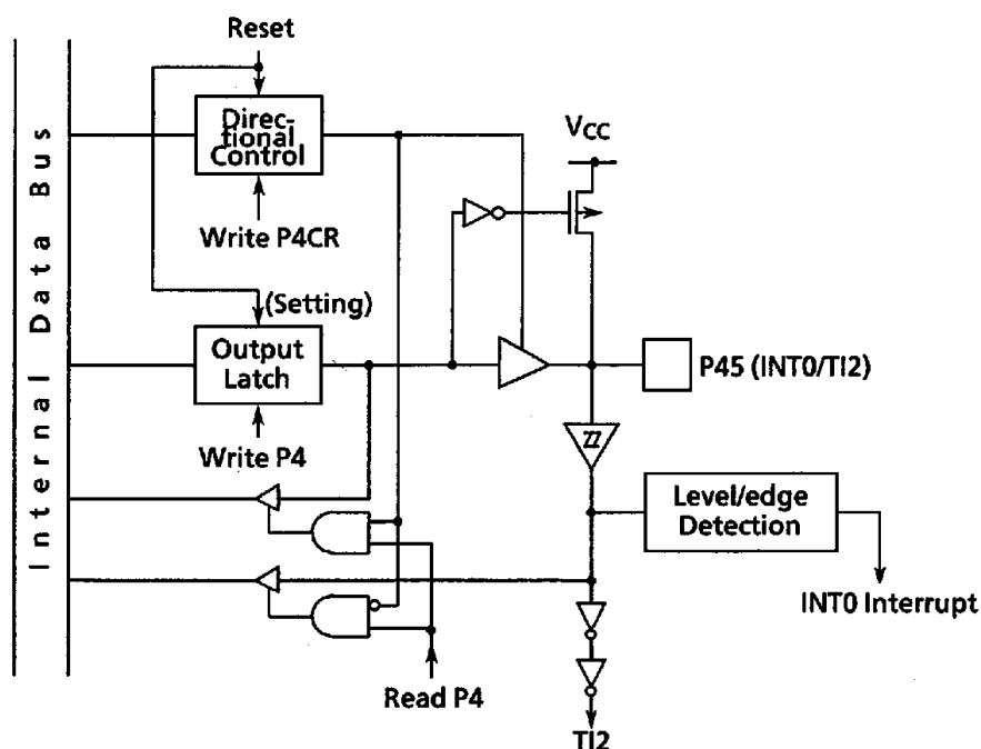
Figure 3.5 (9) Port 4 (P45)
