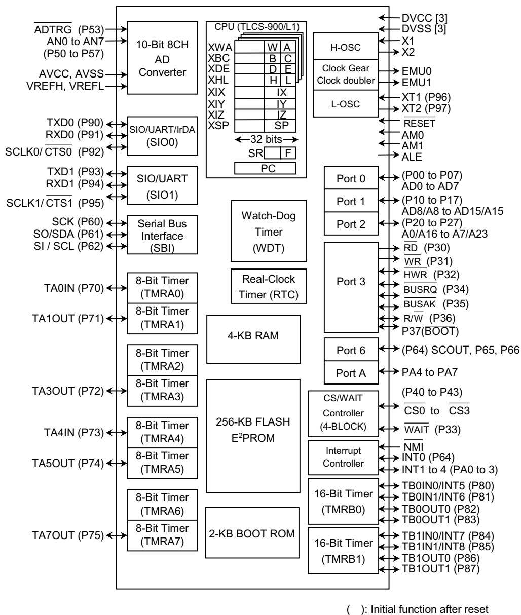
Figure 1.1 TMP91FY12AF Block Diagram
