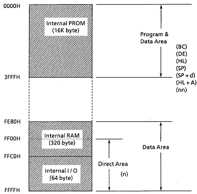
Figure 3.1 Memory Map
