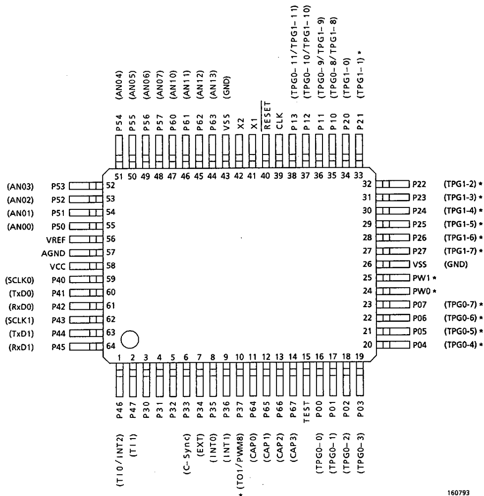
Figure 2.1 (2) Pin Assignment (Flat package)
