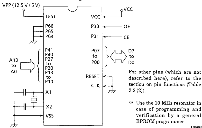
Figure 3.2 PROM Mode Pin Setting
