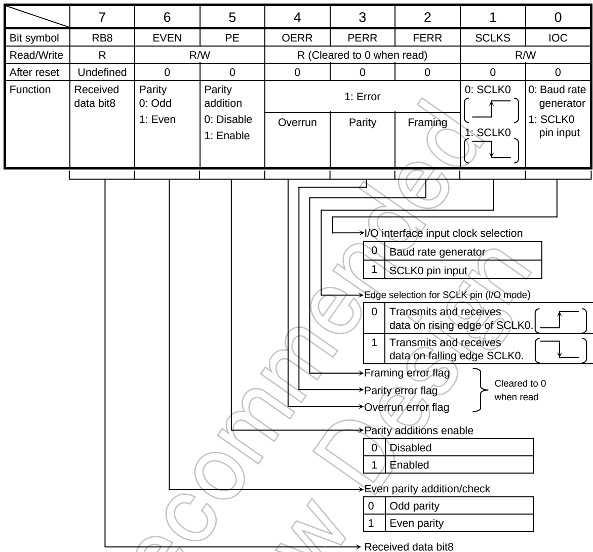
Figure 3.9.7 Serial Control Register (Channel 0, SC0CR)
