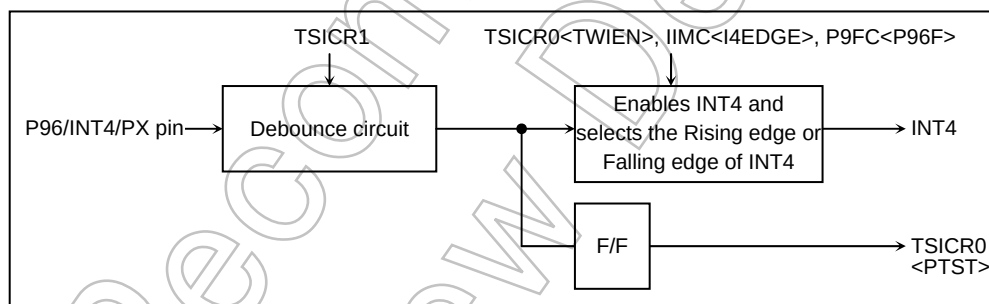
Figure 3.20.3 Block Diagram of Debounce Circuit
