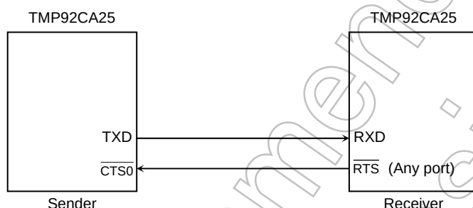
Figure 3.9.4 Handshake Function
