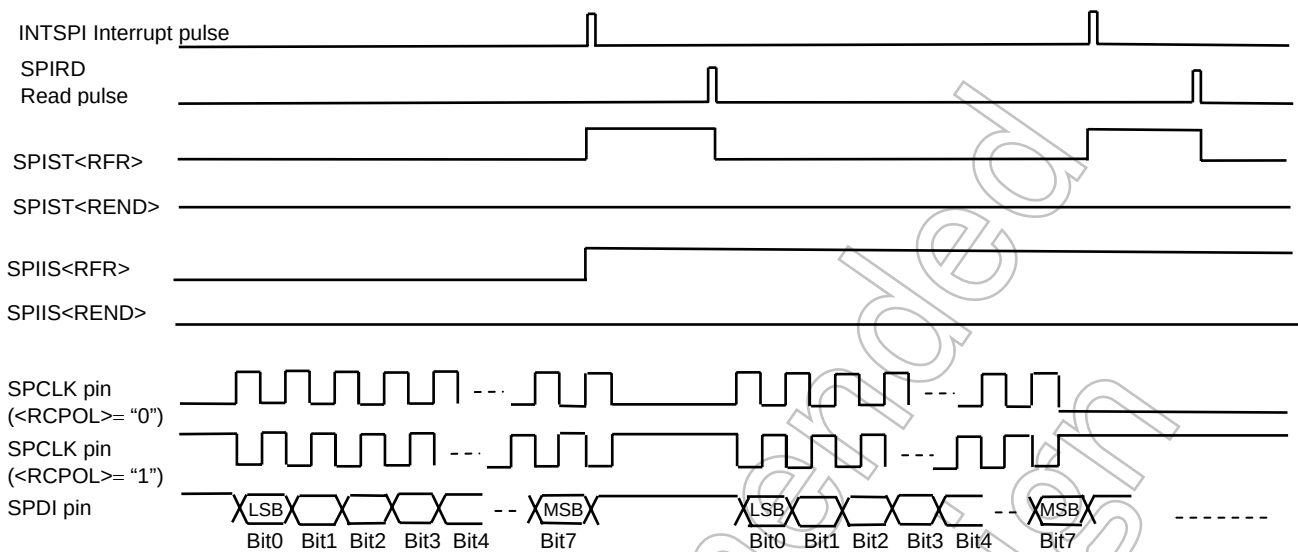
Figure 3.11.27 Micro DMA transmission (UNIT receiving (SPICT<REUEN>=1))
