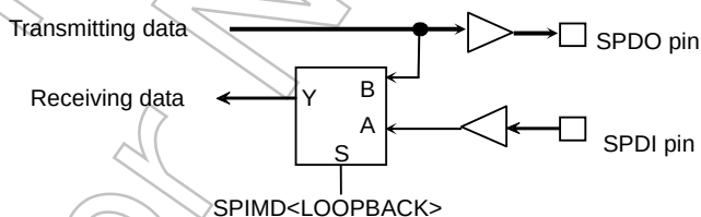
Figure 3.11.3 &lt;LOOPBACK&gt; Register Function
