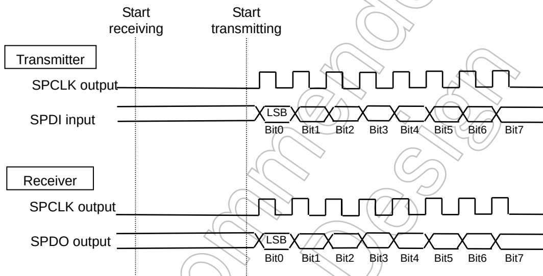
Figure 3.11.11 Alignment transmit/receive
