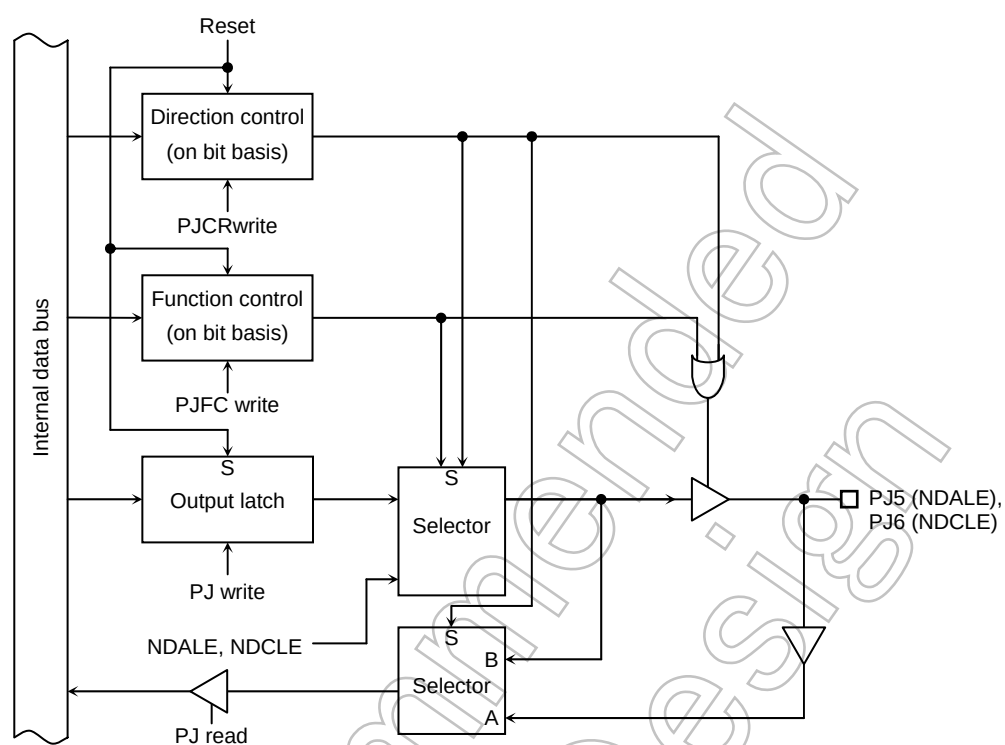
Figure 3.5.35 Port J5 and J6
