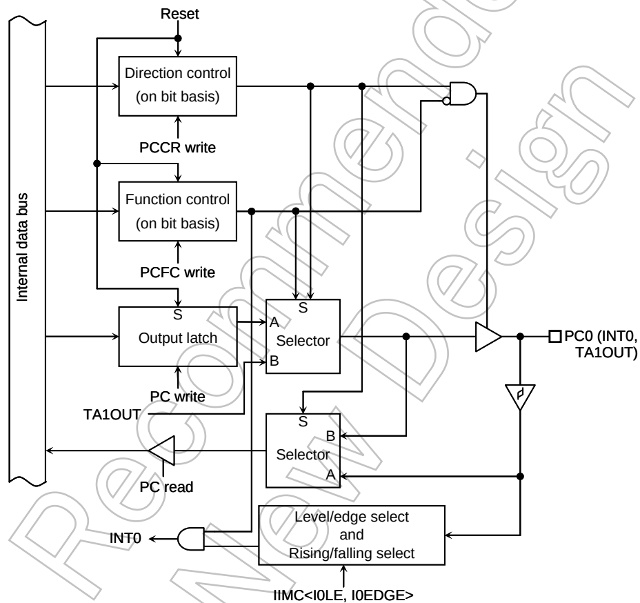
Figure 3.5.20 Port C0
