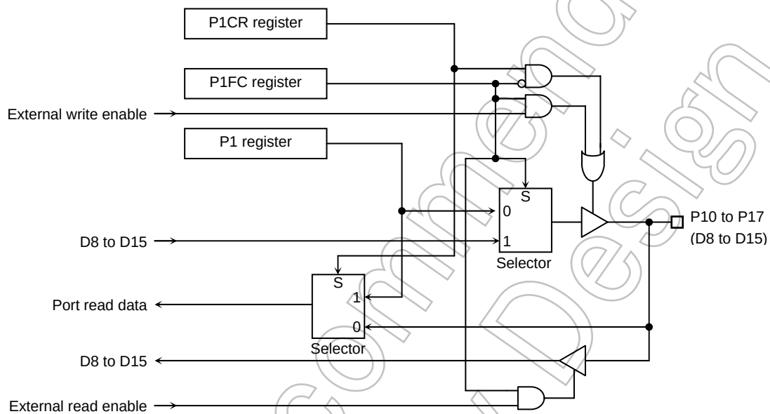
Figure 3.5.1 Port 1
