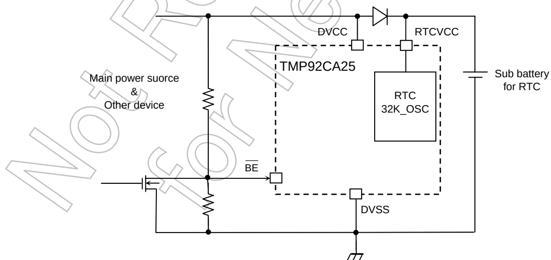
Figure 3.22.2 Outside circuit example for PSB
