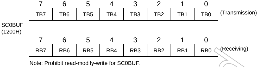
Figure 3.9.9 Serial Transmission/Receiving Buffer Registers (Channel 0, SC0BUF)
