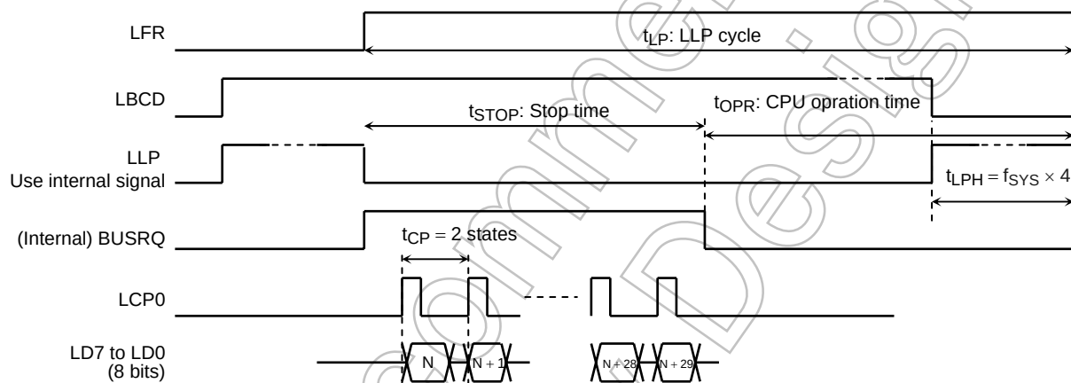
Figure 3.15.3 Whole Timing Diagram of SR Mode
