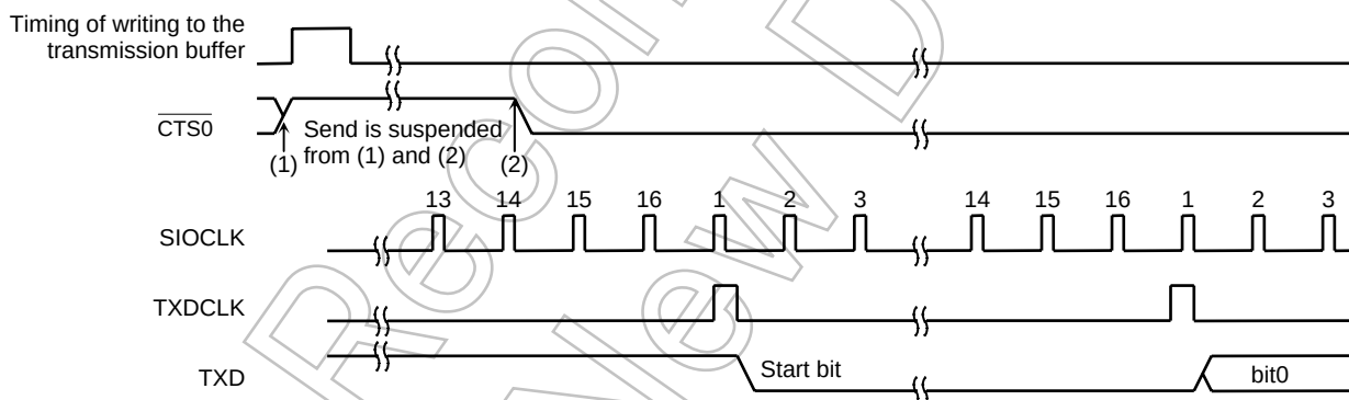
Figure 3.9.4 Handshake Function
