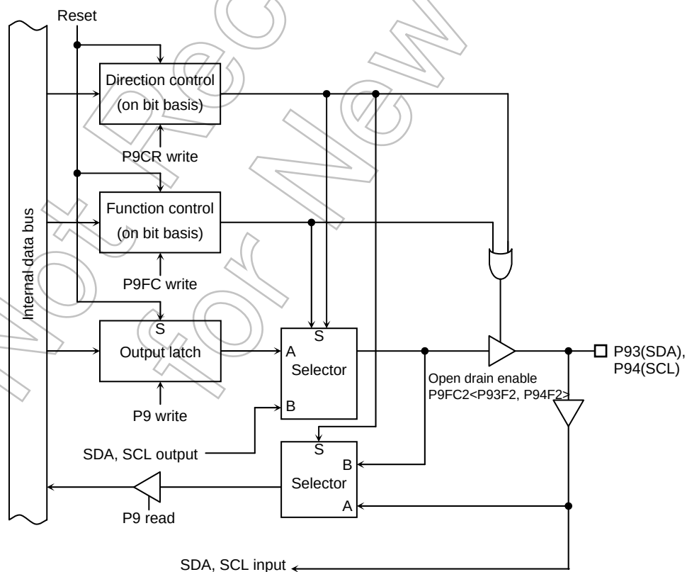
Figure 3.5.14 Port 93 and 94
