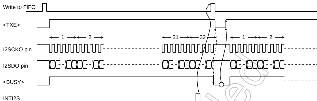
Figure 3.21.7 Whole Timing
