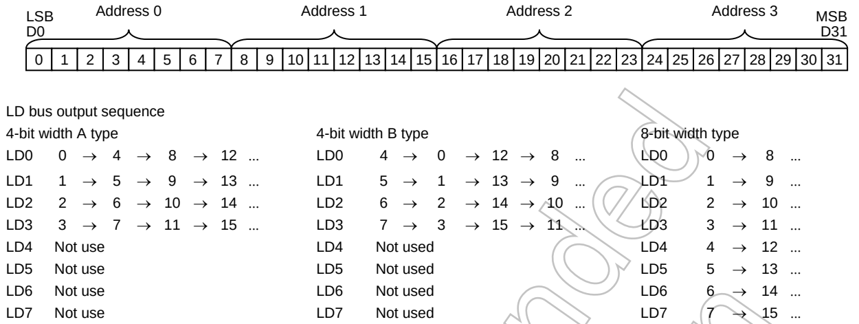
Figure 3.15.2 Relation of Memory Map Image and Output Data
