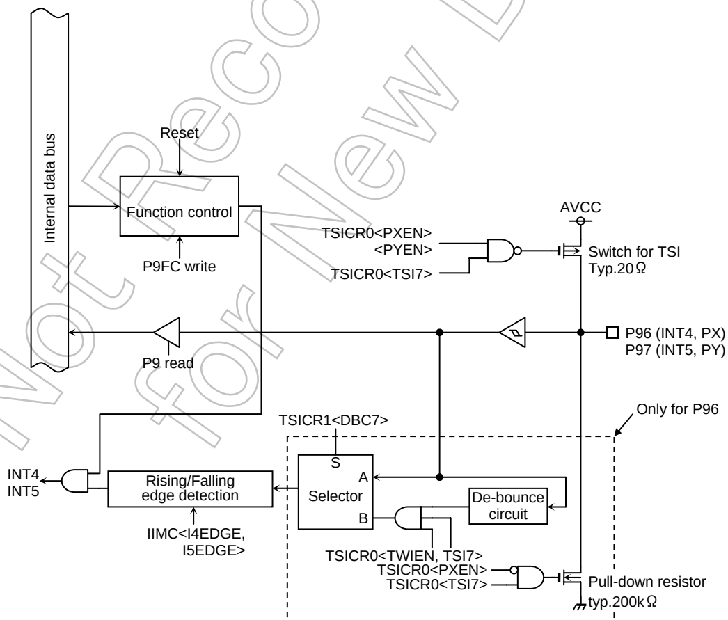
Figure 3.5.16 Port 96, 97
