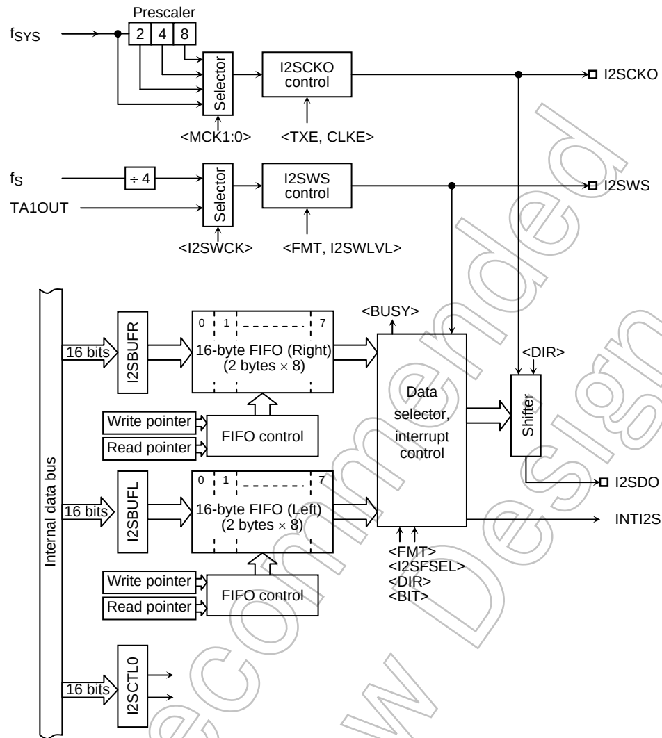
Figure 3.21.1 I²S Block Diagram
