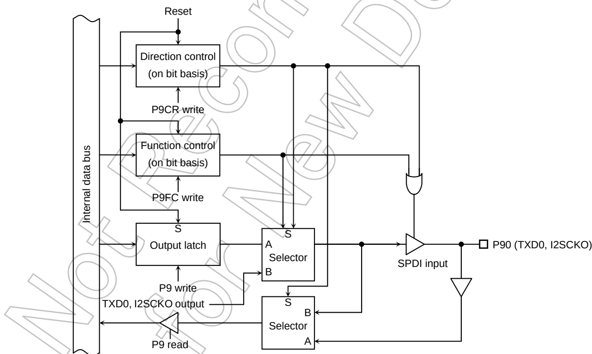
Figure 3.5.12 P90
