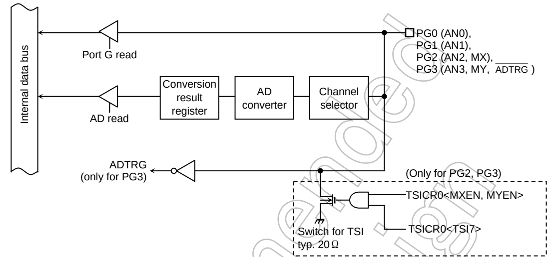
Figure 3.5.32 Port G
