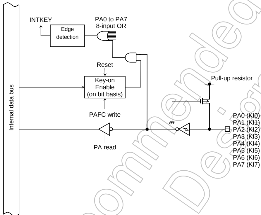
Figure 3.5.18 Port A
