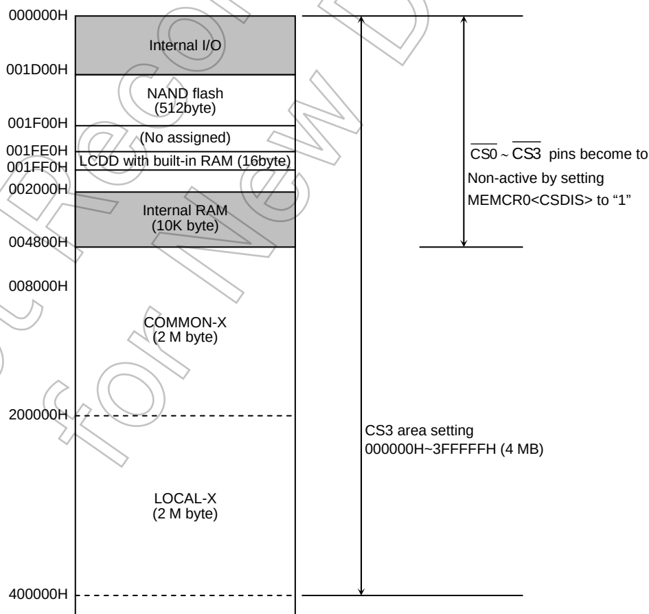
Figure 3.6.5 Recommended CS3 and CS0 Setting
