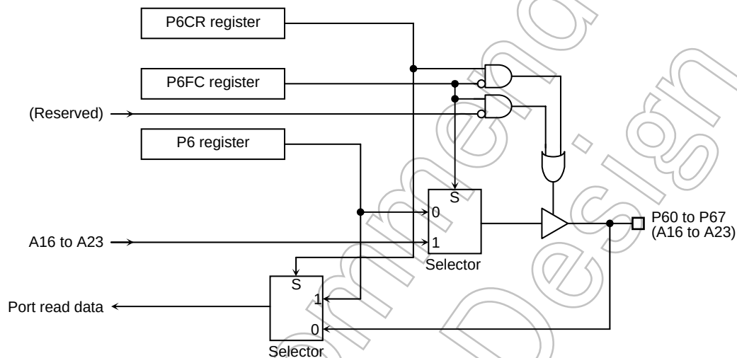
Figure 3.5.5 Port 6
