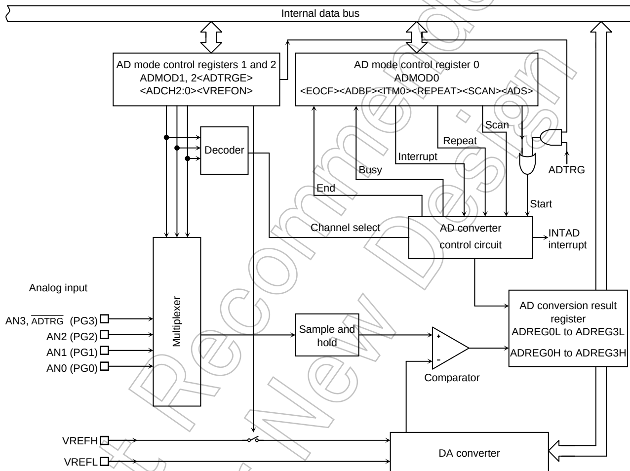
Figure 3.12.1 Block Diagram of AD Converter
