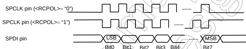
Figure 3.11.5 <TCPOL> Register function
