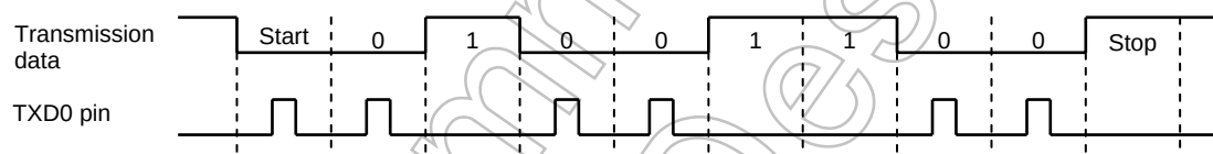
Figure 3.9.19 Transmission Example
