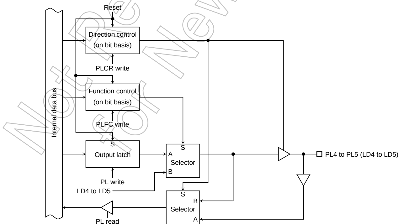
Figure 3.5.42 Register for Port L4 to L5
