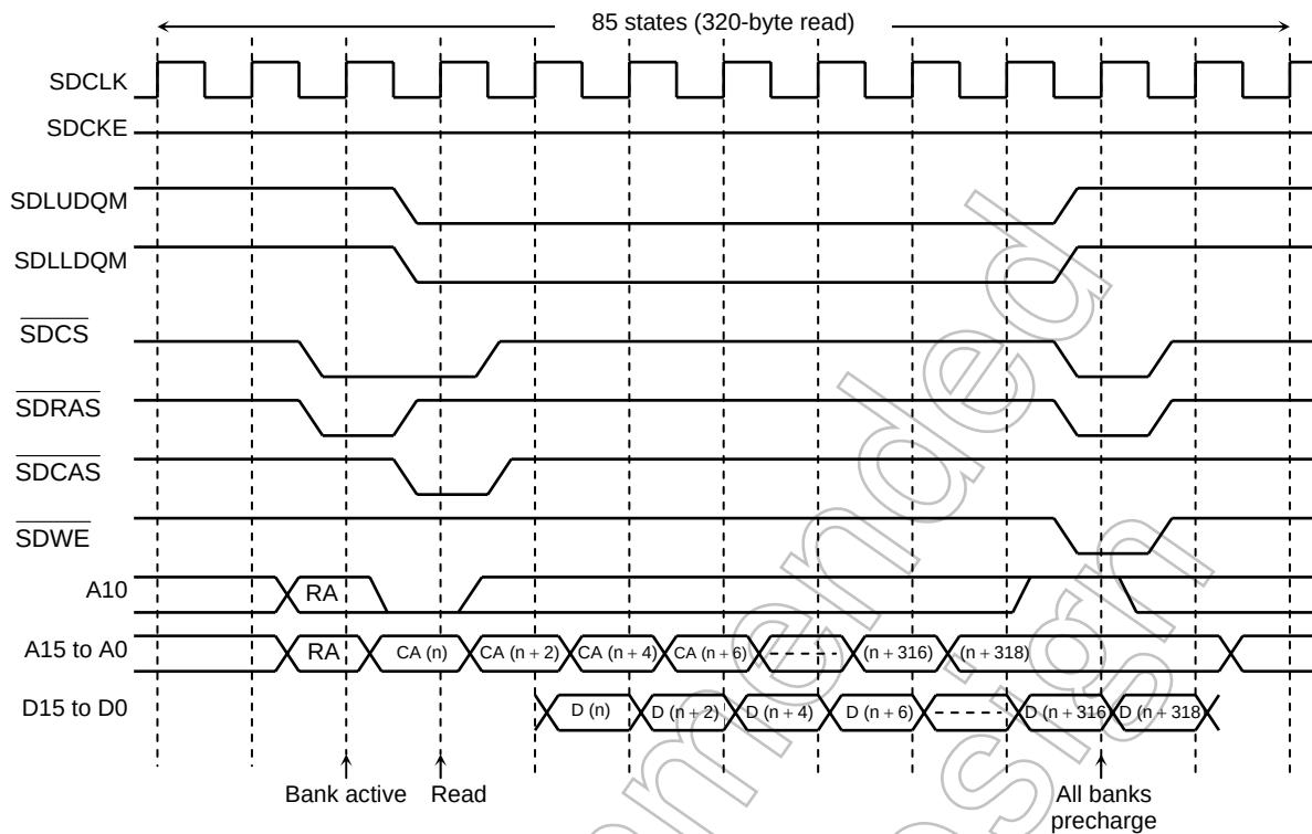
Figure 3.17.2 Timing of Burst Read Cycle
