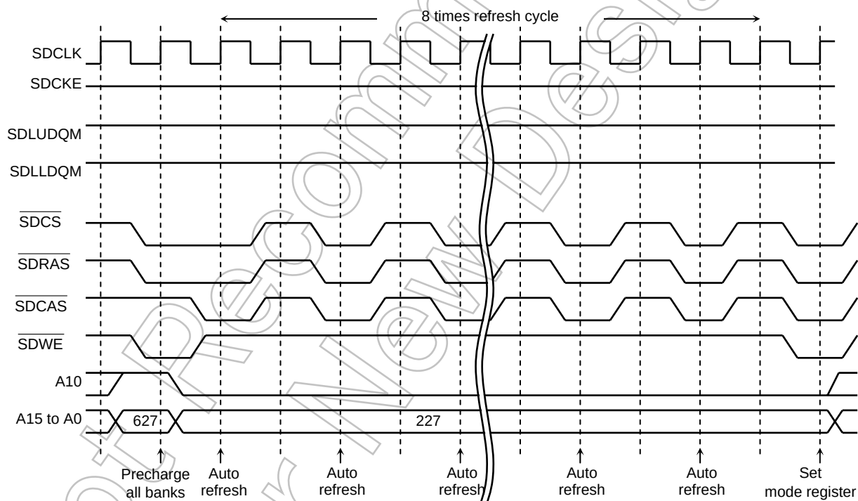
Figure 3.17.7 Timing of Initialization command
