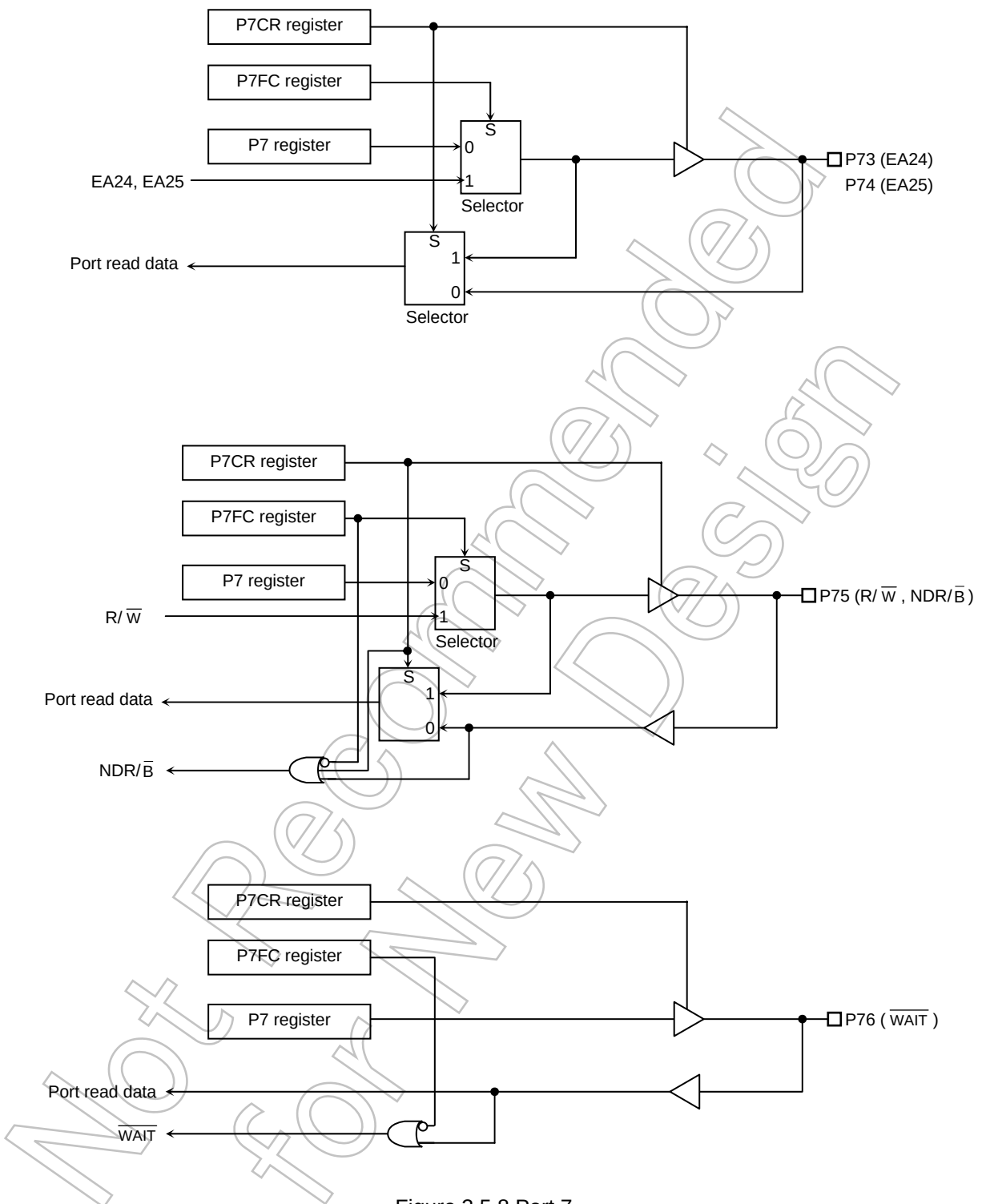
Figure 3.5.8 Port 7
