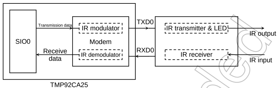
Figure 3.9.18 Block Diagram
