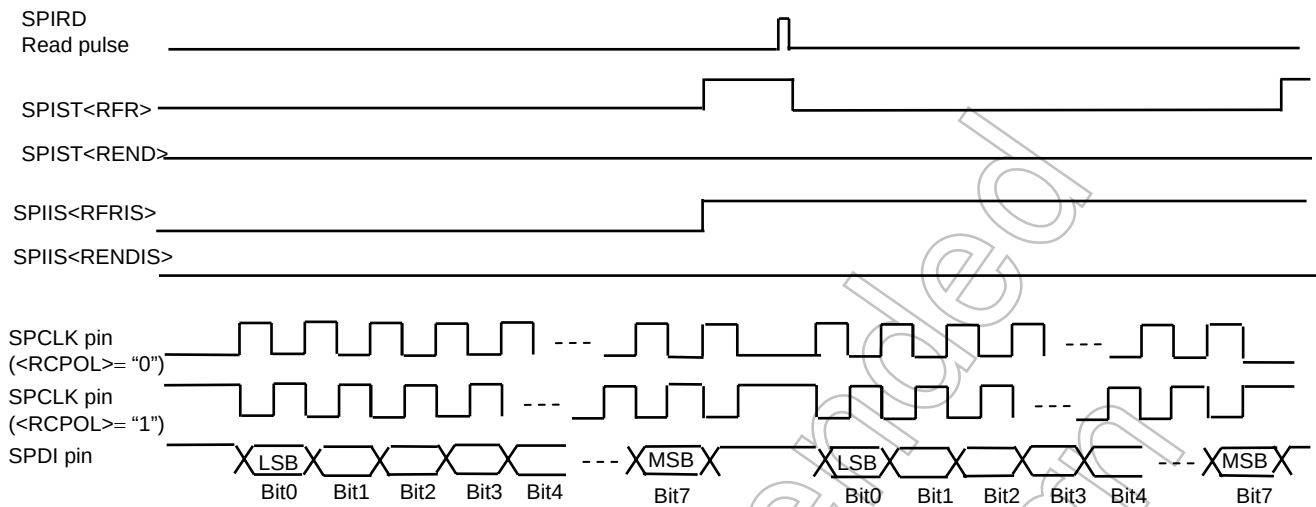
Figure 3.11.24 UNIT receiving ( \text{SPICT}\langle\text{RXUEN}\rangle = 1 )
