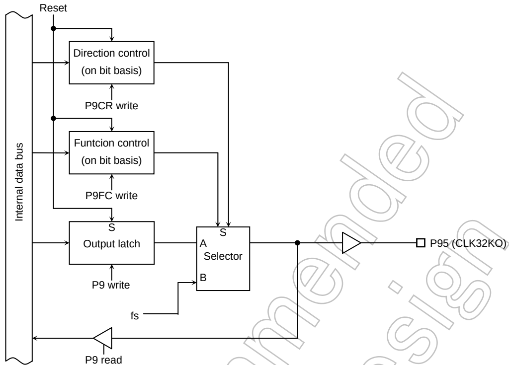
Figure 3.5.15 Port 95
