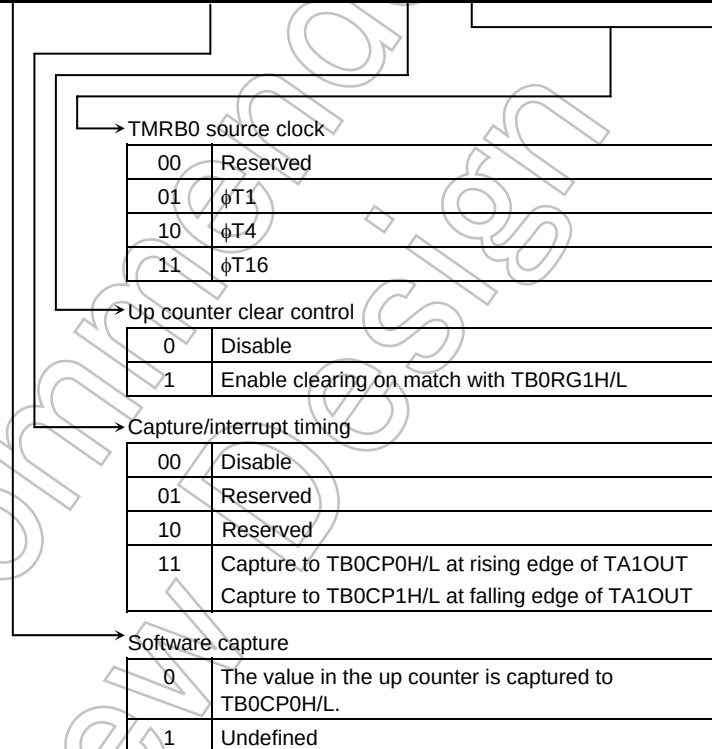
Figure 3.19.3 The Registers for TMRB0
