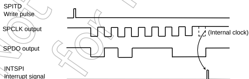
Figure 3.11.28 Example of UNIT transmission
