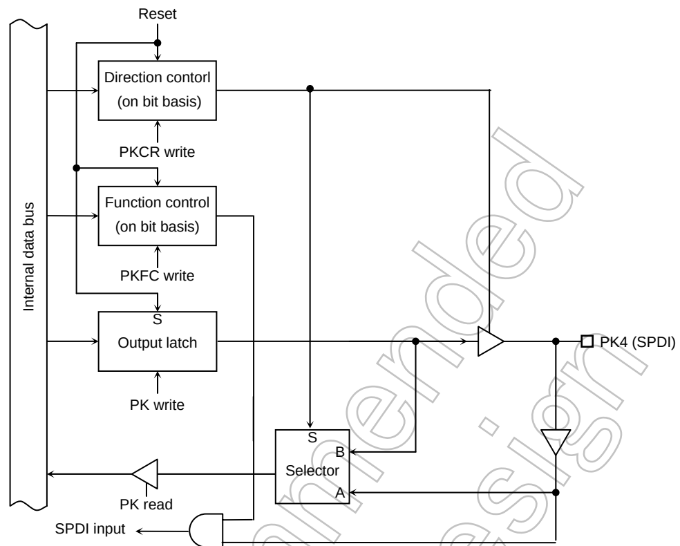
Figure 3.5.38 Port K4
