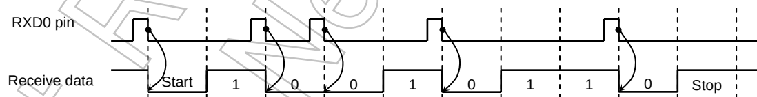
Figure 3.9.20 Receiving Example
