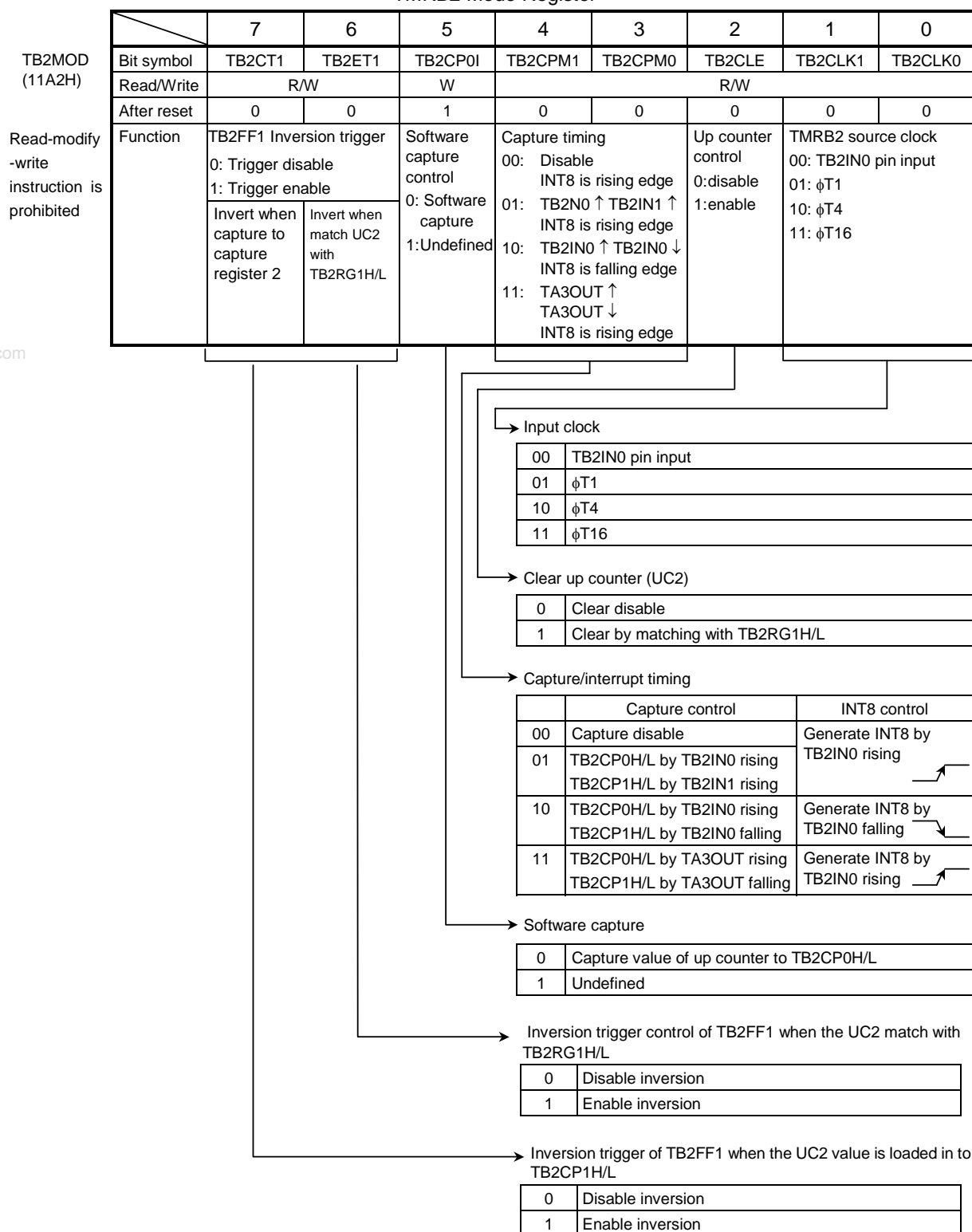
TMRB2 Mode Register
