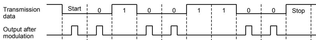
Figure 3.10.37 Example of Modulation of Transmission Data (SIO0)
