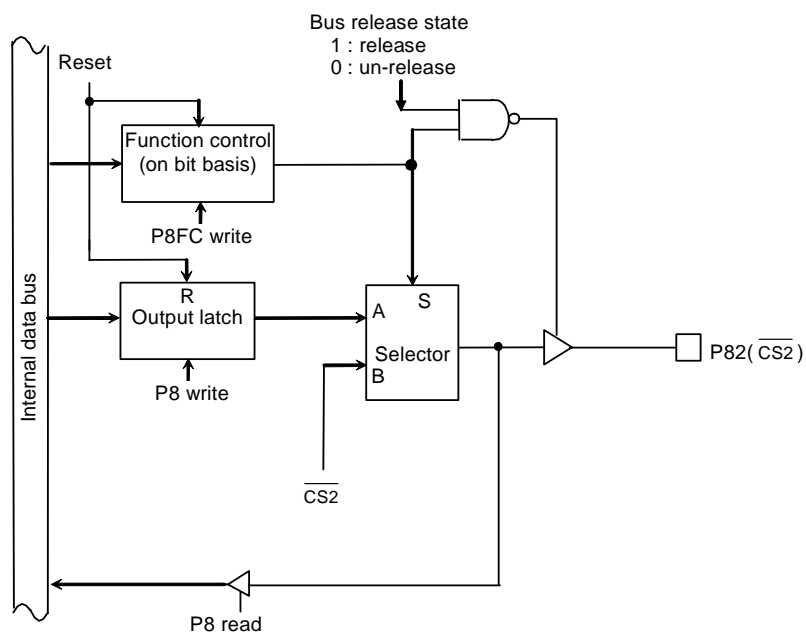
Figure 3.5.10 Port 8(P82)
