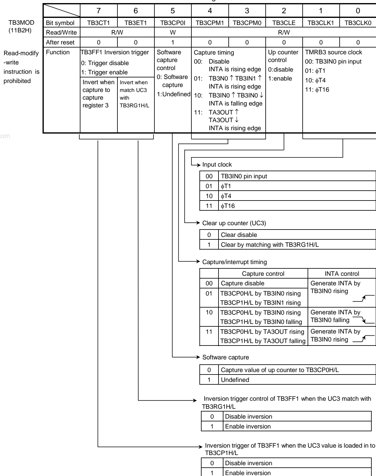
TMRB3 Mode Register
