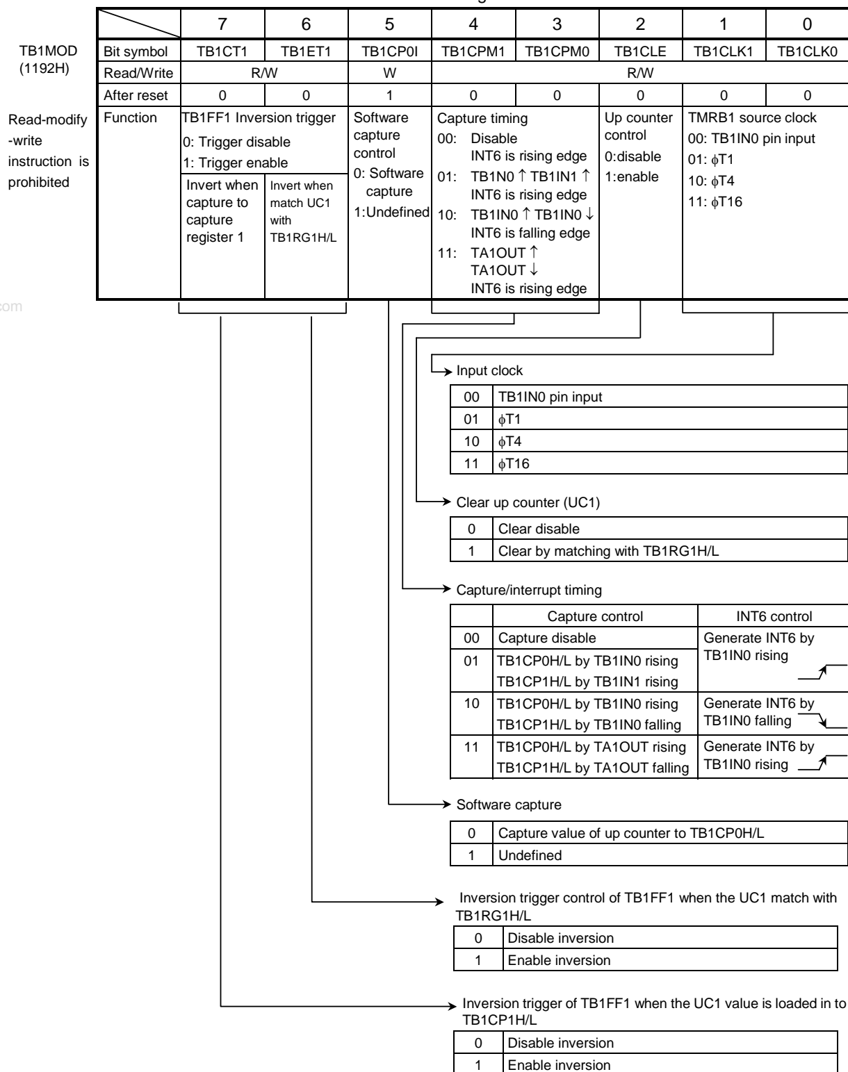
TMRB1 Mode Register
