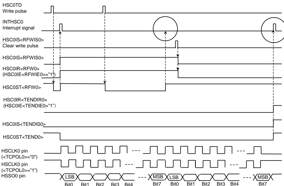
Figure 3.12.36 Transmission timing
