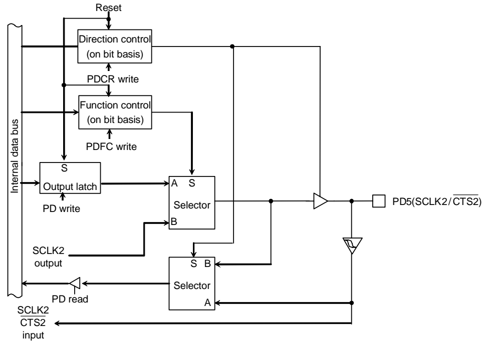
Figure 3.5.30 Port D(PD5)
