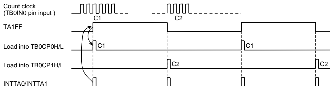
Figure 3.8.33 Frequency Measurement
