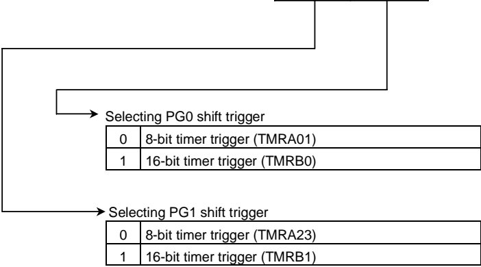
Figure 3.9.6 Pattern Generation Control Register 2 (PG01CR2)
