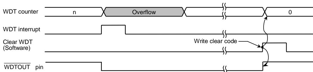
Figure 3.16.2 Normal Mode
