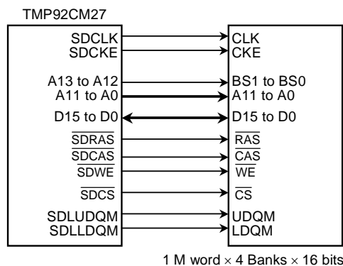
Figure 3.13.8 Connection with SDRAM (4 M word × 16 bits)
