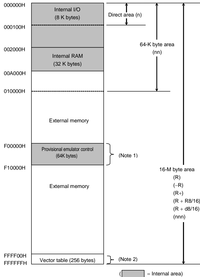
Figure 3.2.1 Memory Map
