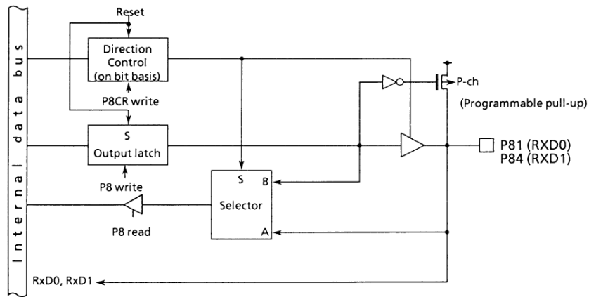
Figure 3.5 (13). Port 81, 84
