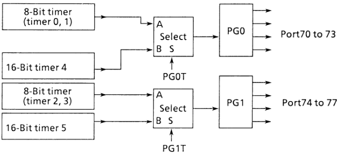
Figure 3.10 (6). Connection of Timer and Pattern Generator
