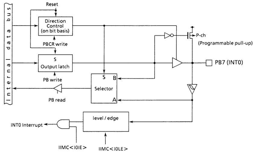
Figure 3.5 (22). Port B7
