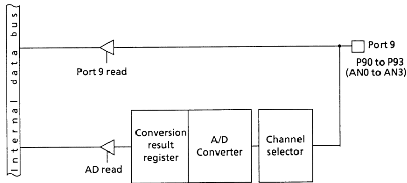
Figure 3.5 (17). Port 9
