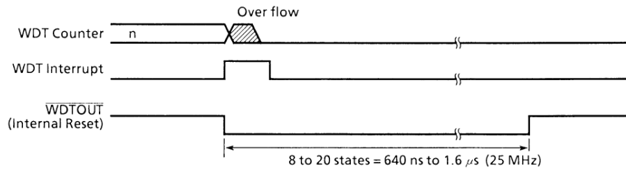
Figure 3.13 (3). Reset Mode
