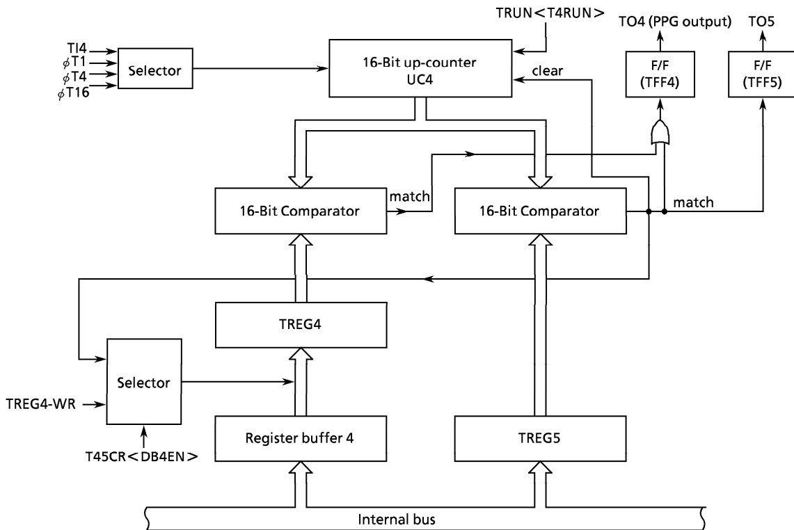
Figure 3.8 (9) Block Diagram of 16-Bit PPG Mode
