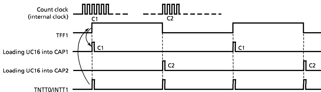
Figure 3.8 (12) Frequency Measurement
