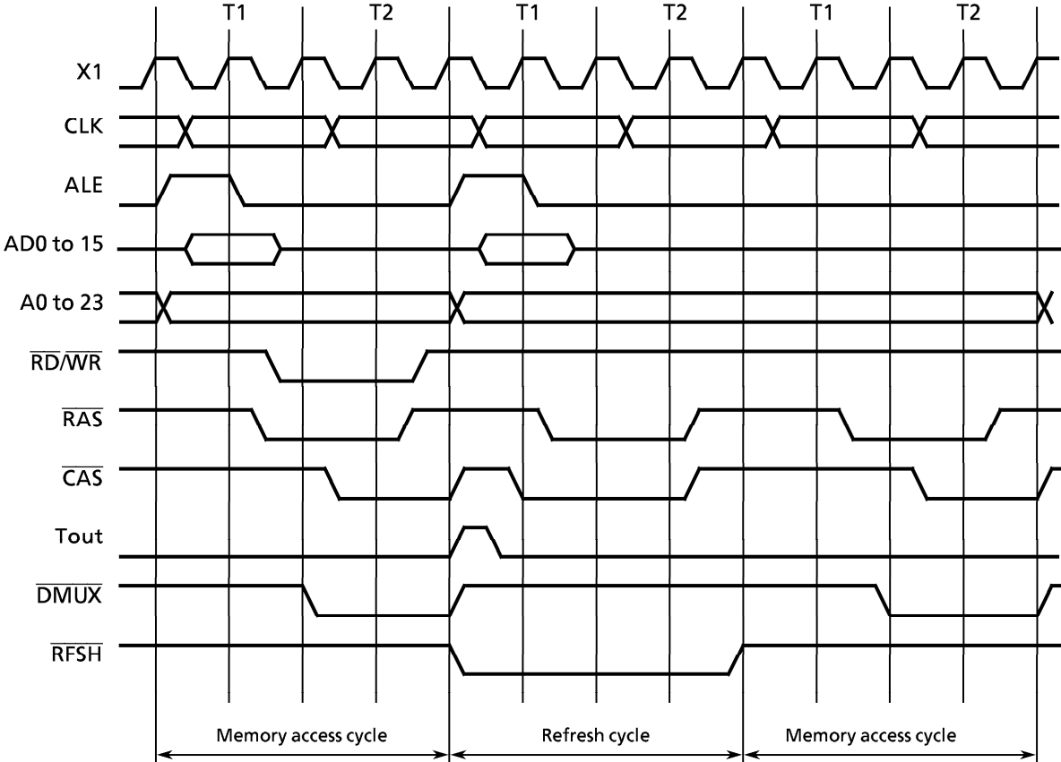
Figure 3.13 (10) Timing Diagram when Refresh Cycle is Inserted in Memory Access Cycle
