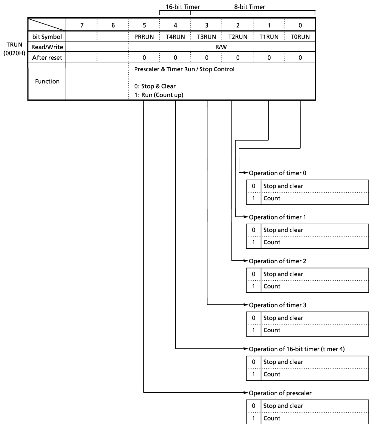
Figure 3.7 (7) Timer Operation Control Register (TRUN)
