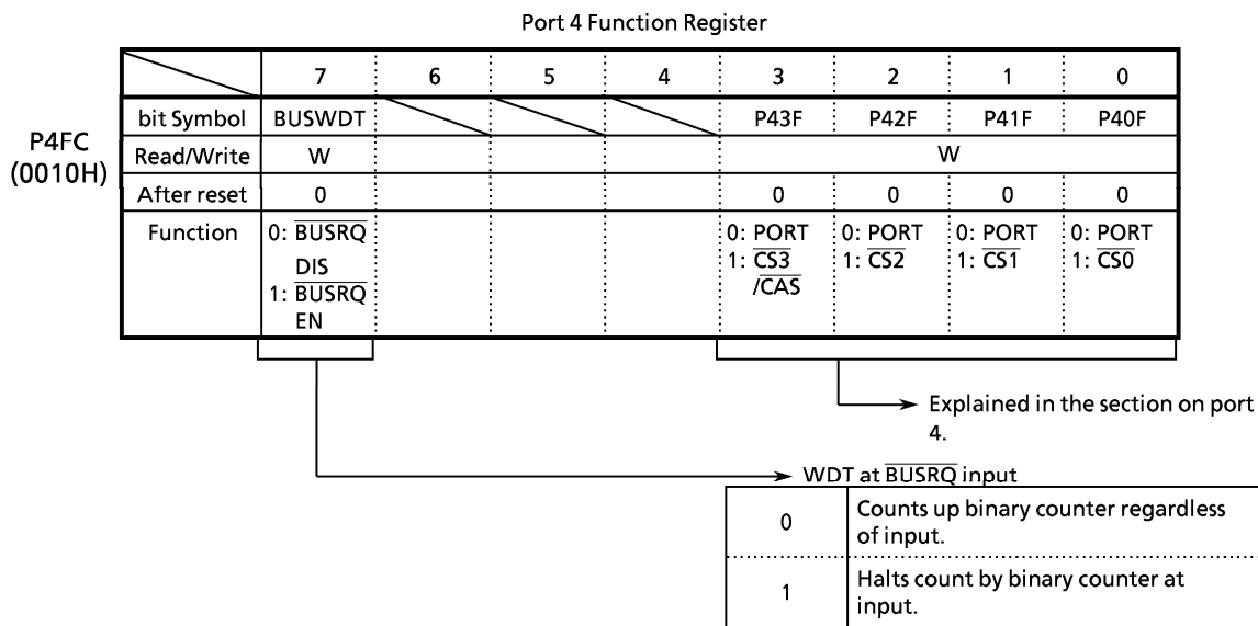
Figure 3.12 (6)
