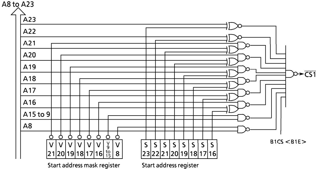
Figure 3.6 (4) CS1 Address Decode Block Diagram
