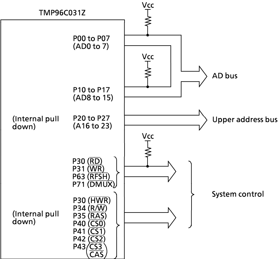
Figure 3.5 (1) External bus interface example when bus release function is in use
