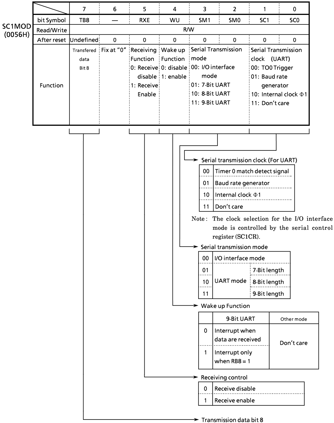
Figure 3.10 (6) Serial Mode Control Register (Channel 1, SC1MOD)
