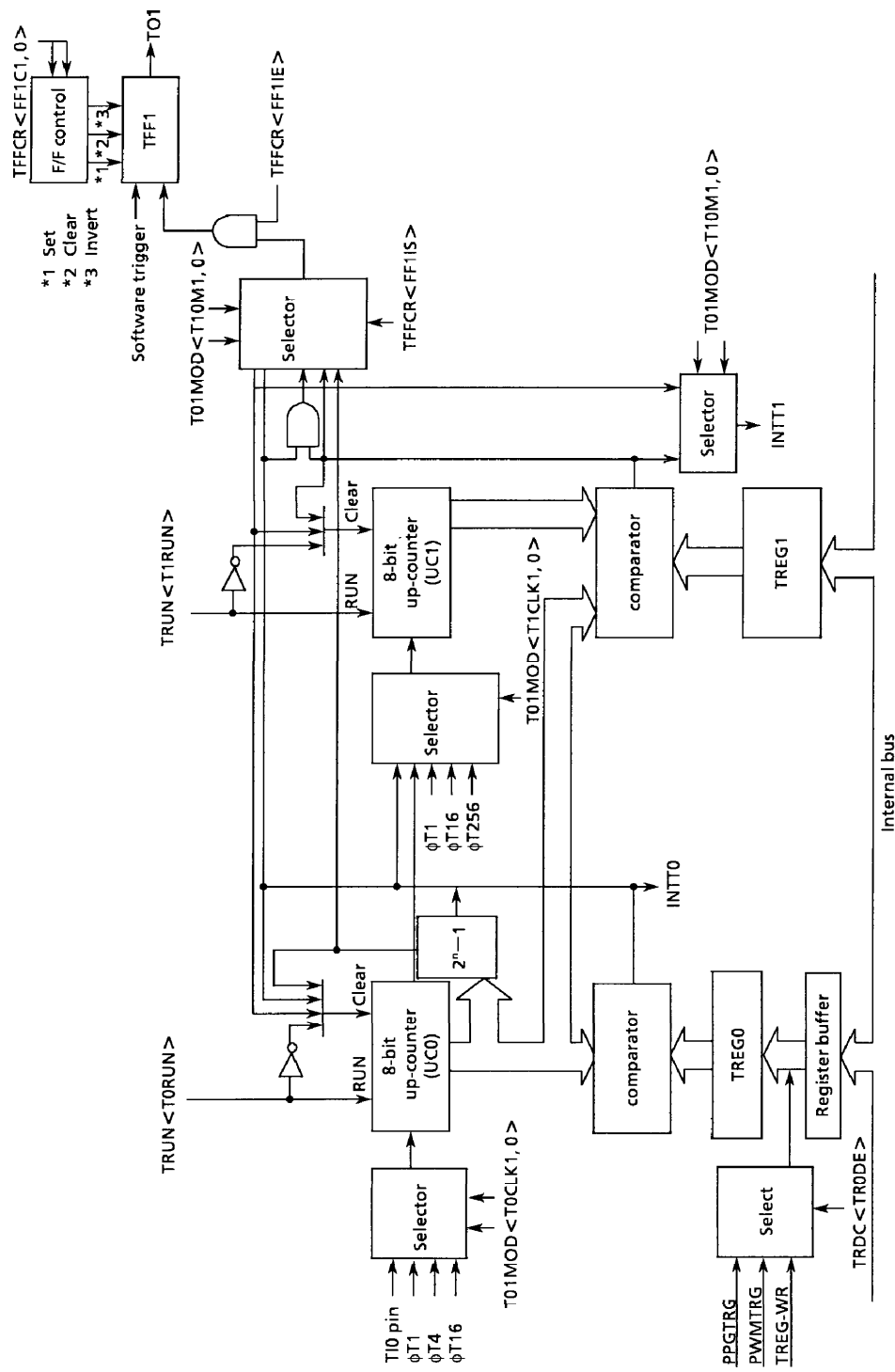
Figure 3.7 (1) Block Diagram of 8-bit Timers (Timers 0 and 1)
