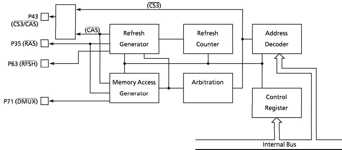
Figure 3.13 (1) DRAM Controller Block Diagram
