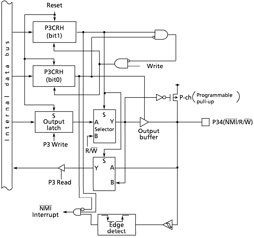
Figure 3.5 (7) Port 3 (P34)
