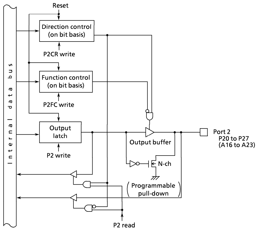
Figure 3.5 (2) Port 2
