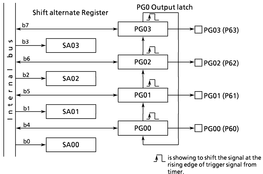
Figure 3.9 (10) Block Diagram of 4-Phase 1-step Excitation/2-step Excitation (Normal Rotation)
