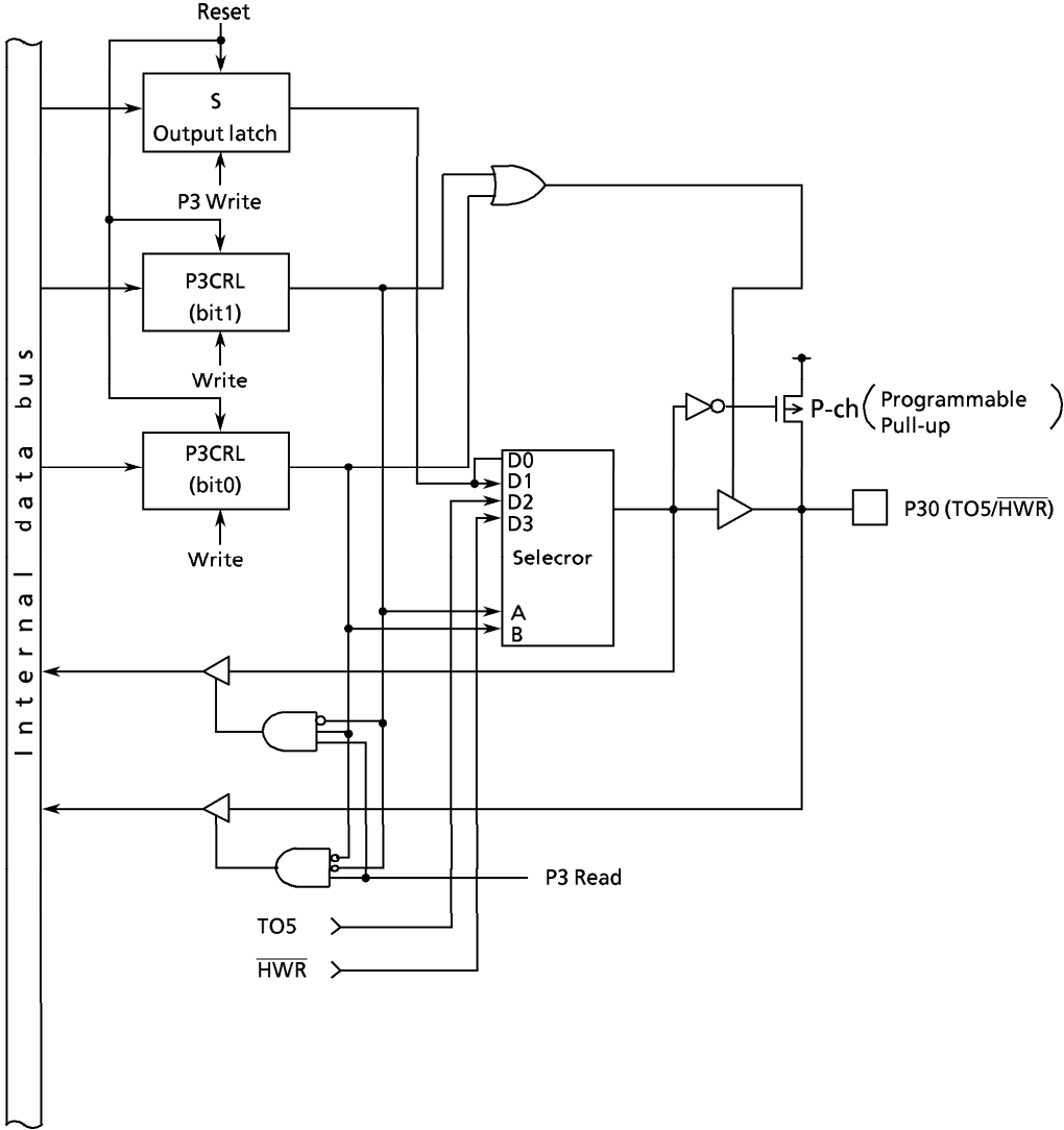
Figure 3.5 (4) Port 3 (P30)
