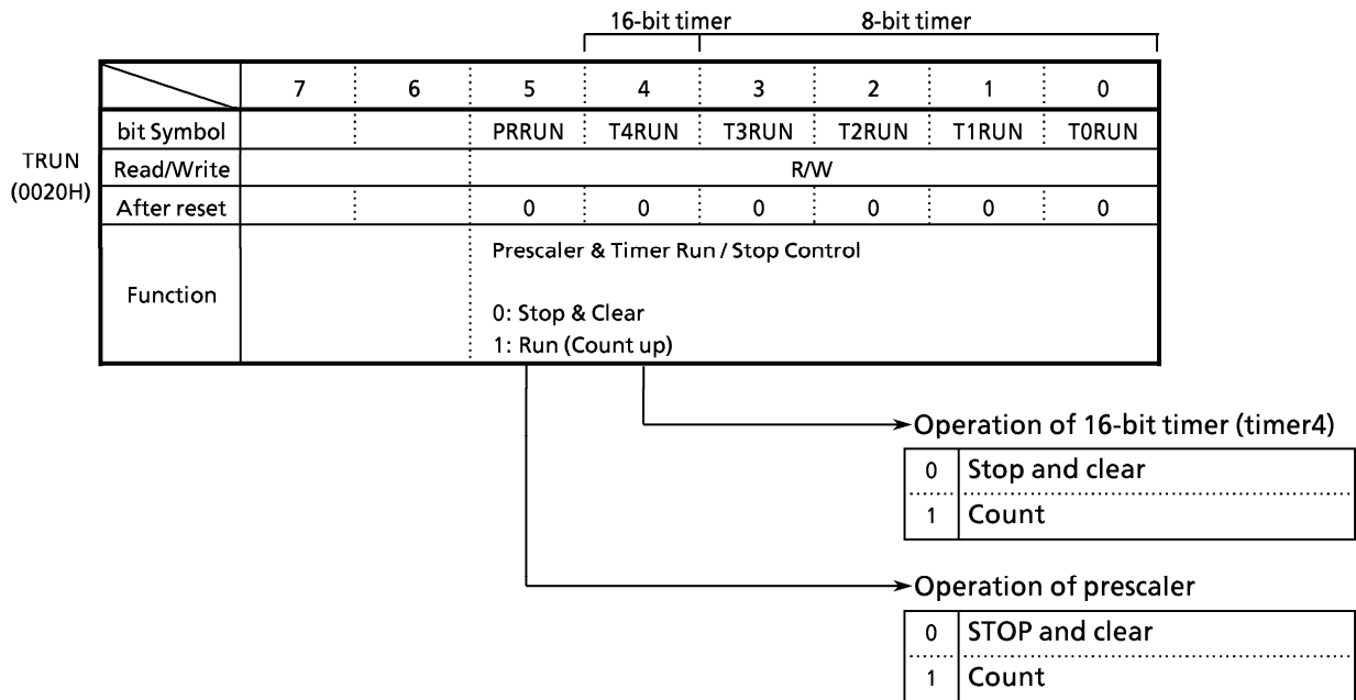
Figure 3.8 (6) Timer Operation Control Register (TRUN)
