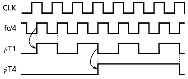
Figure 3.7 (2) Prescaler
