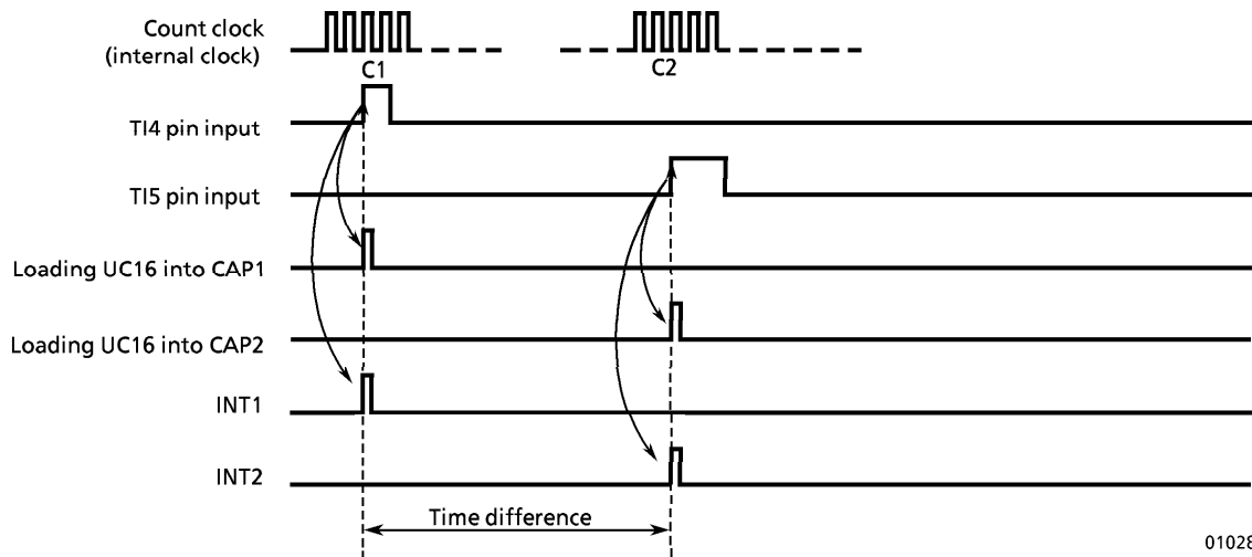
Figure 3.8 (14) Time Difference Measurement
