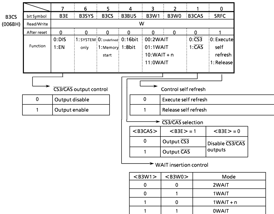
Figure 3.13 (2) Chip Select Wait Control Register (B3CS)
