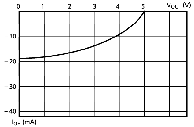
Figure 4.5 V_{OUT} - I_{OH} TYPICAL CURVE
