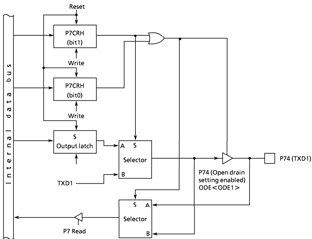
Figure 3.5 (19) Port 7 (P74)
