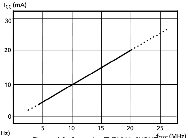
Figure 4.2 f_{OSC} - I_{CC} TYPICAL CURVE
