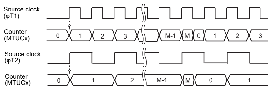
Figure 21-5 Count-up/clear operation when \phi T1 , \phi T2 or \phi T4 is selected as a source clock
