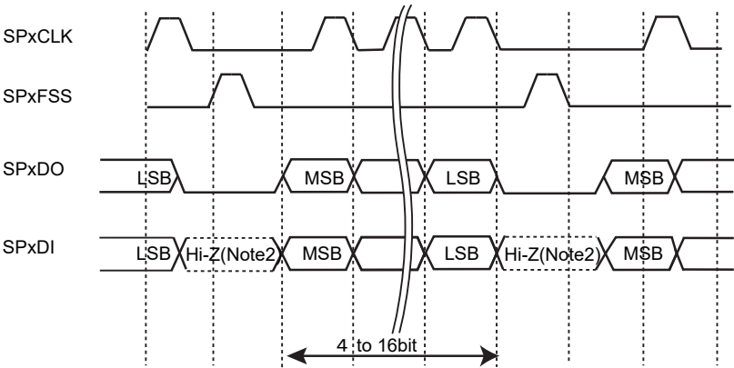
Figure 15-5 SPI frame format (continuous transfer, \langle \text{SPO} \rangle = "0" & \langle \text{SPH} \rangle = "0" )
