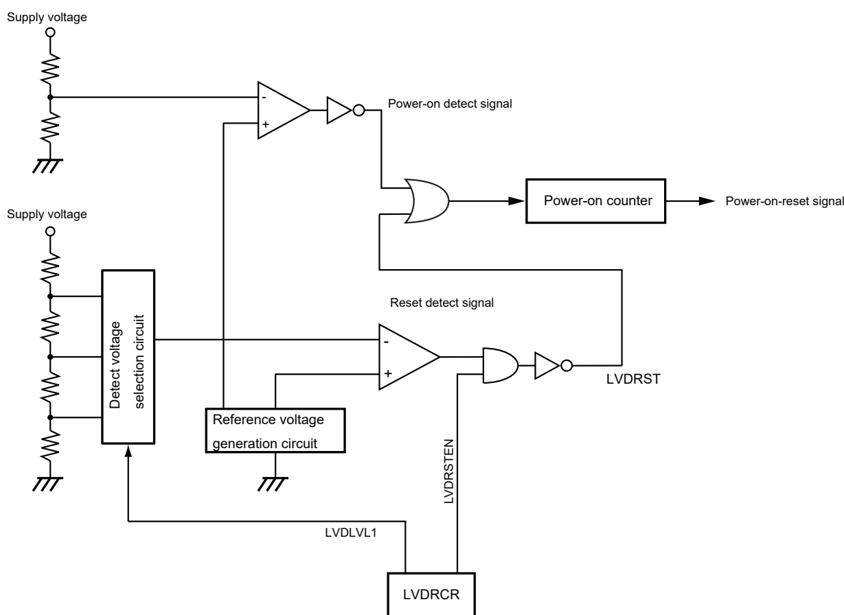
Figure 24-1 Power-on-reset circuit
