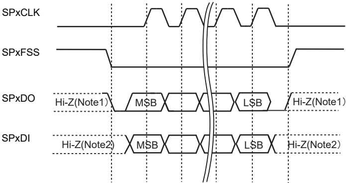
Figure 15-4 SPI frame format (single transfer, \langle \text{SPO} \rangle = "0" & \langle \text{SPH} \rangle = "0" )
