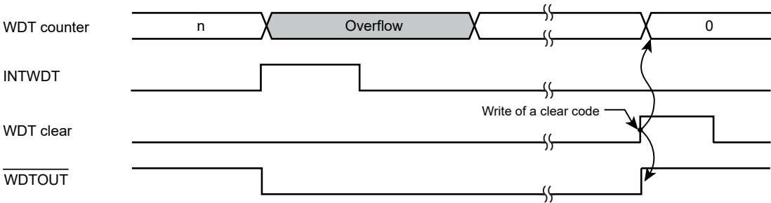
Figure 27-2 INTWDT interrupt generation
