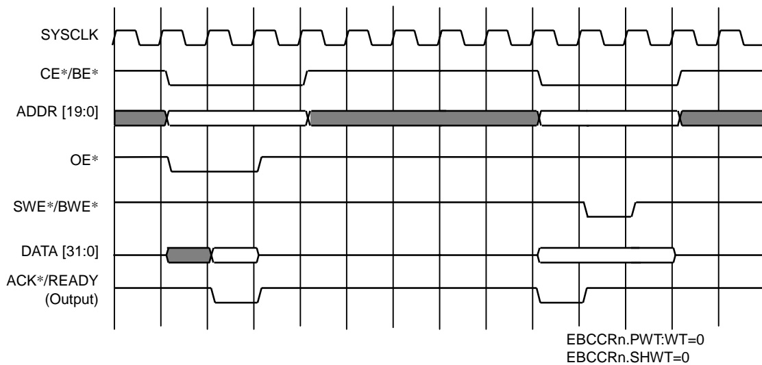
Figure 7.3.5 SWHT Disable (Normal Mode, Single Read/Write Cycle)
