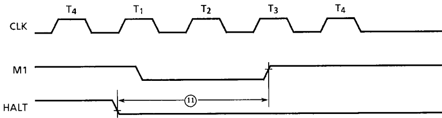
Figure 4.6.6 Clock suspension timing (IDLE1, IDLE2 and STOP modes)
