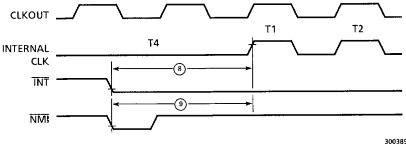
Figure 4.6.4 Clock restart timing (IDLE2 mode)
