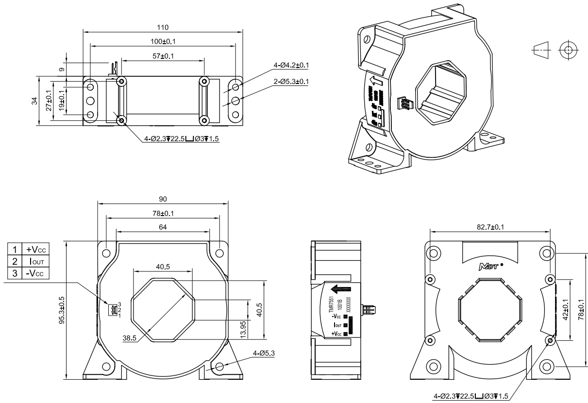
Figure 13. Dimension (unit: mm, tolerances for unmarked scales ±1 mm)
