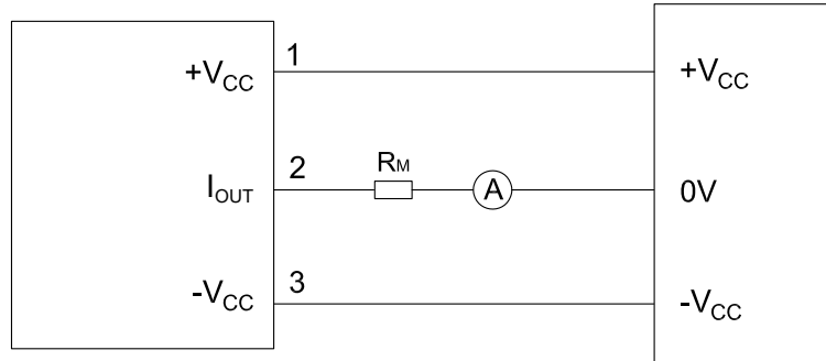
Figure 12. Electrical Connection
