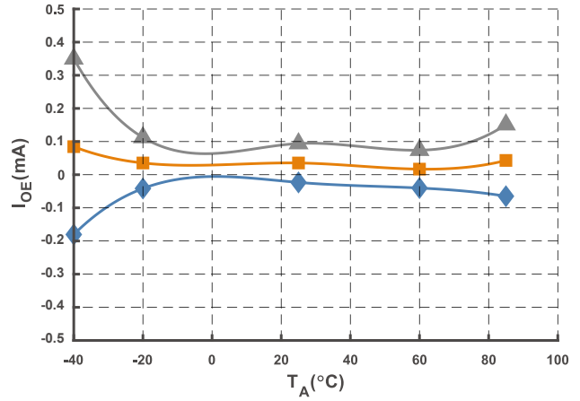
Figure 9. Offset Error
