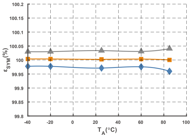
Figure 8. Symmetry
