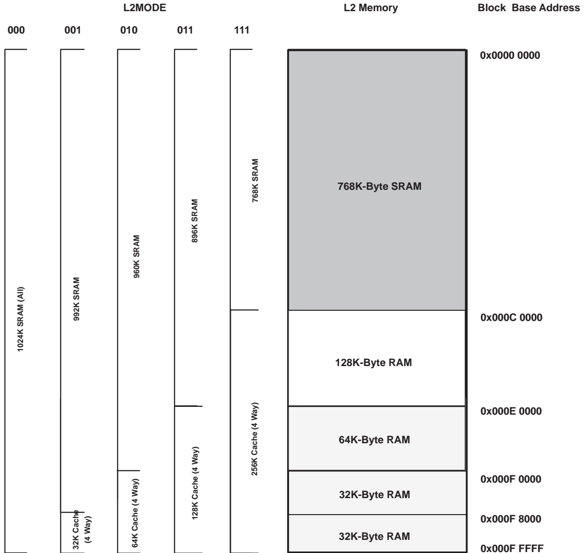
Figure 2. TMS320TC100Q L2 Architecture Memory Configuration
