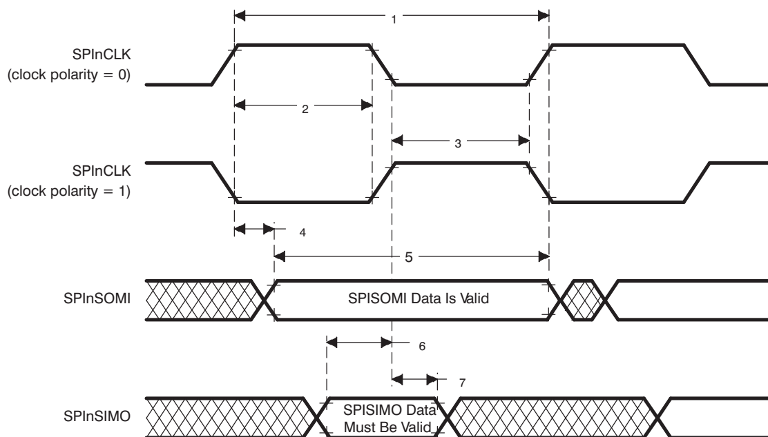
Figure 14. SPI Slave Mode External Timing (CLOCK PHASE = 0)
