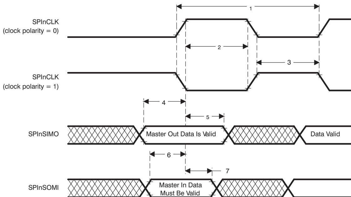
Figure 13. SPIn Master Mode External Timing (CLOCK PHASE = 1)
