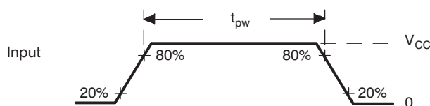
Figure 11. CMOS-Level Inputs
