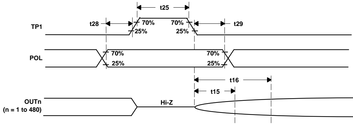
Figure 8. Output Timing
