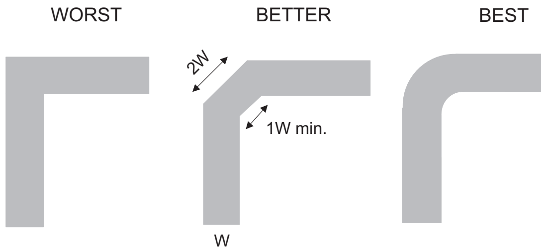
Figure 31. Trace Example
