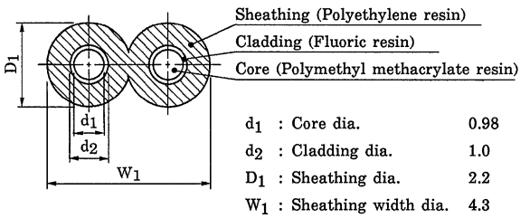
(2) Optical fiber
