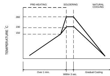
Figure 3. Hand Soldering
