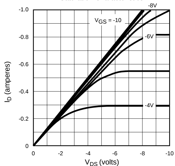
Saturation Characteristics
