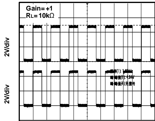
Figure 14. Large-Scale Step Response
