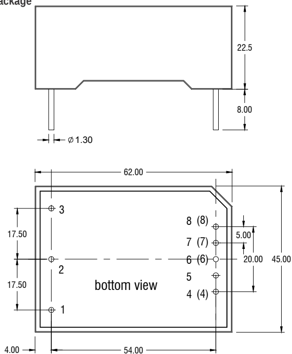
DIP Package
