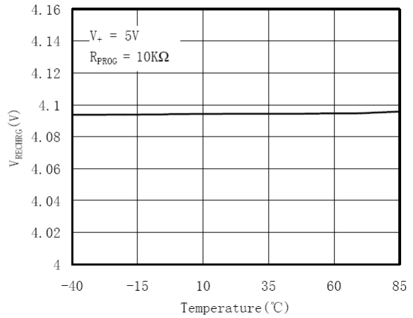
Recharge Voltage Threshold vs. Temperature
