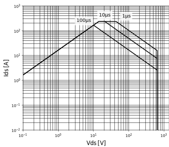
Figure 15. Safe Operating Area T_c = 25^\circ\text{C}
